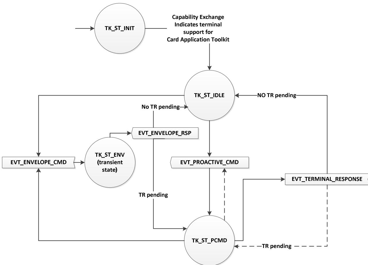
Figure 10.10: State transitions
