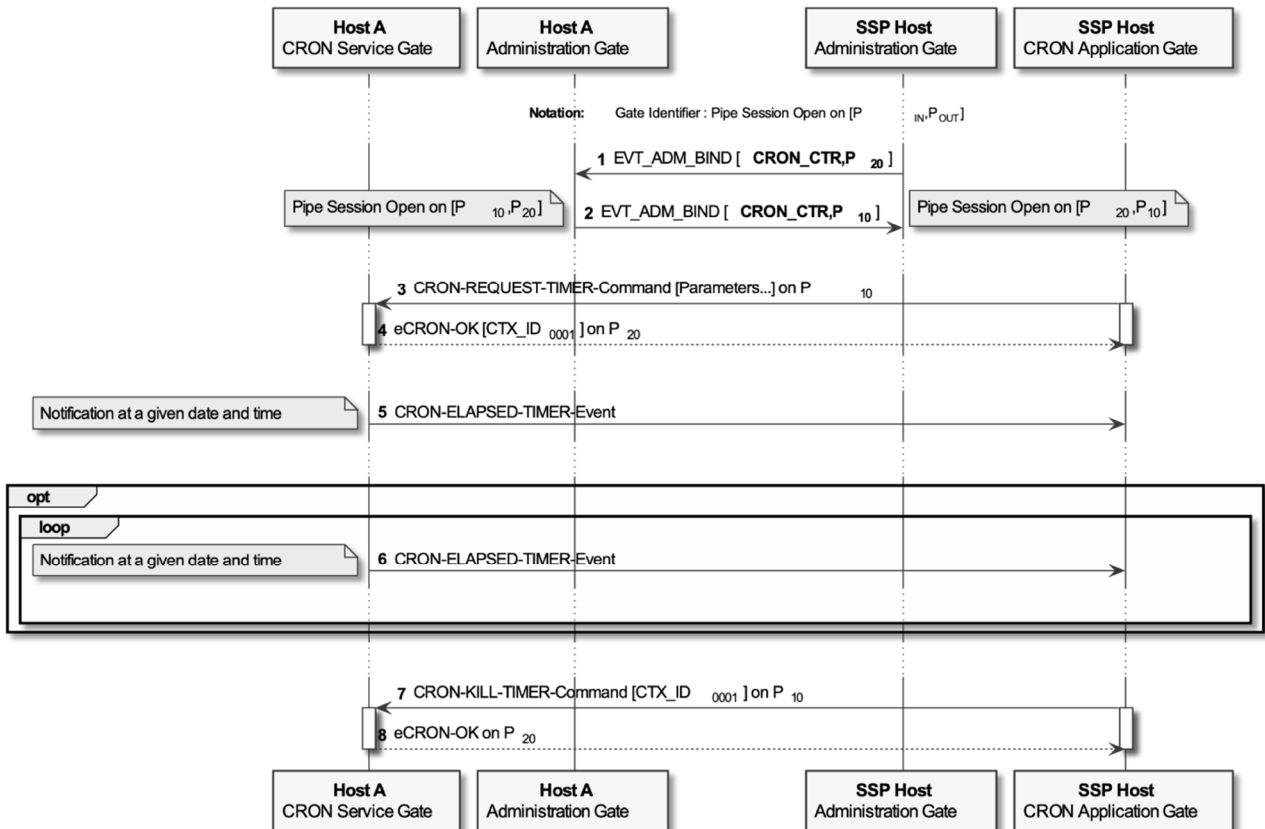
Figure F.1: CRON timer request
