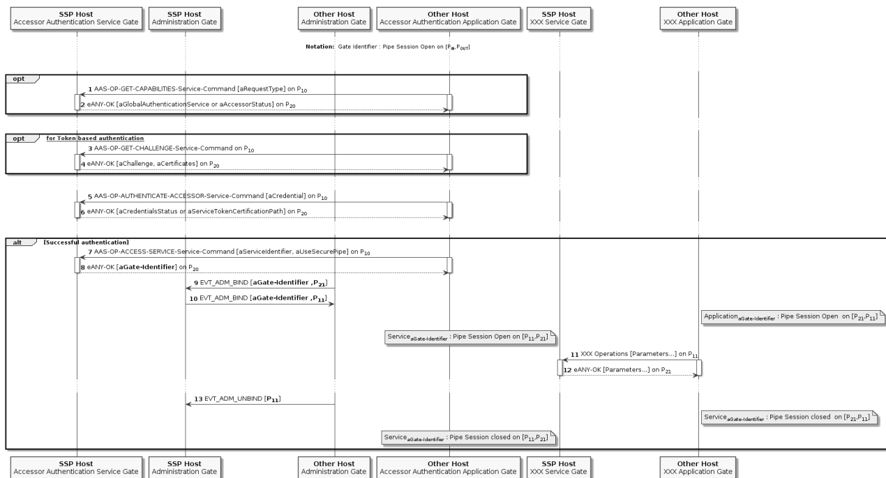
Figure J.4: Accessor authentication session opening
