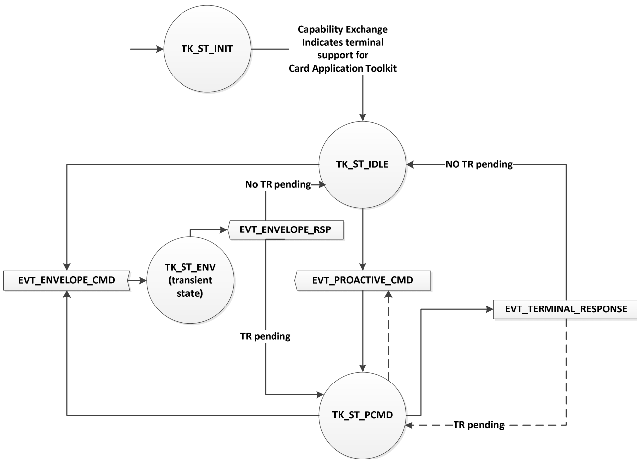
Figure 10.10: State transitions
