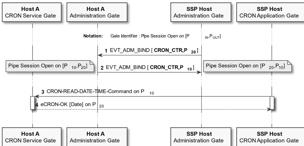
Figure F.3: CRON Read Date
