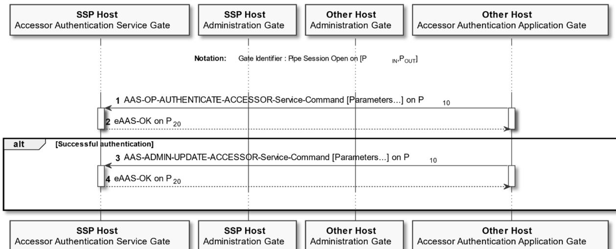
Figure J.3: Accessor credentials update
