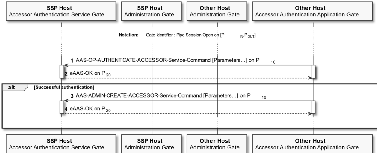
Figure J.1: Accessor creation
