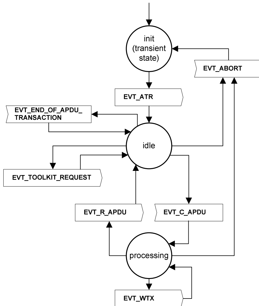
Figure 10.2: State transitions
