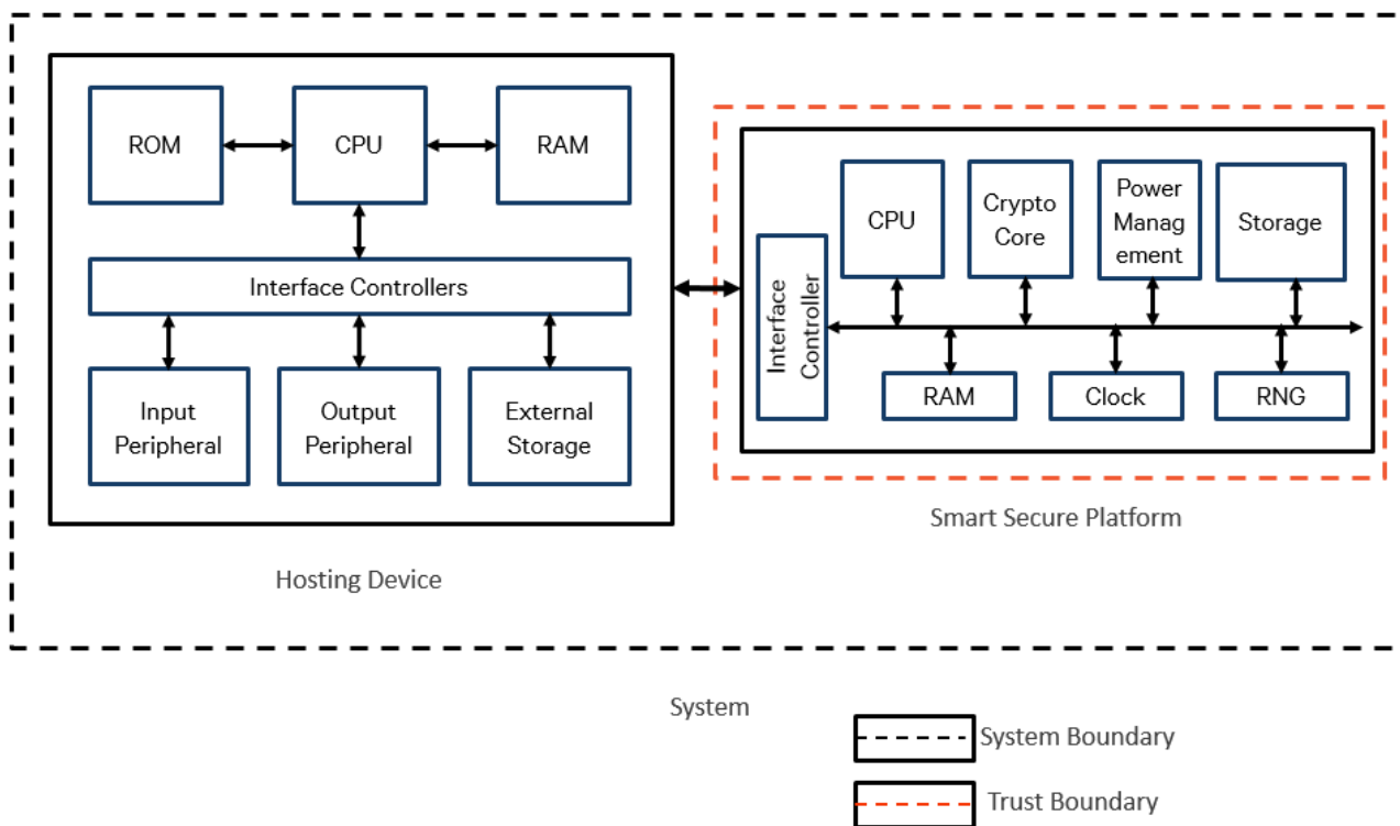
Figure 6.3: SSP Security
