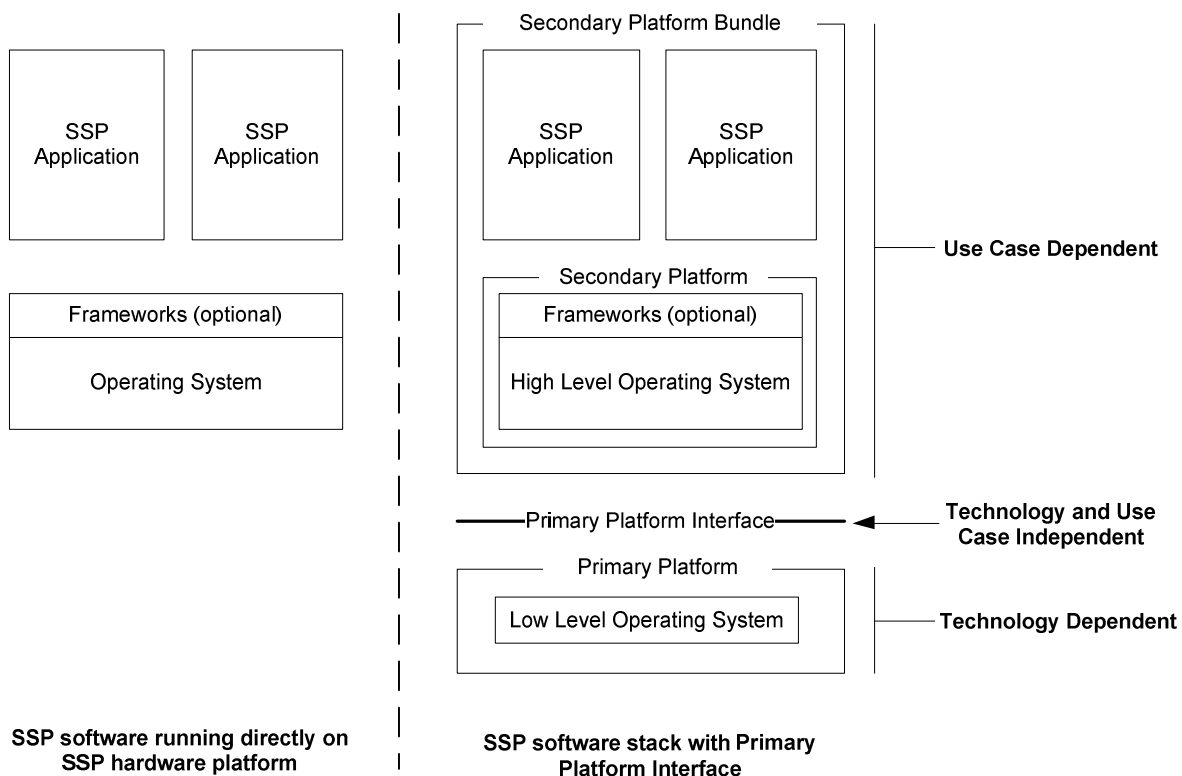
Figure 5.1: SSP software architectures
