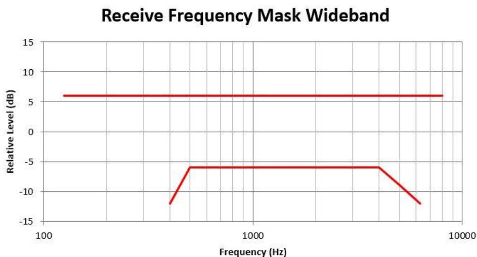
Figure 6.1.2.1-1: Handheld receive sensitivity/frequency response
