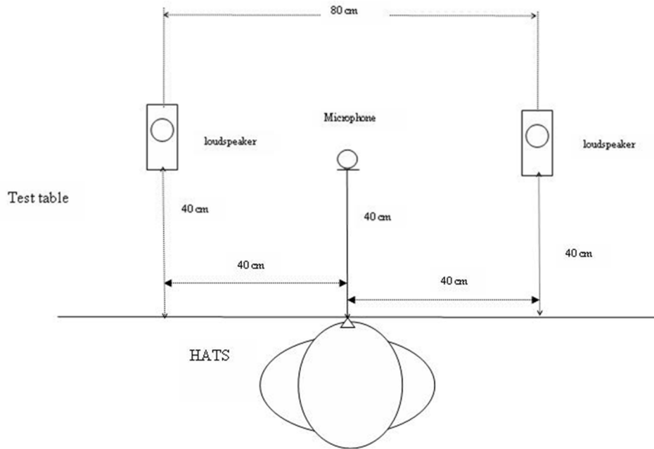
Figure 5.2.4.2-2: Configuration of softphone using external speakers and microphone relative to the HATS-top sight
