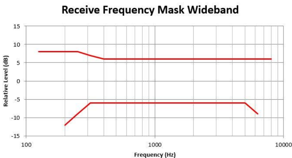
Figure 6.1.2.4-1: Desktop receive sensitivity/frequency response
