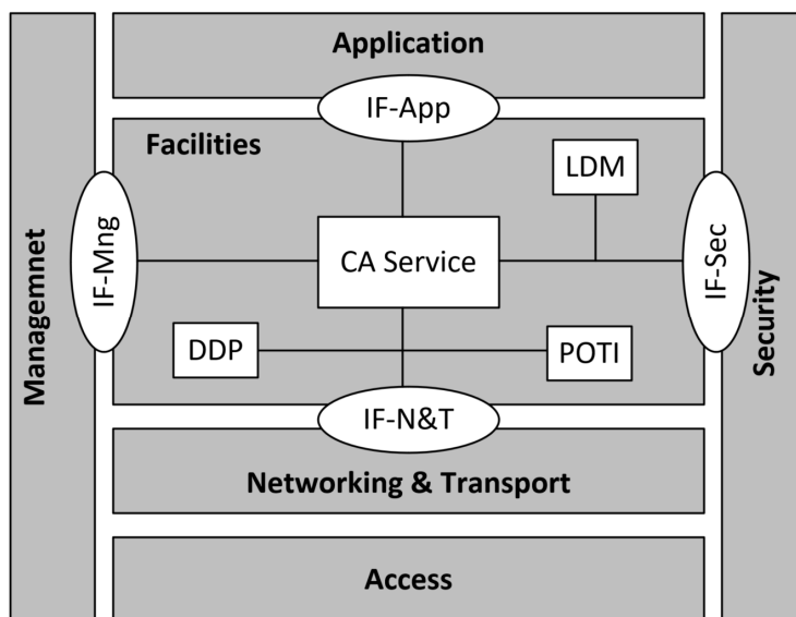
Figure 1: CA service within the ITS-S architecture
