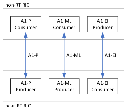
Figure 5.1-1: Service framework for the A1 services
