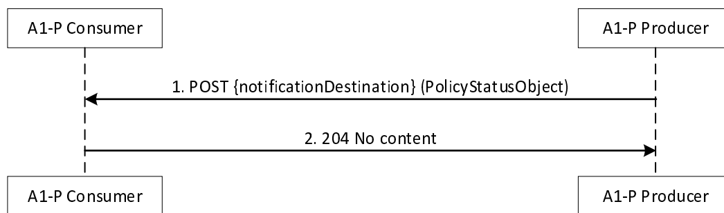
Figure 5.2.4.8.1-1: Feedback policy operation
