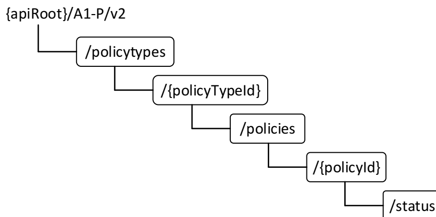
Figure 6.2.3.1.1-1: Resource URI structure of the A1-P API
