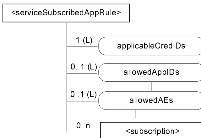
Figure 9.6.29-1: Structure of <serviceSubscribedAppRule> resource
