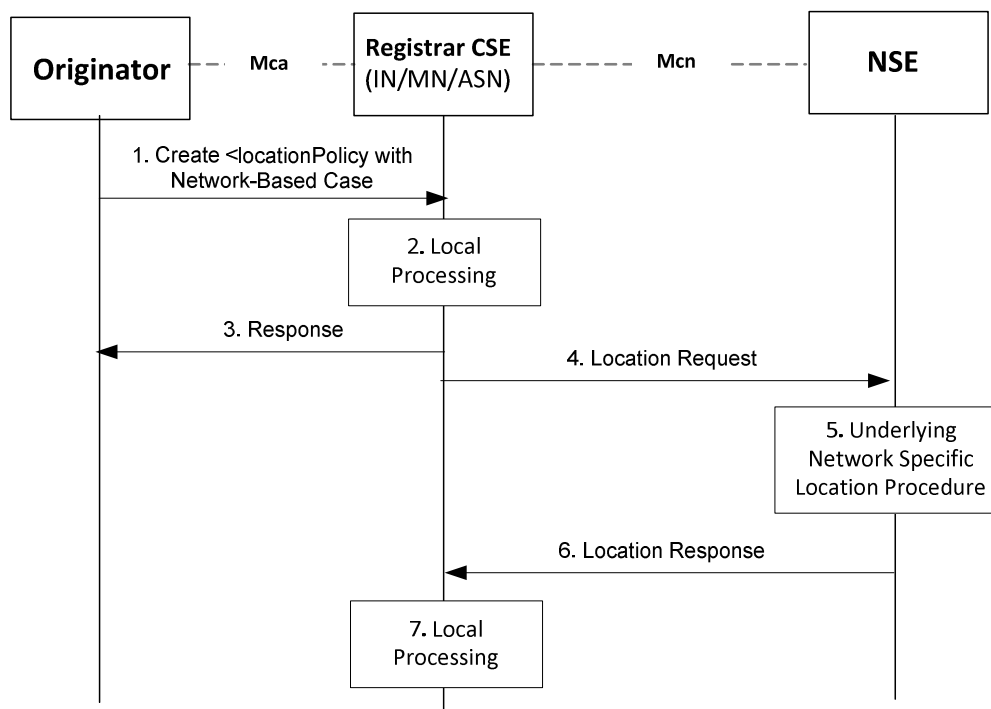
Figure 8.5.2-1: General Procedure for Location Request
