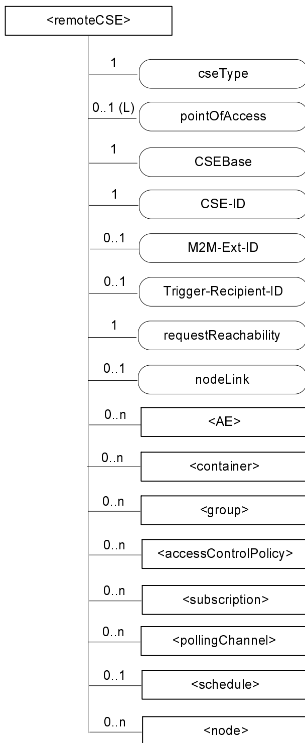
Figure 9.6.4-1: Structure of <remoteCSE> resource
