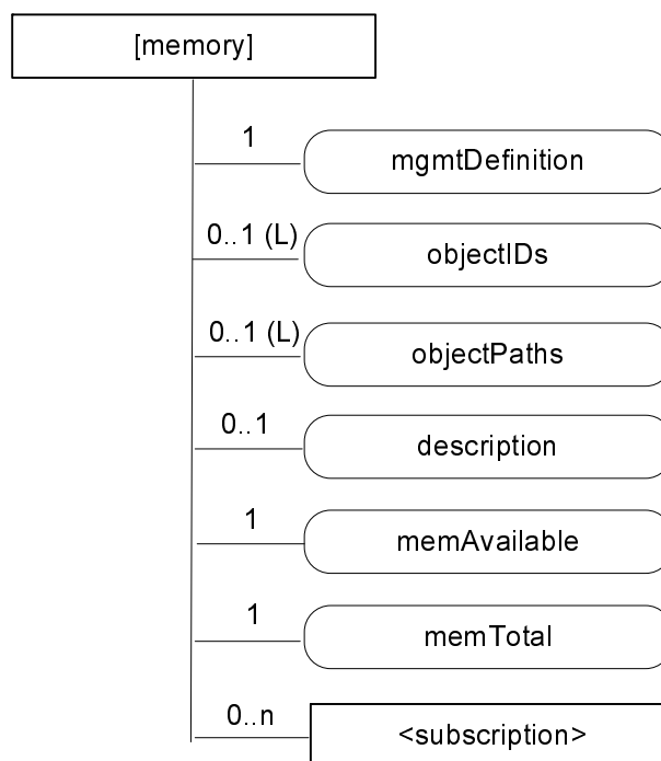
Figure D.4-1: Structure of [memory] resource
