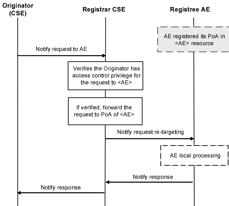
Figure 9.3.2.3-1: Re-targeting a notification request to an AE
