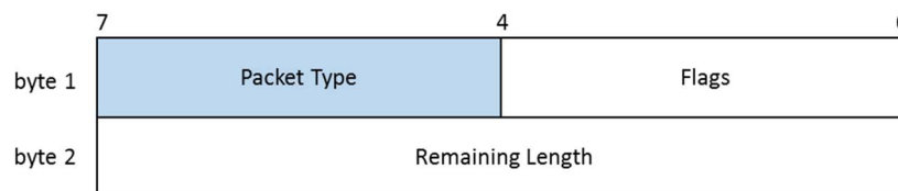
Figure 6.4.1-2: Fixed header structure
