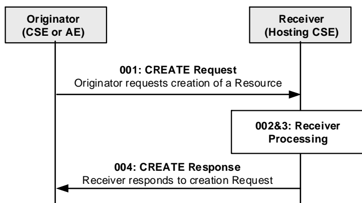
Figure 6.4.2.4-1: Procedure for Creating a Resource (oneM2M TS-0001 [2], clause 10)
