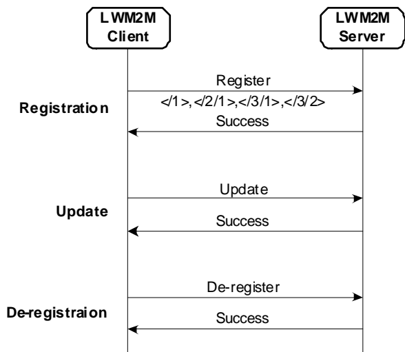
Figure A.5.3.2-1: Example of Registration Procedure
