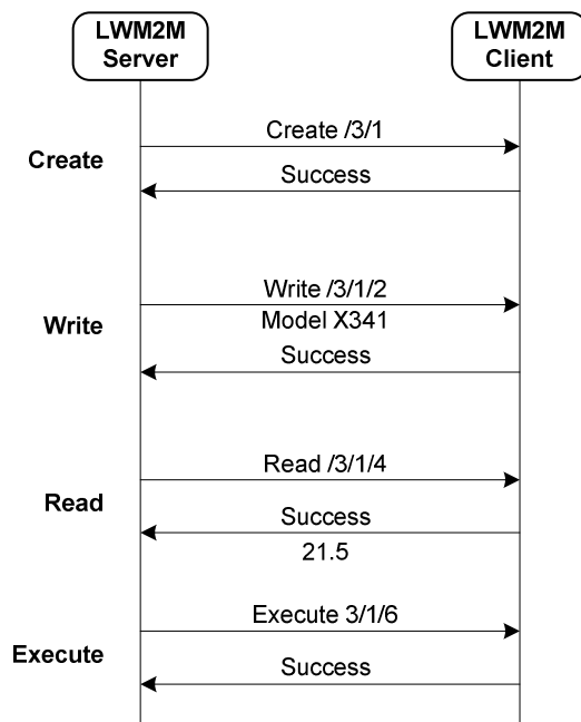
Figure A.5.3.3-1: Example of Device Management and Service Enablement Interface
