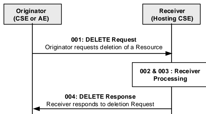
Figure 6.4.2.5-1: Procedure for Deleting a resource (oneM2M TS-0001 [2], clause 10)
