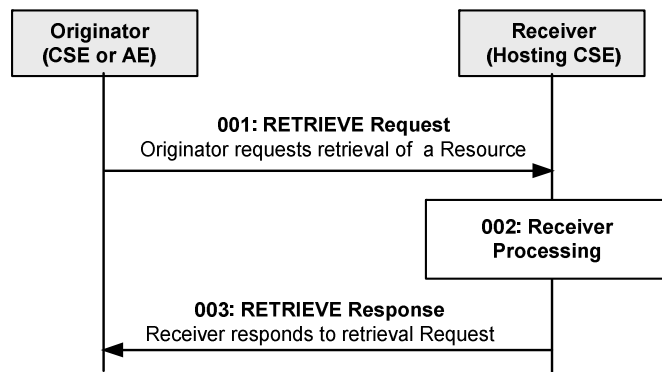
Figure 6.4.2.3-1: Procedure for Retrieving a Resource (oneM2M TS-0001 [2], clause 10)
