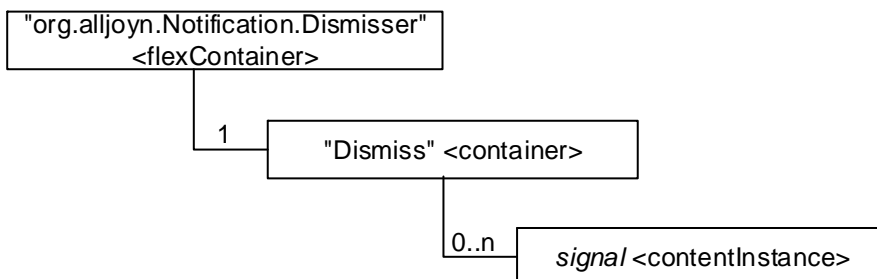
Figure C.1.3-1: Structure of Dismisser interface mapping
