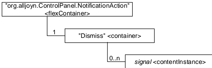
Figure C.2.5-1: Structure of NotificationAction interface mapping
