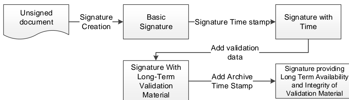
Figure 4: Signature Lifecycle
