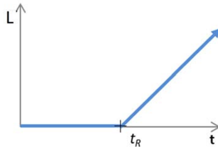
Figure C.4.6-1: Lateness function
