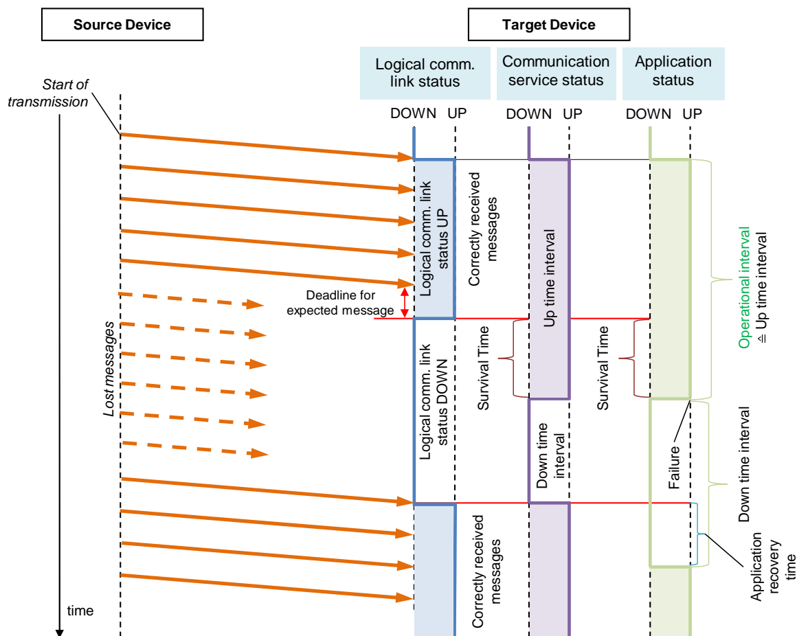
Figure C.3-1: Relation between logical communication link, communication service and application statuses (example with lost messages)
