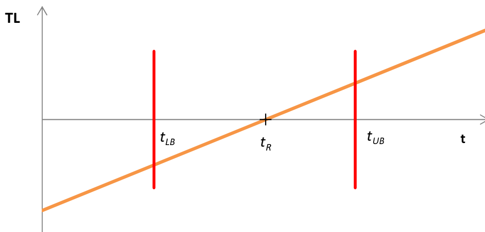
Figure C.4.3-1: Timeliness function
