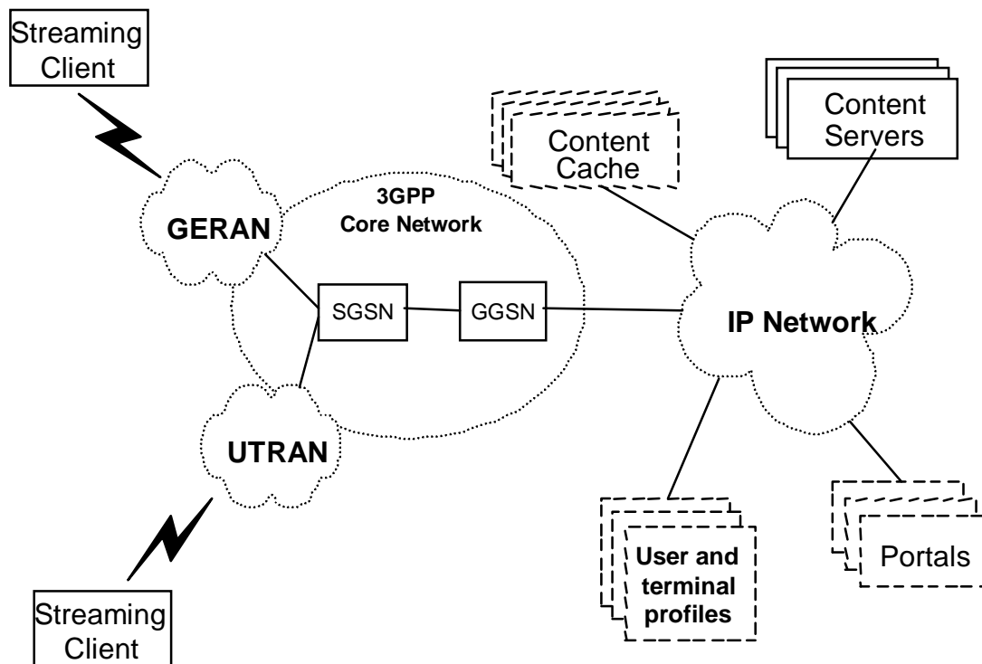
Figure 01: Network elements involved in a 3G packet switched streaming service
