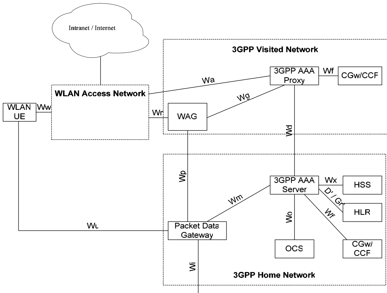
Figure 8: Configuration of a 3GPP/WLAN interworking function
