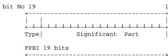
Figure 14: General structure of FPBI
