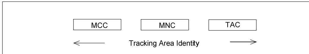
Figure 28.6-1: Structure of the 5GS Tracking Area Identity (TAI)
