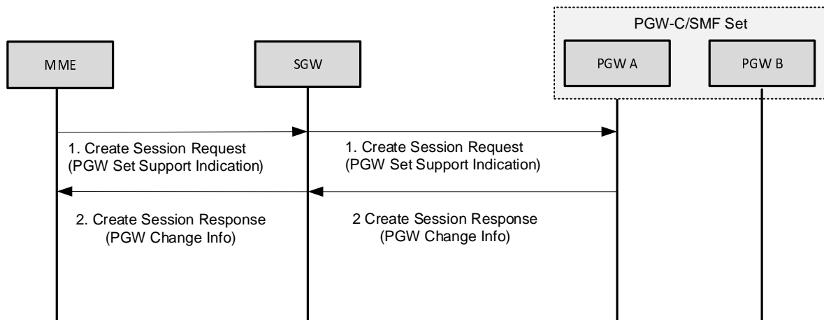
Figure 31.2-1: PDN connection establishment
