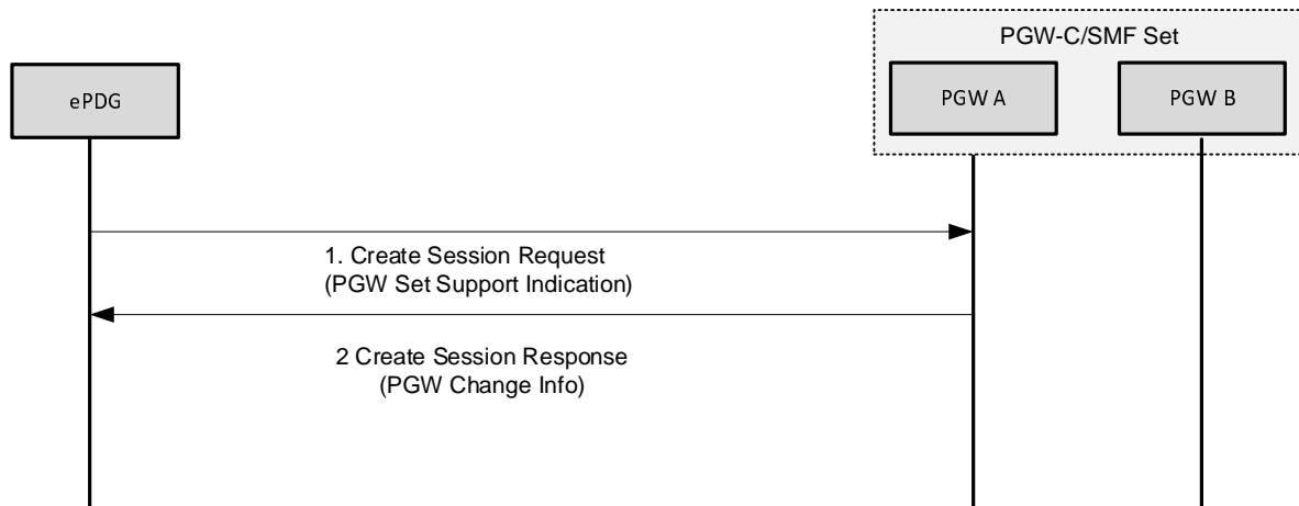
Figure 31.2A-1: PDN connection establishment
