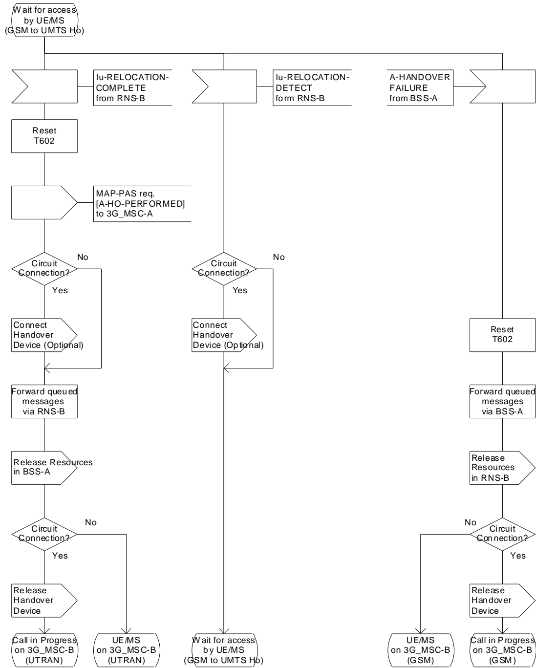
Figure 44 (sheet 9 of 54): Handover control procedure in 3G_MSC-B
