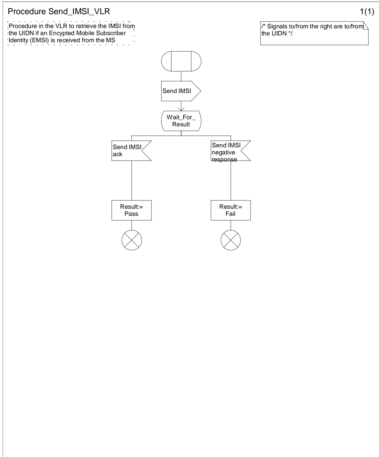
Figure 4.1.2.9: Procedure Send_IMSI_VLR
