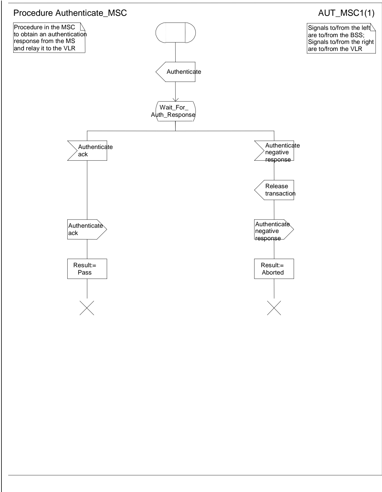
Figure 4.1.1.2 (sheet 1 of 1): Procedure Authenticate_MSC
