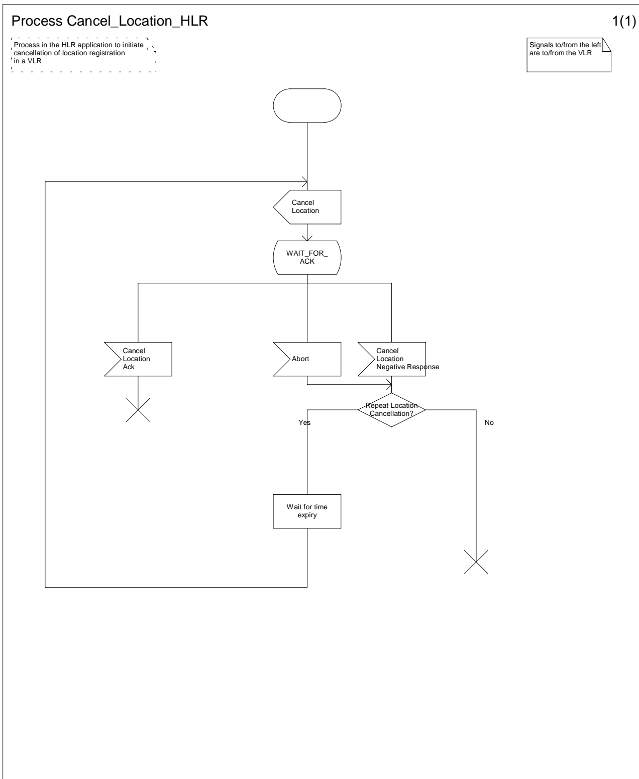
Figure 4.2.2.1: Process Cancel_Location_HLR
