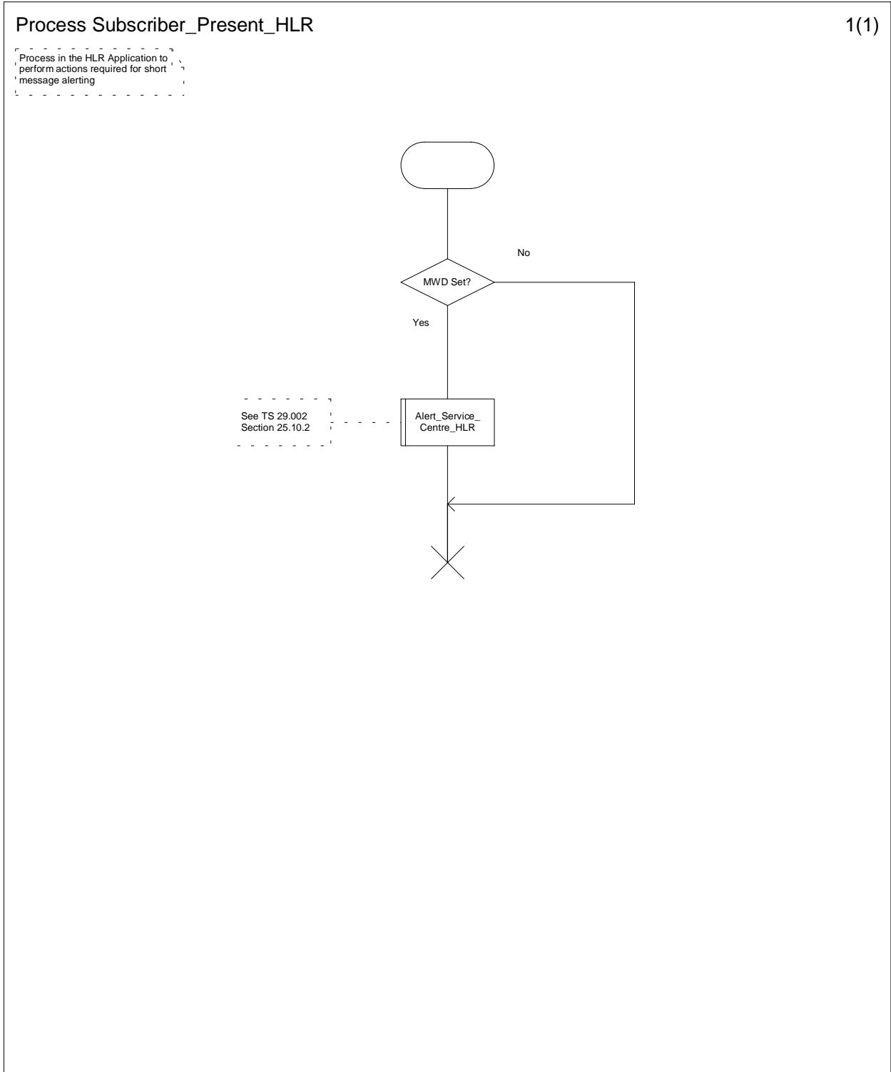
Figure 4.1.3.3: Process Subscriber_Present_HLR
