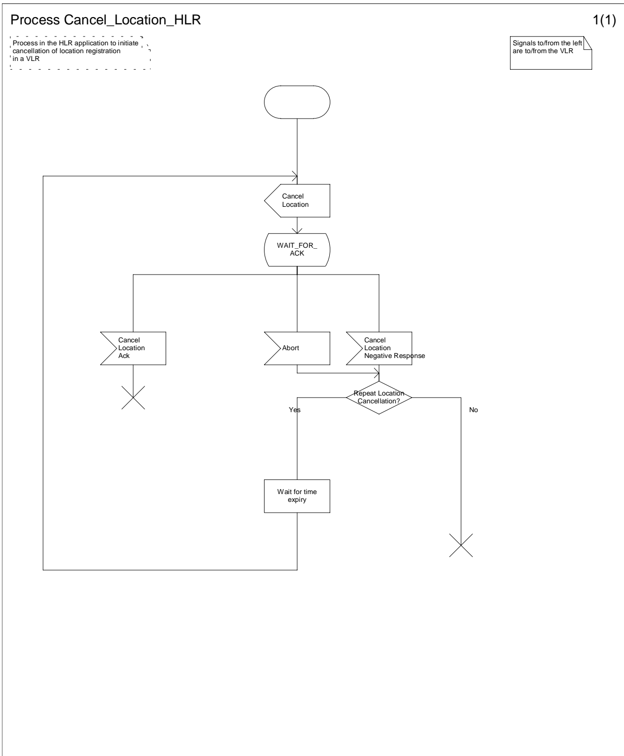
Figure 4.2.2.1: Process Cancel_Location_HLR
