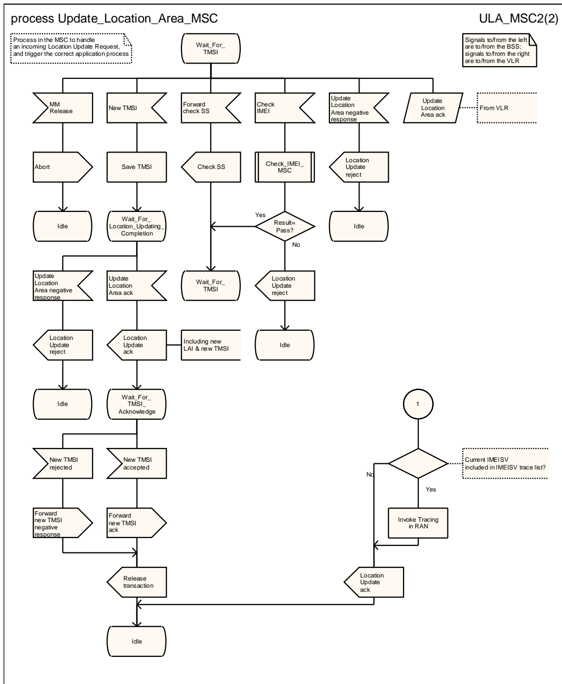
Figure 4.1.1.1 (sheet 2 of 2): Process Update_Location_Area_MSC
