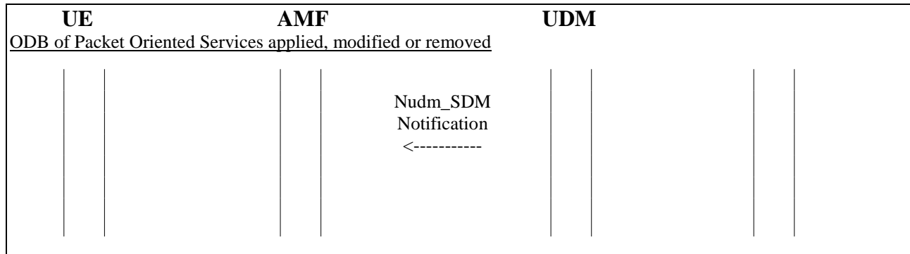
Figure 2.6C.1/1: Transfer of updated subscription information to AMF
