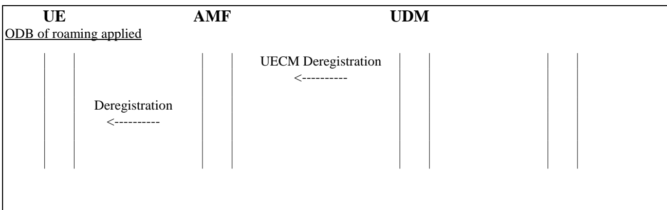
Figure 2.3.1/2: Immediate Application of Barring of Roaming in UDM
