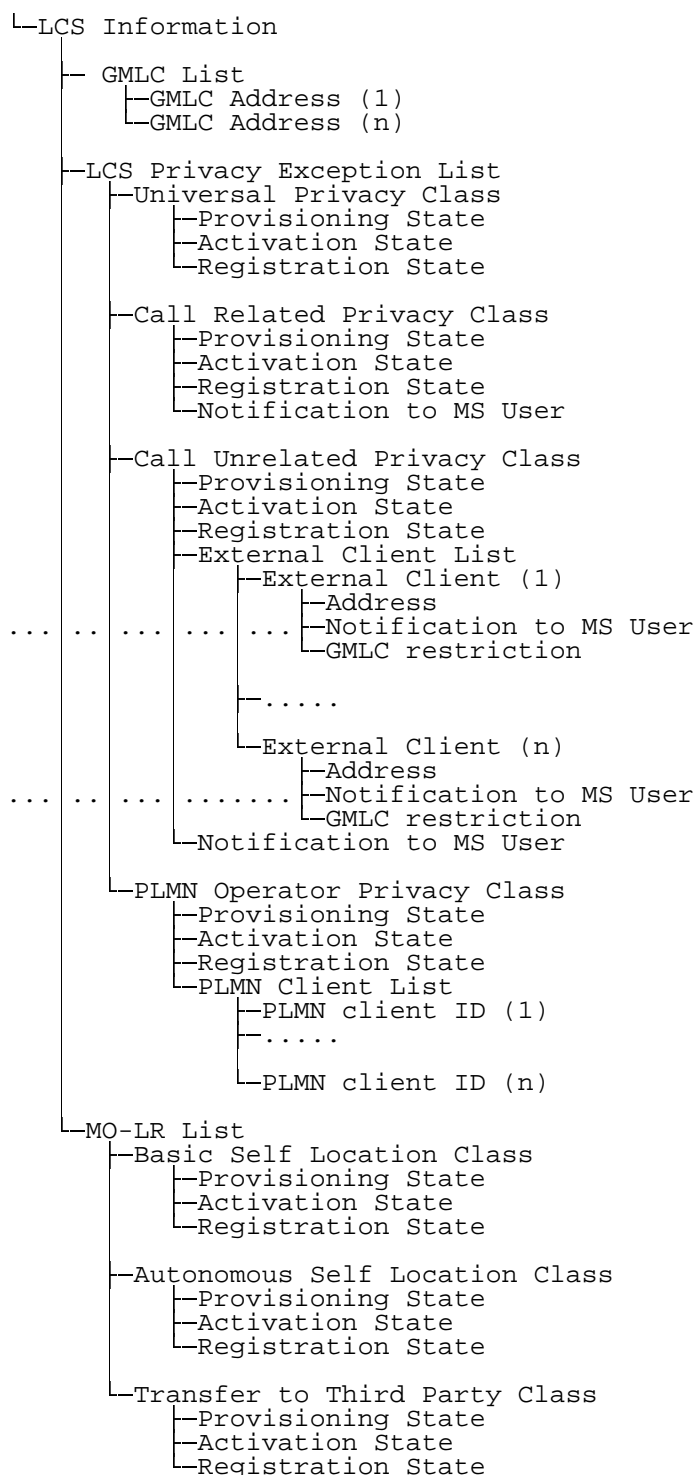
Figure 16: LCS Information
