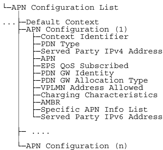
Figure 17a: EPS subscription data
