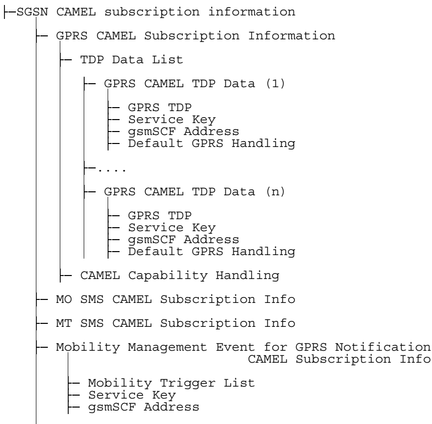
Figure 22: SGSN CAMEL subscription info
