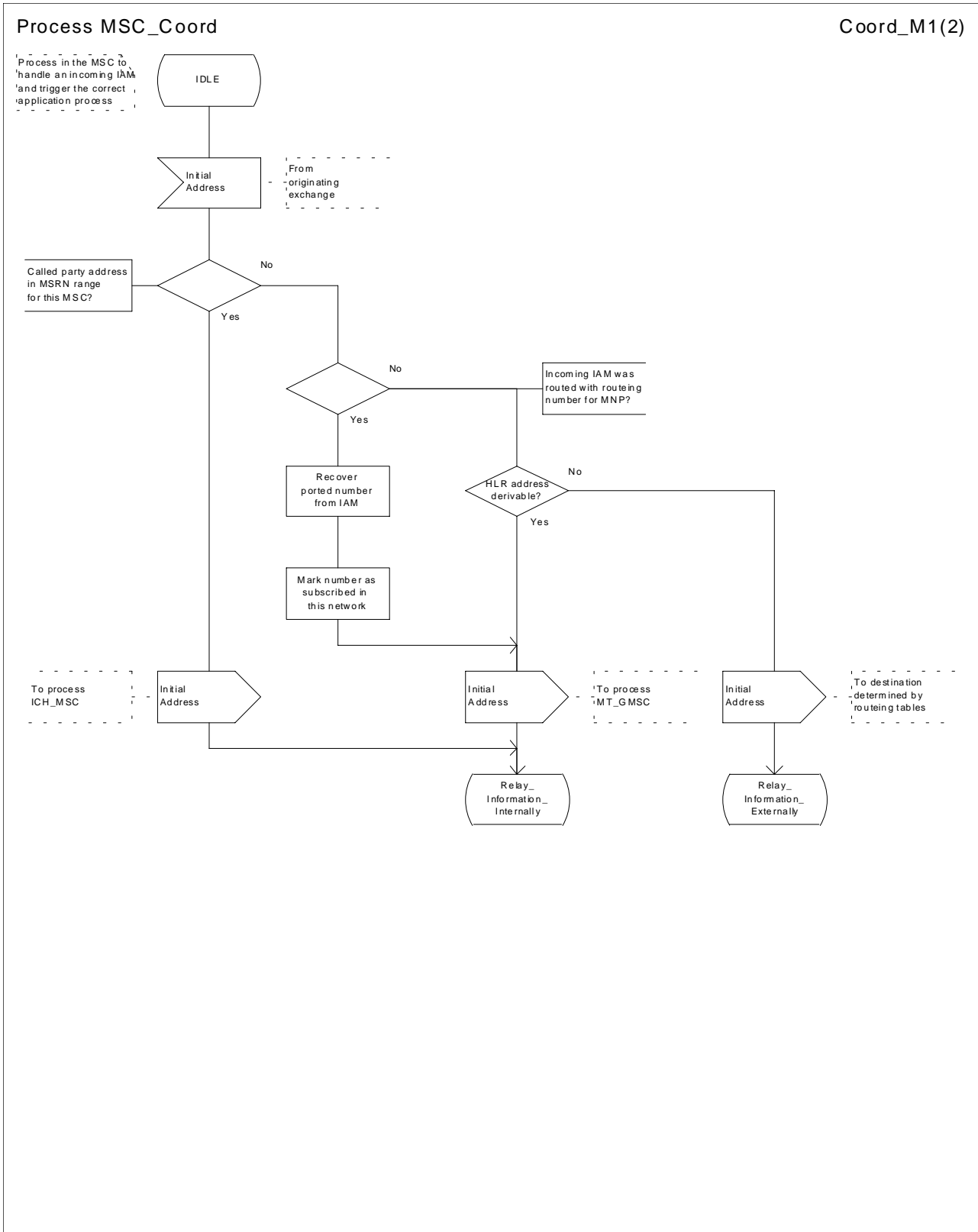
Figure 79a: Process MSC_Coord (sheet 1)
