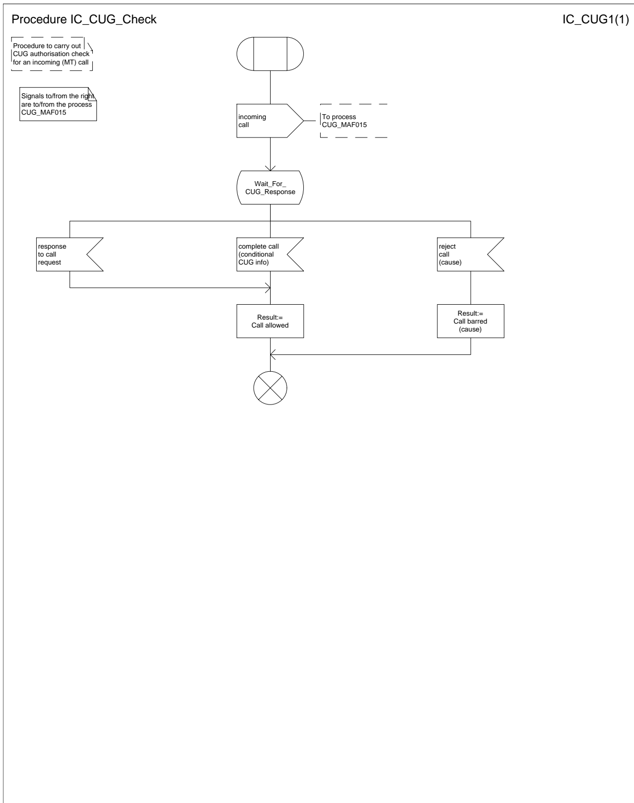
Figure 51: Procedure IC_CUG_Check
