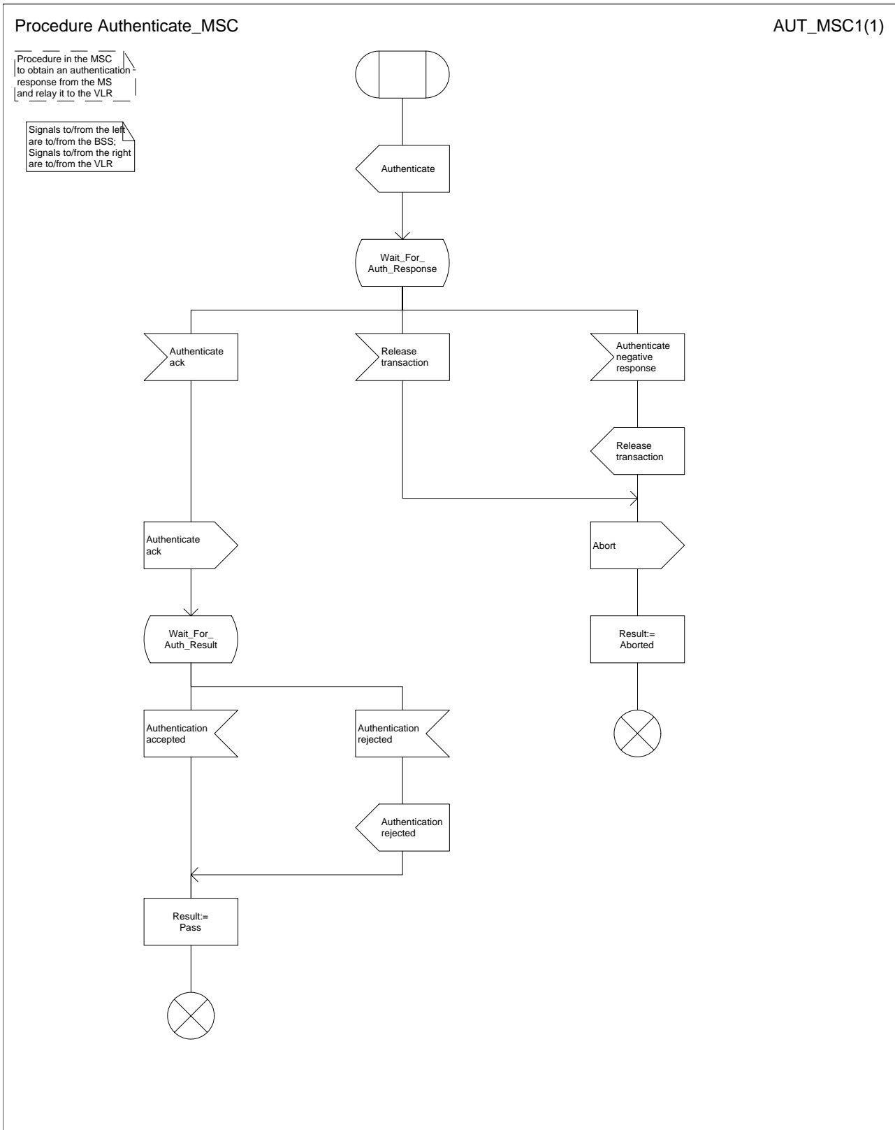
Figure 10: Procedure Authenticate_MSC
