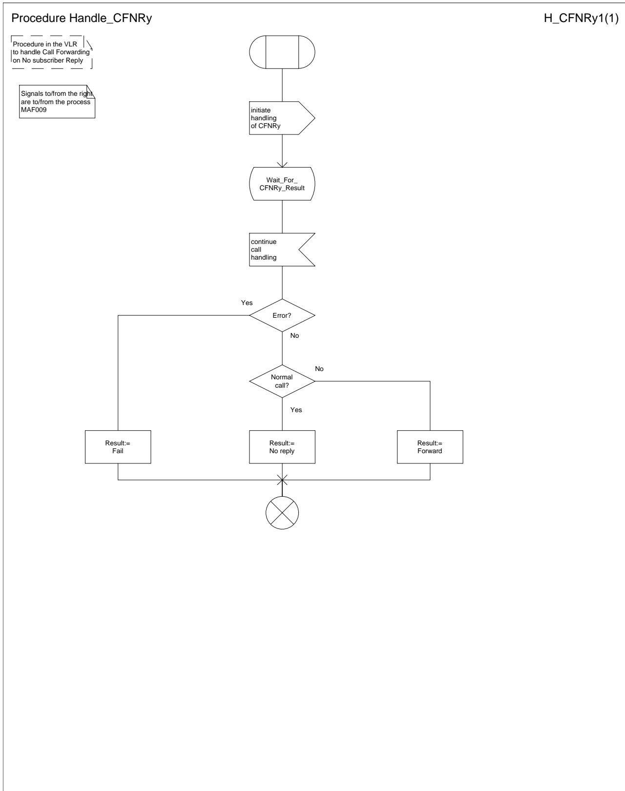
Figure 78: Procedure Handle_CFNRy
