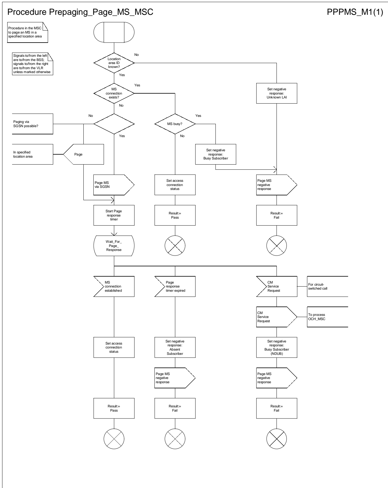
Figure 59: Procedure Prepaging_Page_MS_MSC
