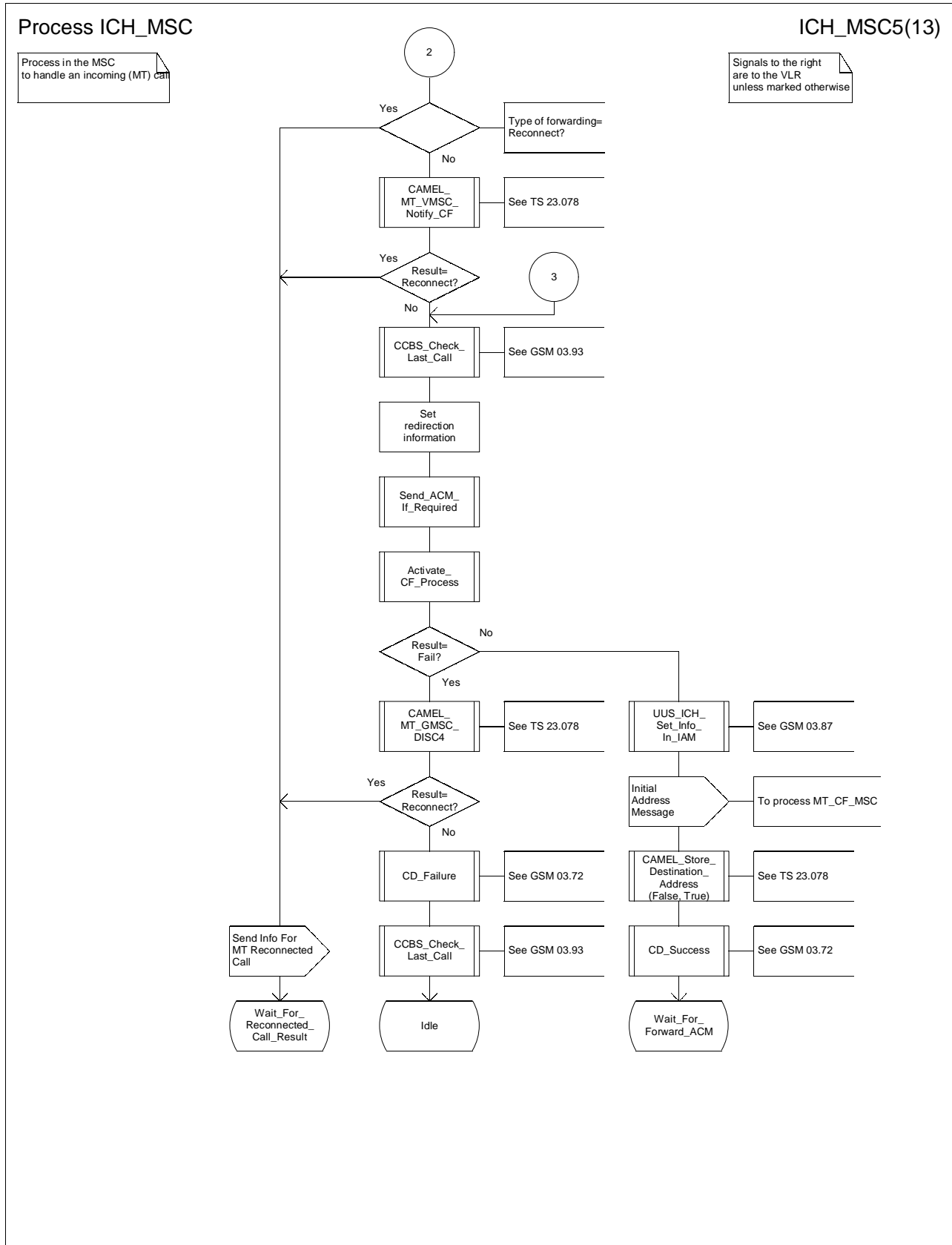
Figure 62e: Process ICH_MSC (sheet 5)
