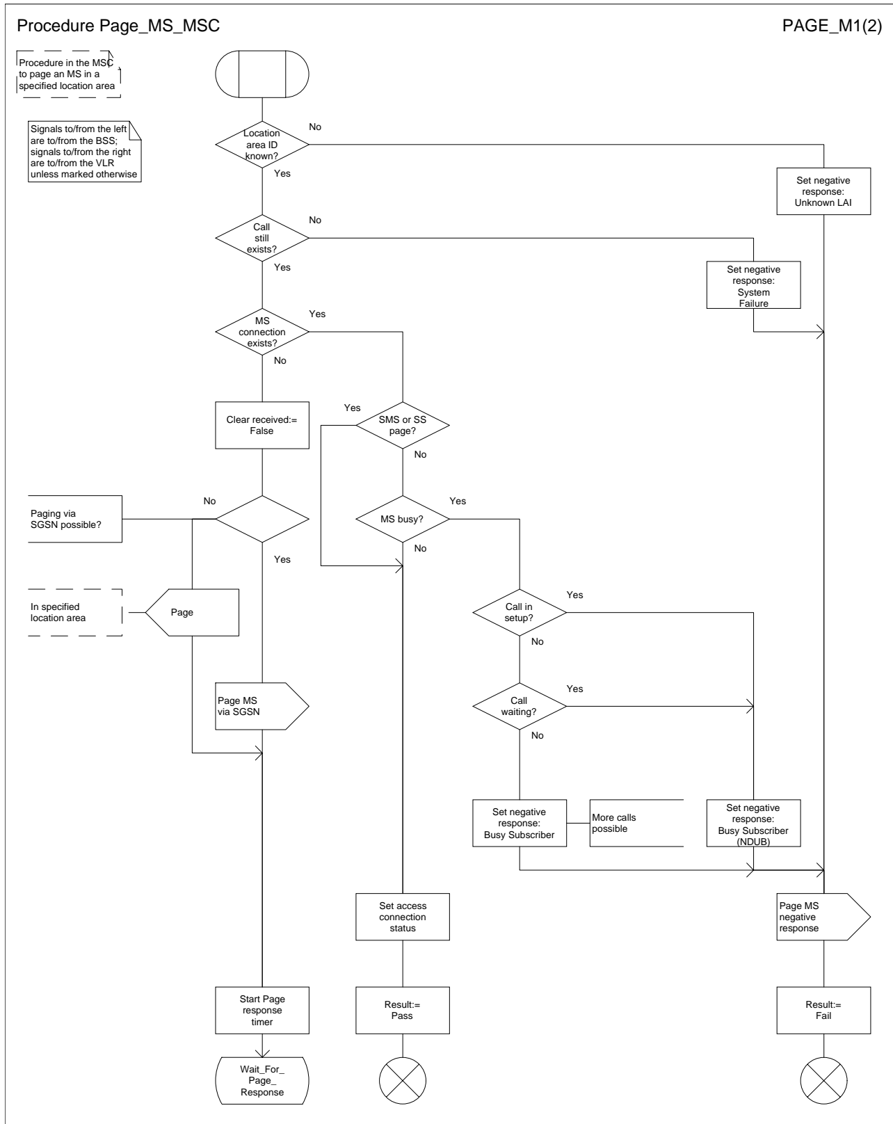
Figure 63a: Procedure Page_MS_MSC (sheet 1)
