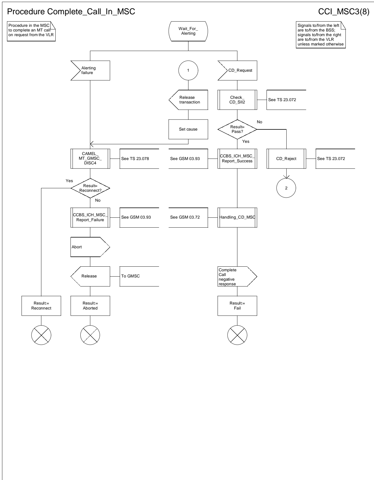
Figure 65c: Procedure Complete_Call_In_MSC (sheet 3)
