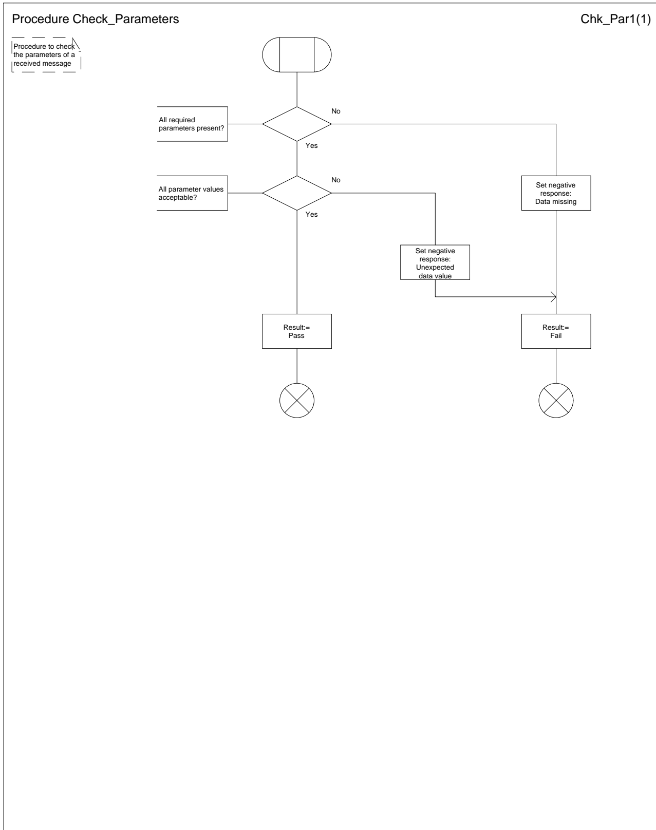
Figure 44: Procedure Check_Parameters
