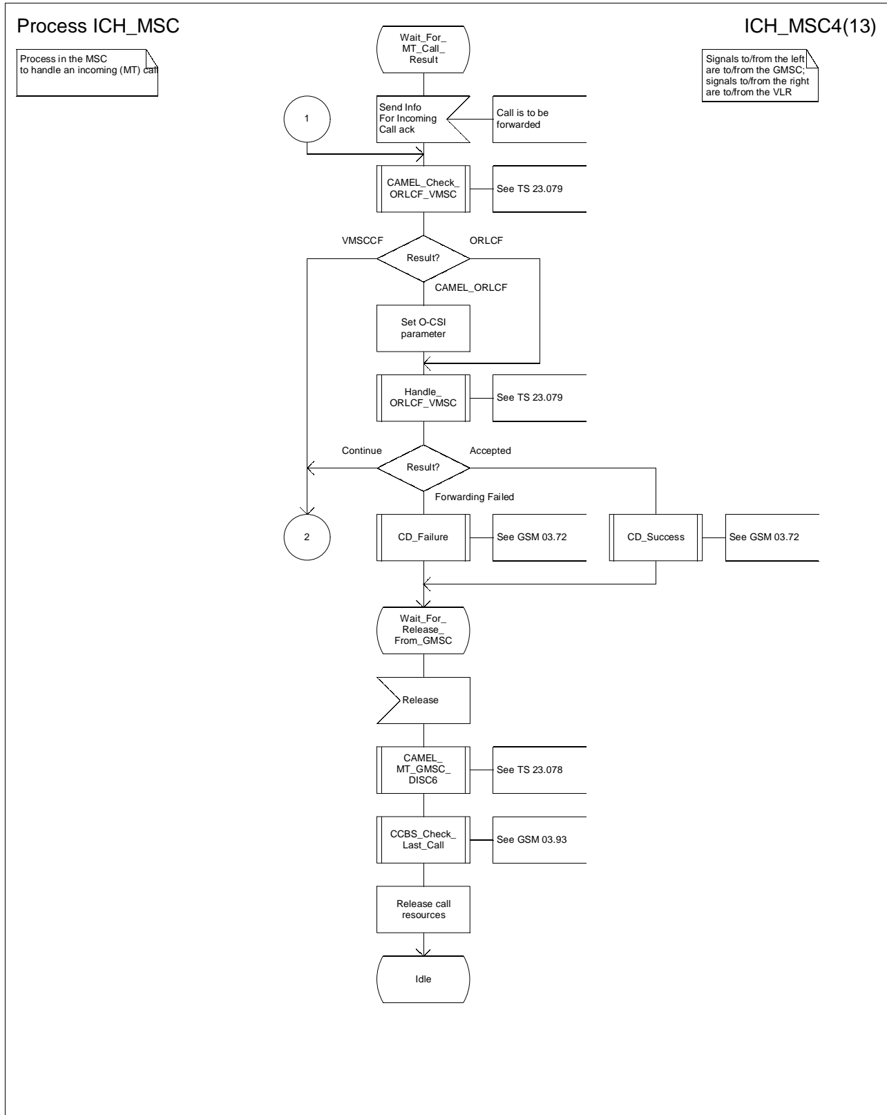
Figure 62d: Process ICH_MSC (sheet 4)
