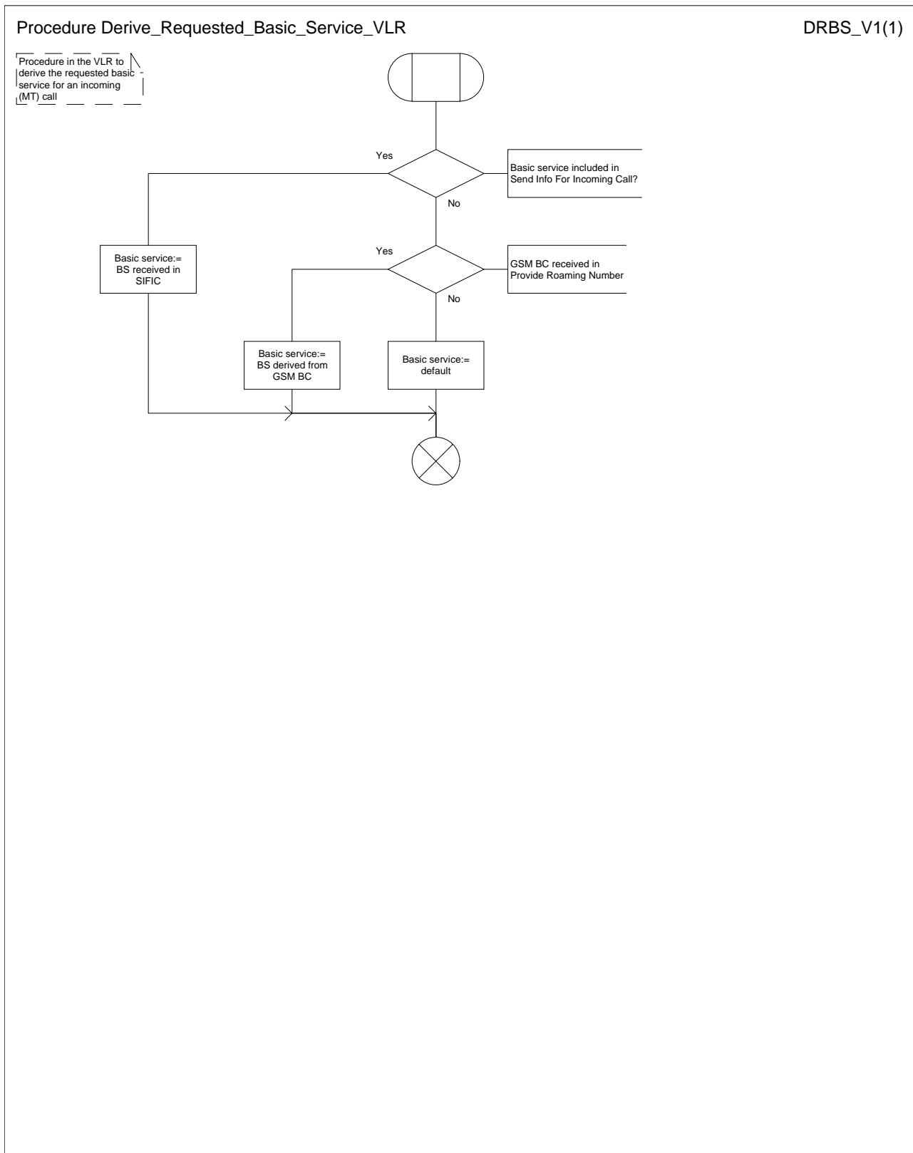
Figure 73: Procedure Derive_Requested_Basic_Service_VLR
