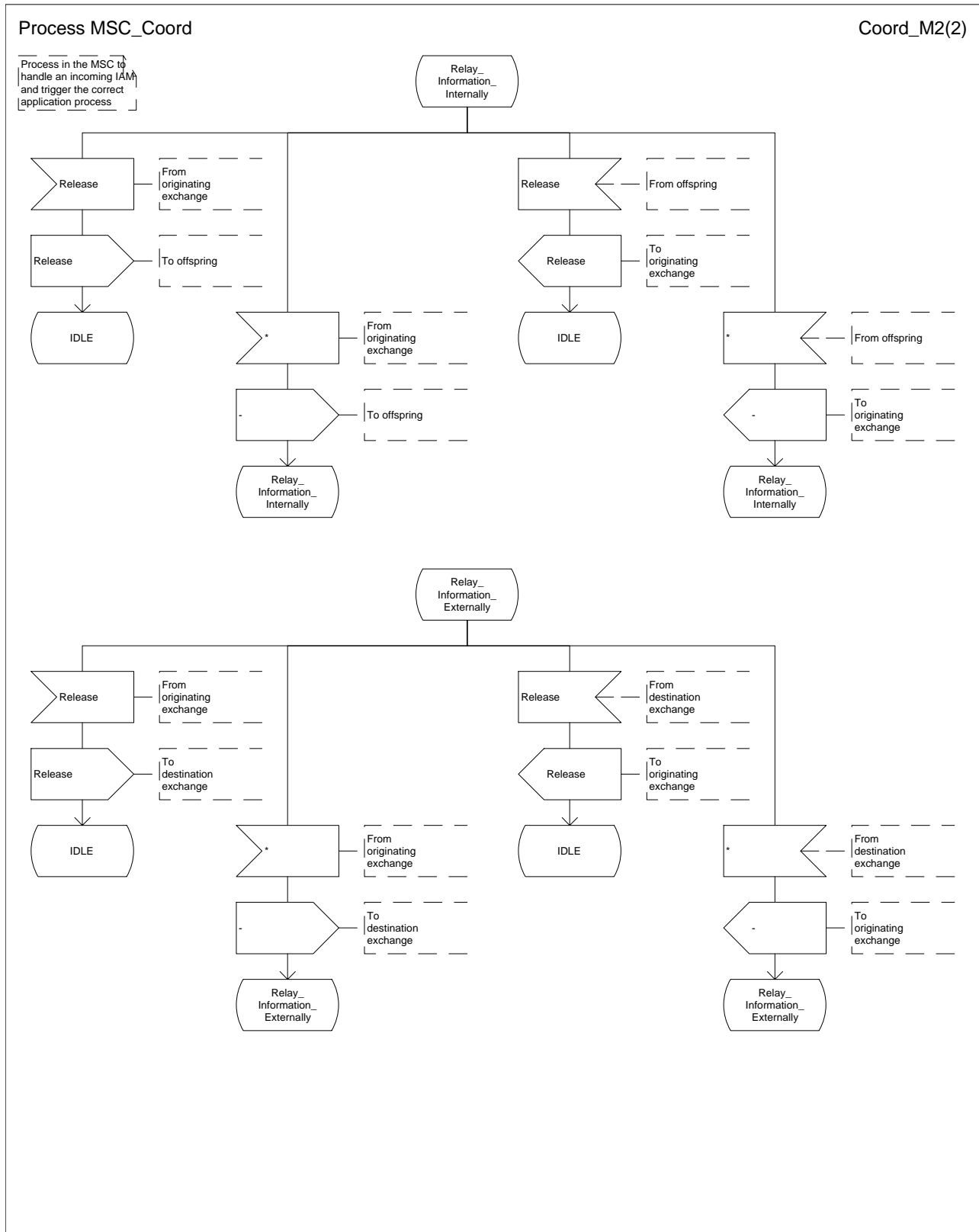
Figure 79b: Process MSC_Coord (sheet 2)
