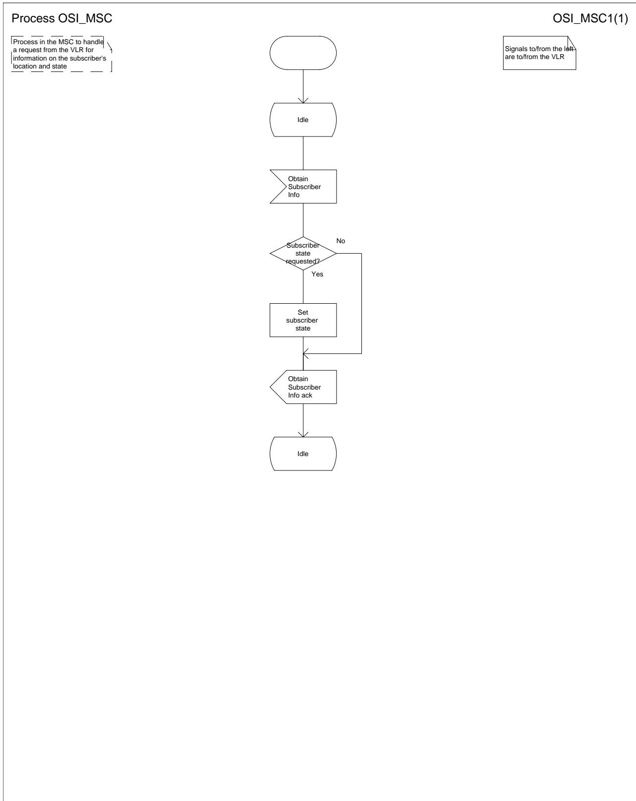
Figure 61: Process OSI_MSC
