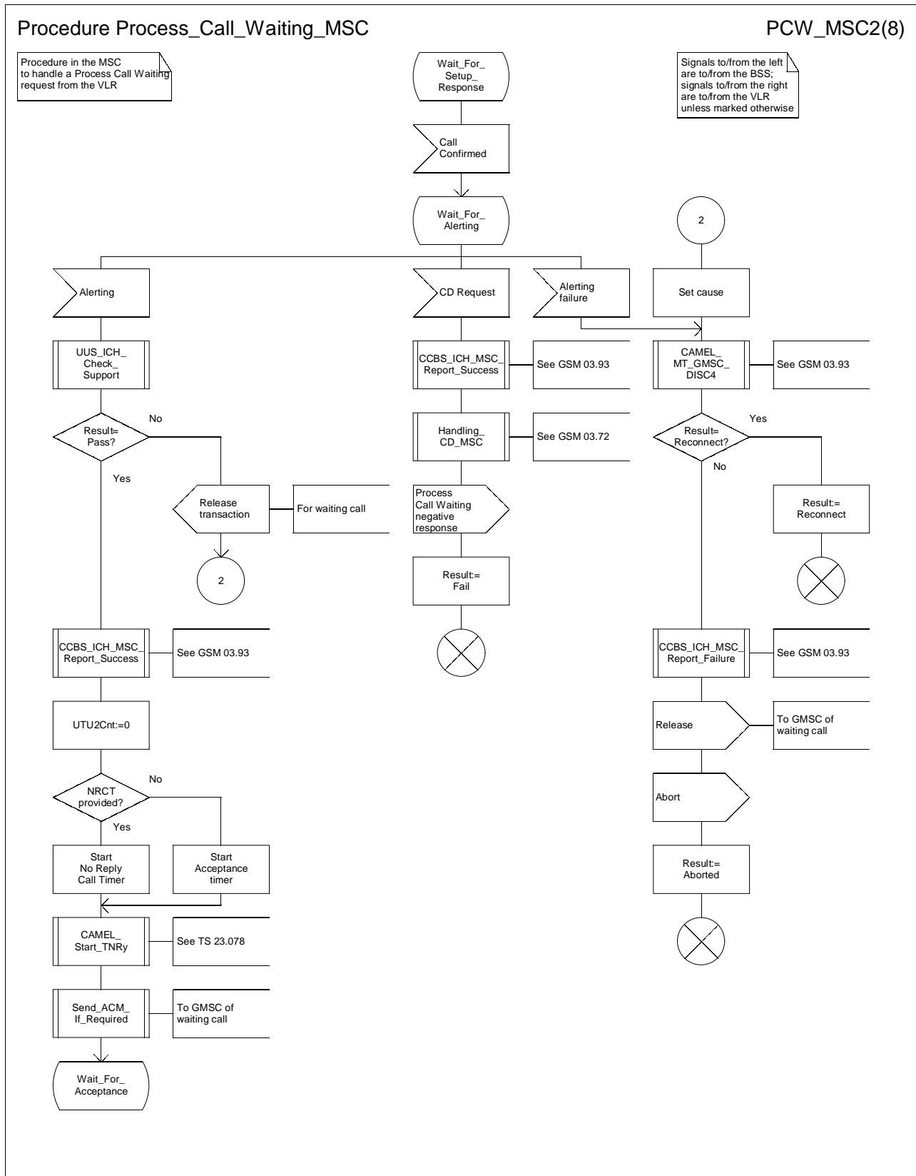
Figure 66b: Procedure Process_Call_Waiting_MSC (sheet 2)
