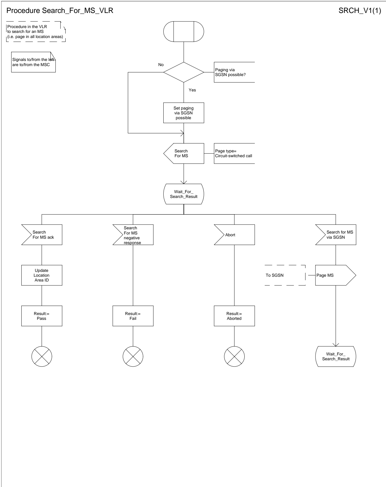
Figure 74: Procedure Search_For_MS_VLR
