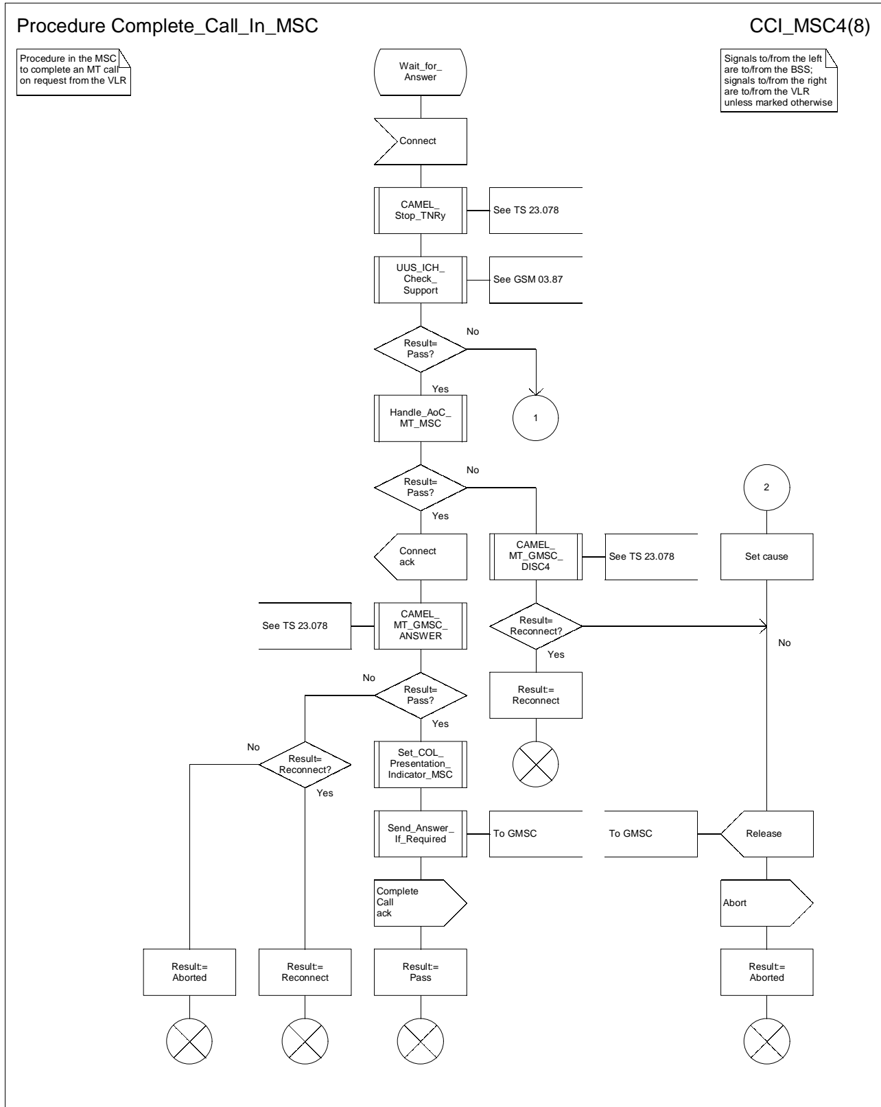
Figure 65d: Procedure Complete_Call_In_MSC (sheet 4)
