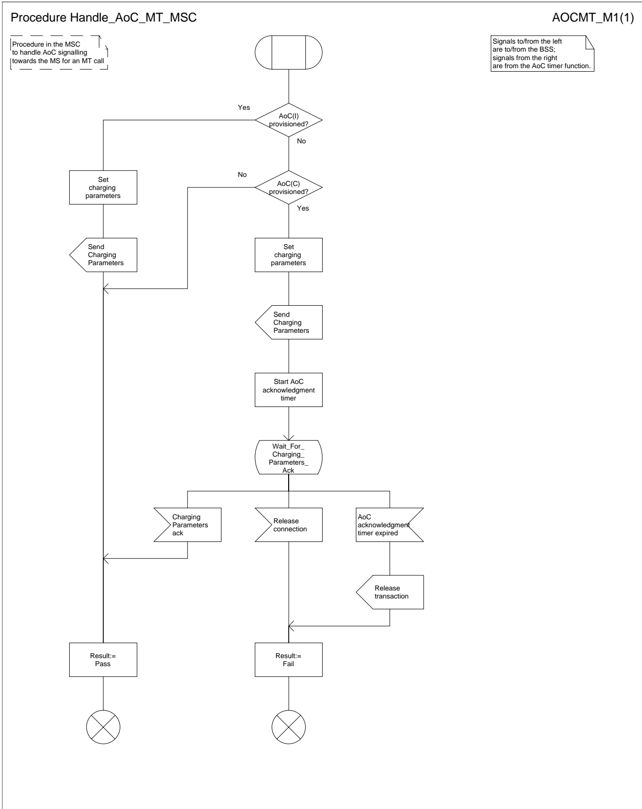
Figure 70: Procedure Handle_AoC_MT_MSC
