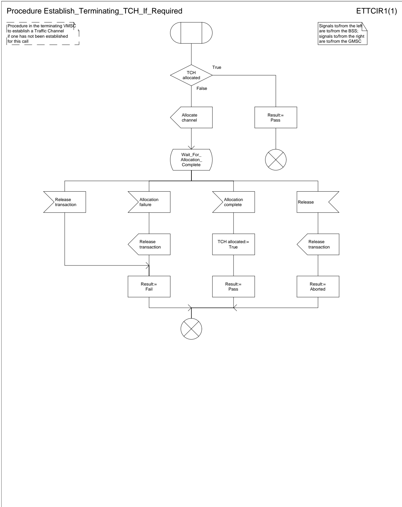
Figure 69: Procedure Establish_Terminating_TCH_If_Required
