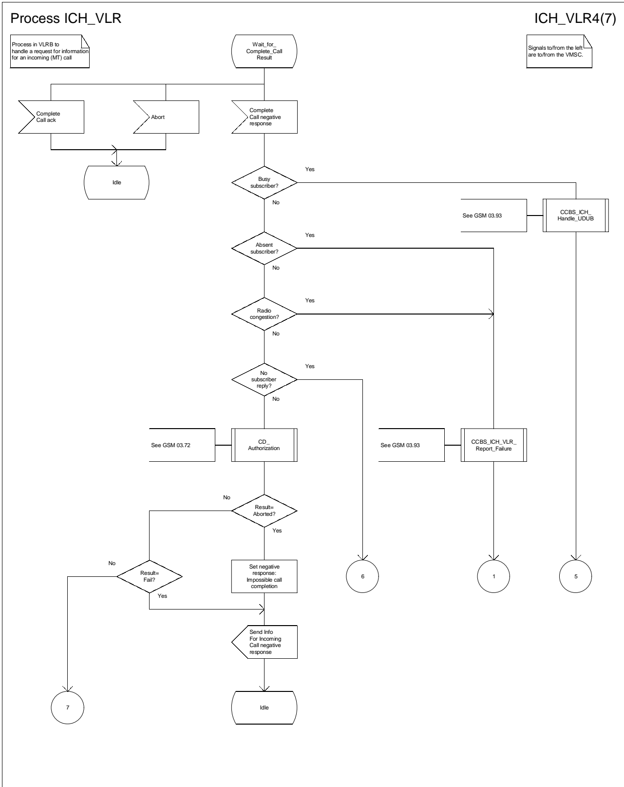
Figure 72d: Process ICH_VLR (sheet 4)
