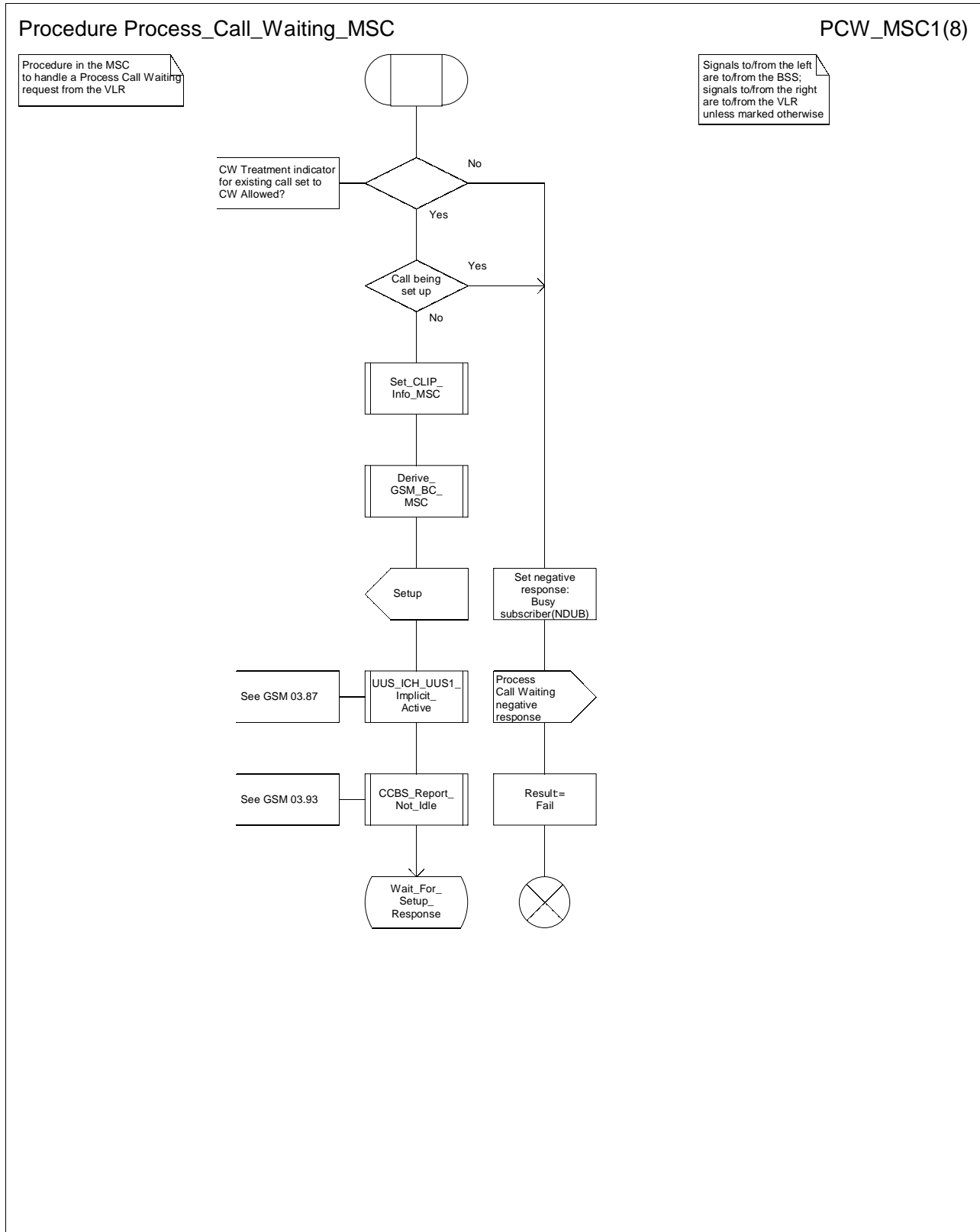
Figure 66a: Procedure Process_Call_Waiting_MSC (sheet 1)
