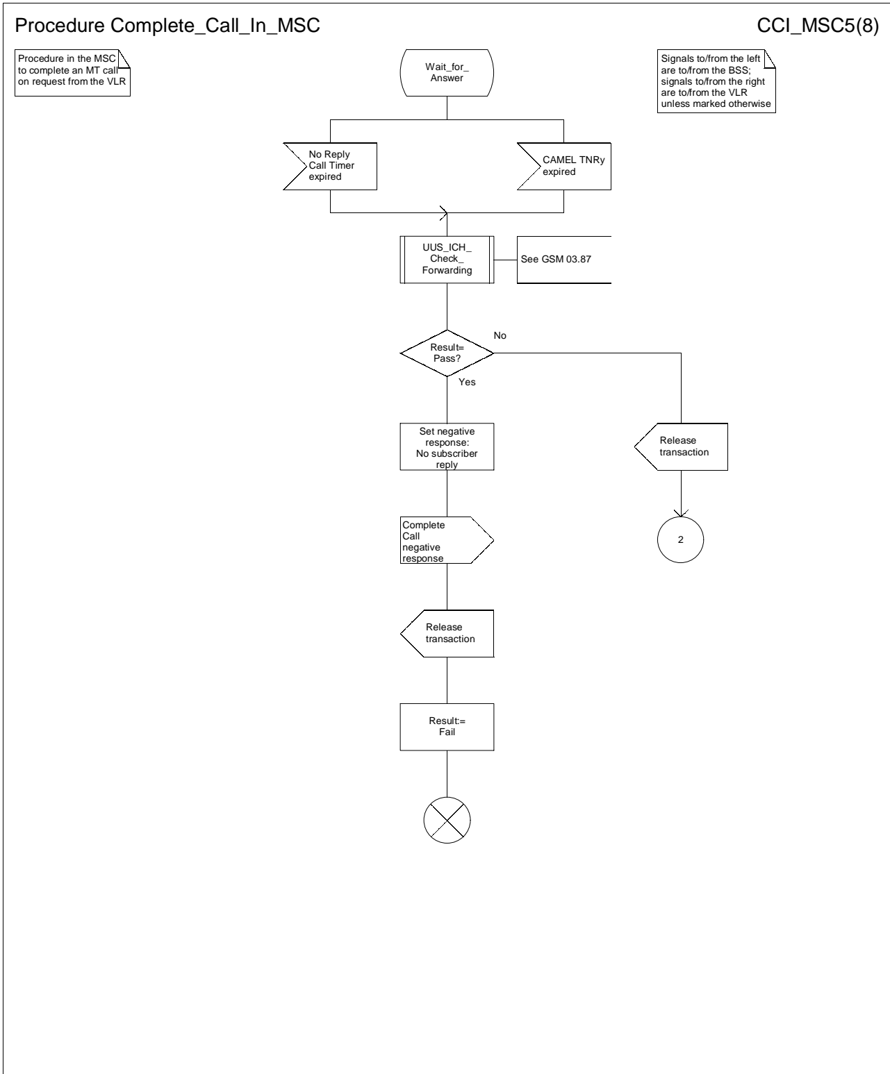
Figure 65e: Procedure Complete_Call_In_MSC (sheet 5)
