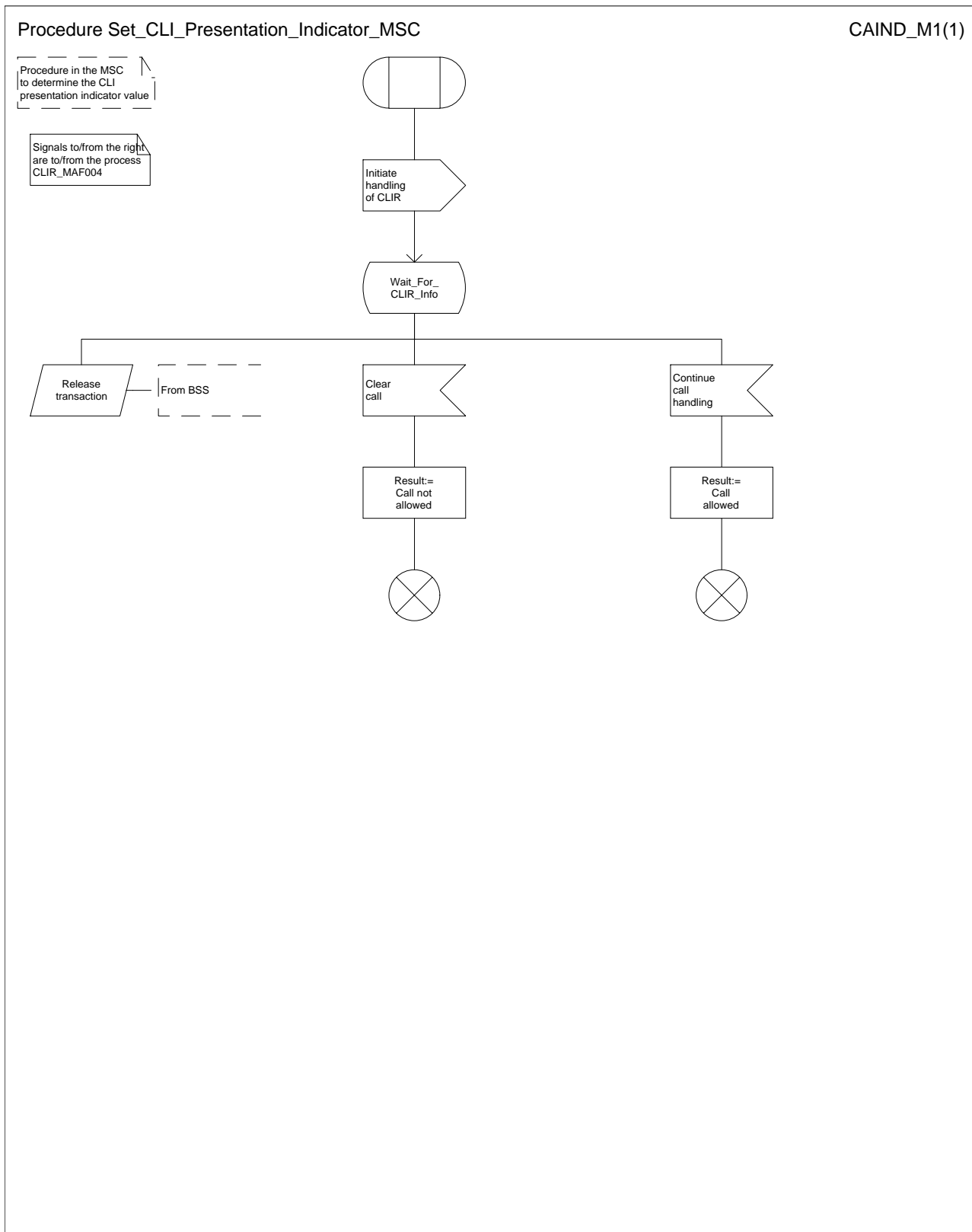
Figure 14: Procedure Set_CLI_Presentation_Indicator_MSC
