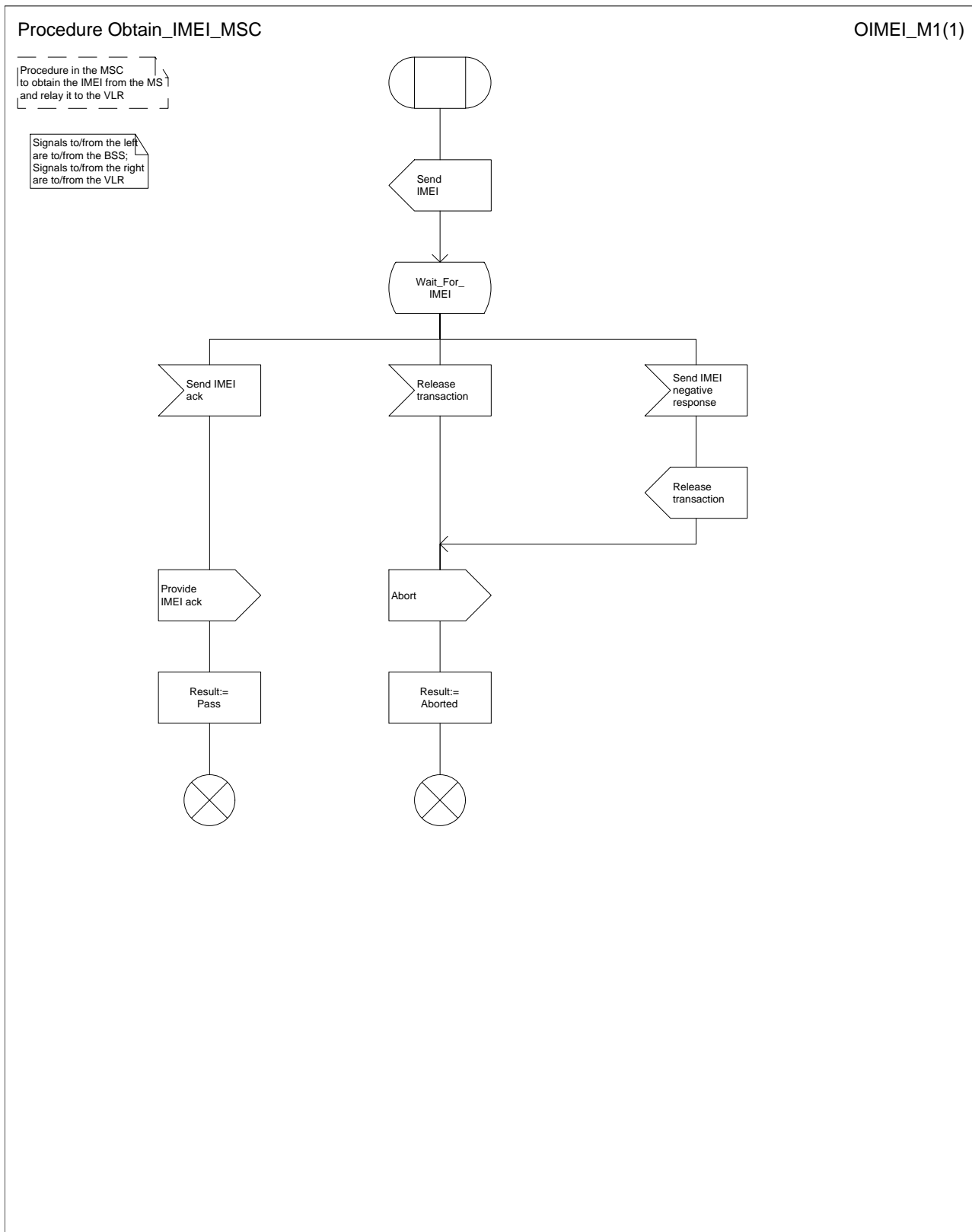
Figure 11: Procedure Obtain_IMEI_MSC
