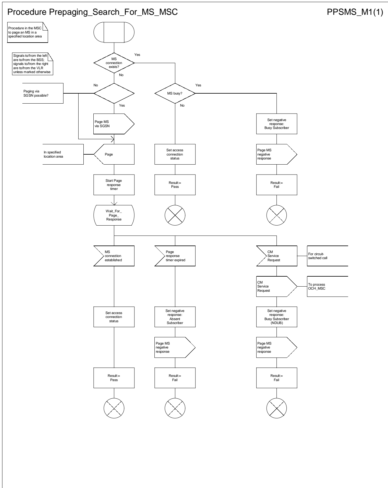
Figure 60: Procedure Prepaging_Search_For_MS_MSC
