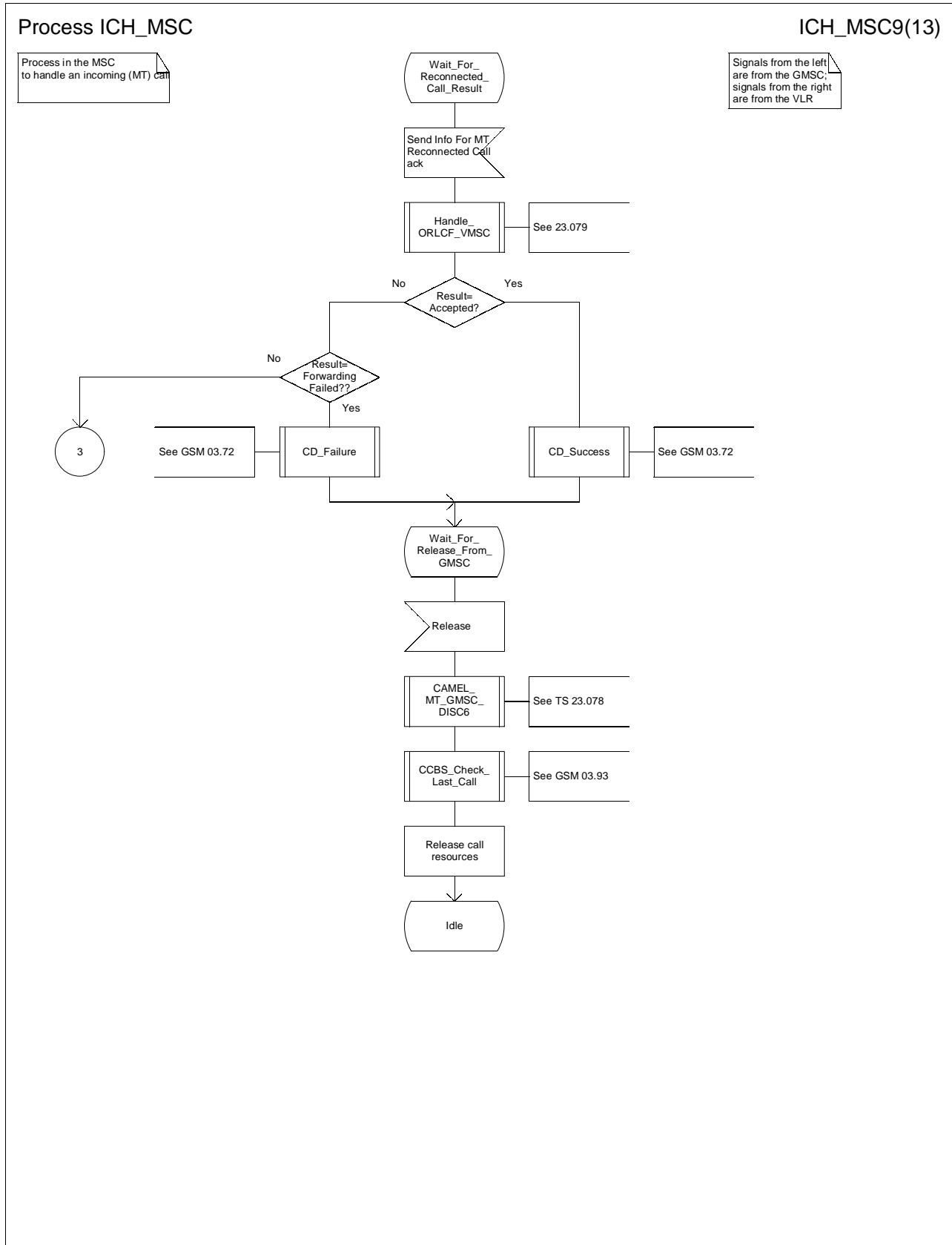
Figure 62i: Process ICH_MSC (sheet 9)
