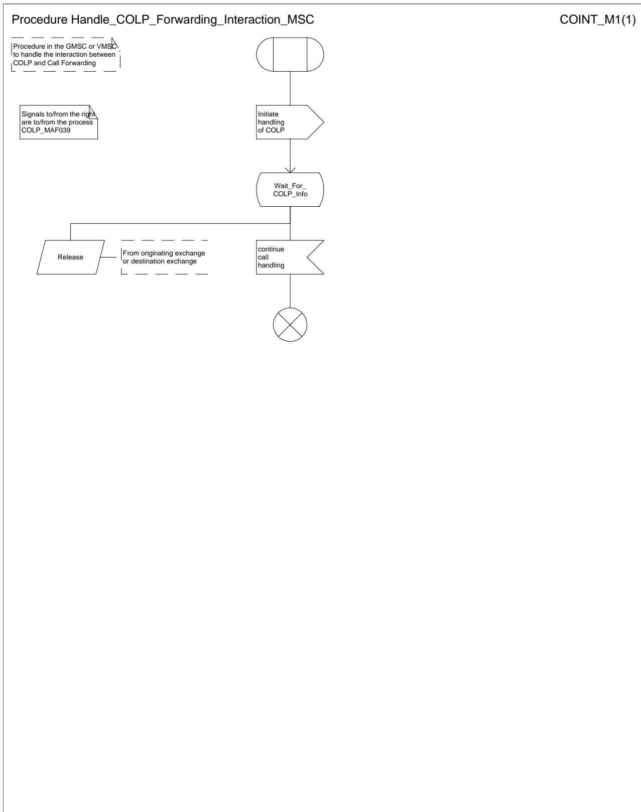
Figure 40: Procedure Handle_COLP_Forwarding_Interaction_MSC
