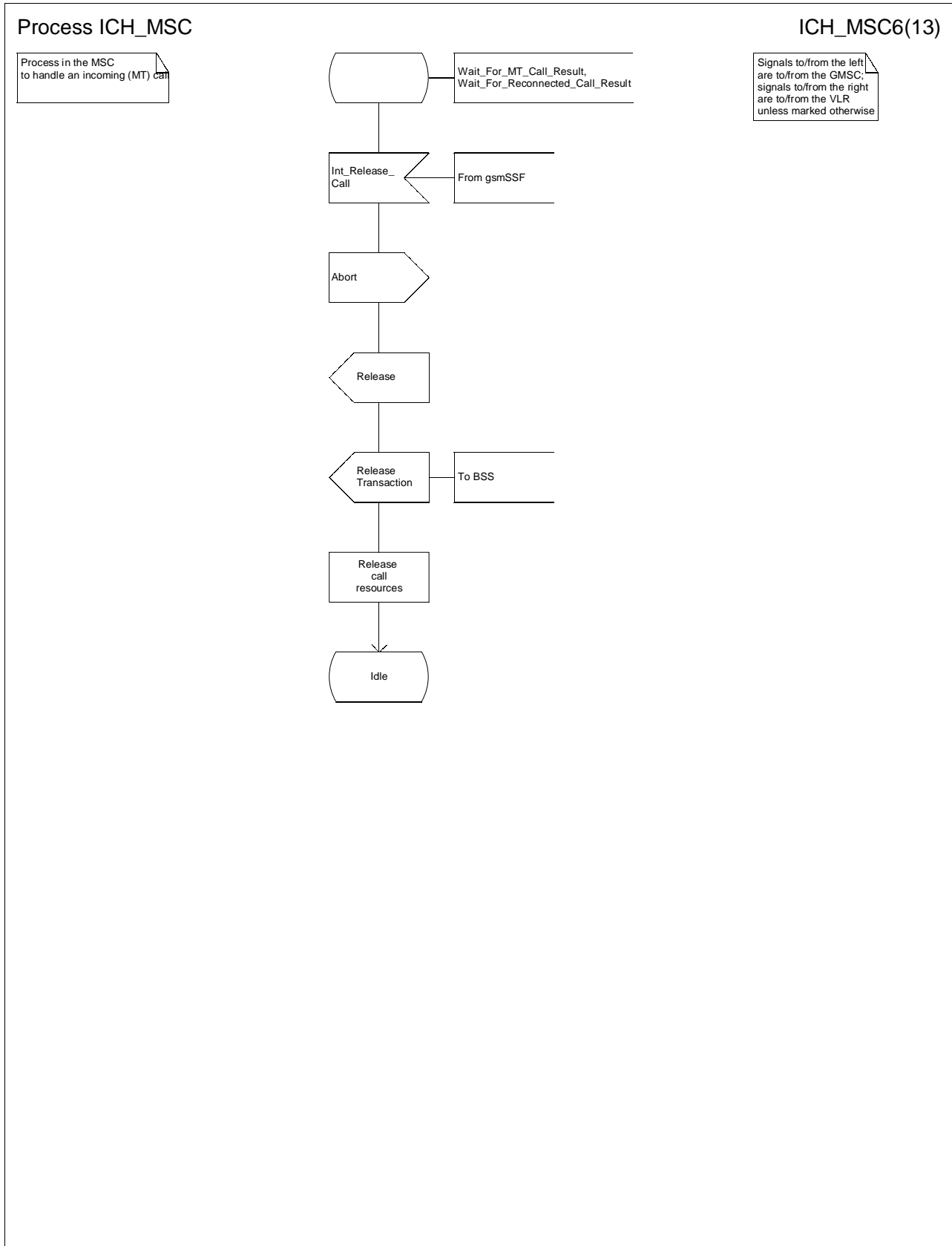
Figure 62f: Process ICH_MSC (sheet 6)
