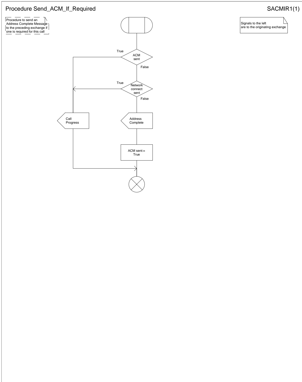
Figure 37: Procedure Send_ACM_If_Required
