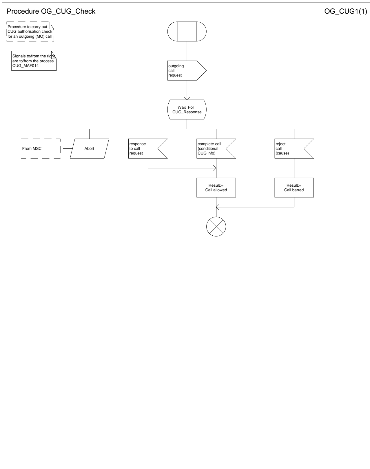
Figure 31: Procedure OG_CUG_Check
