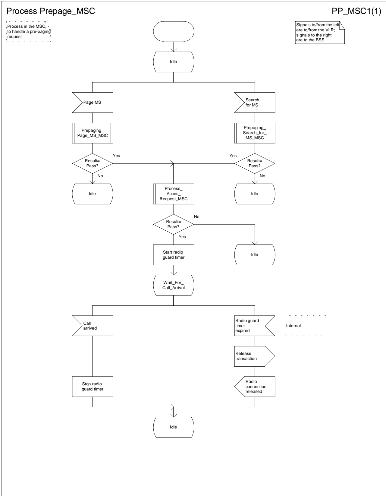
Figure 58: Process Prepage_MSC
