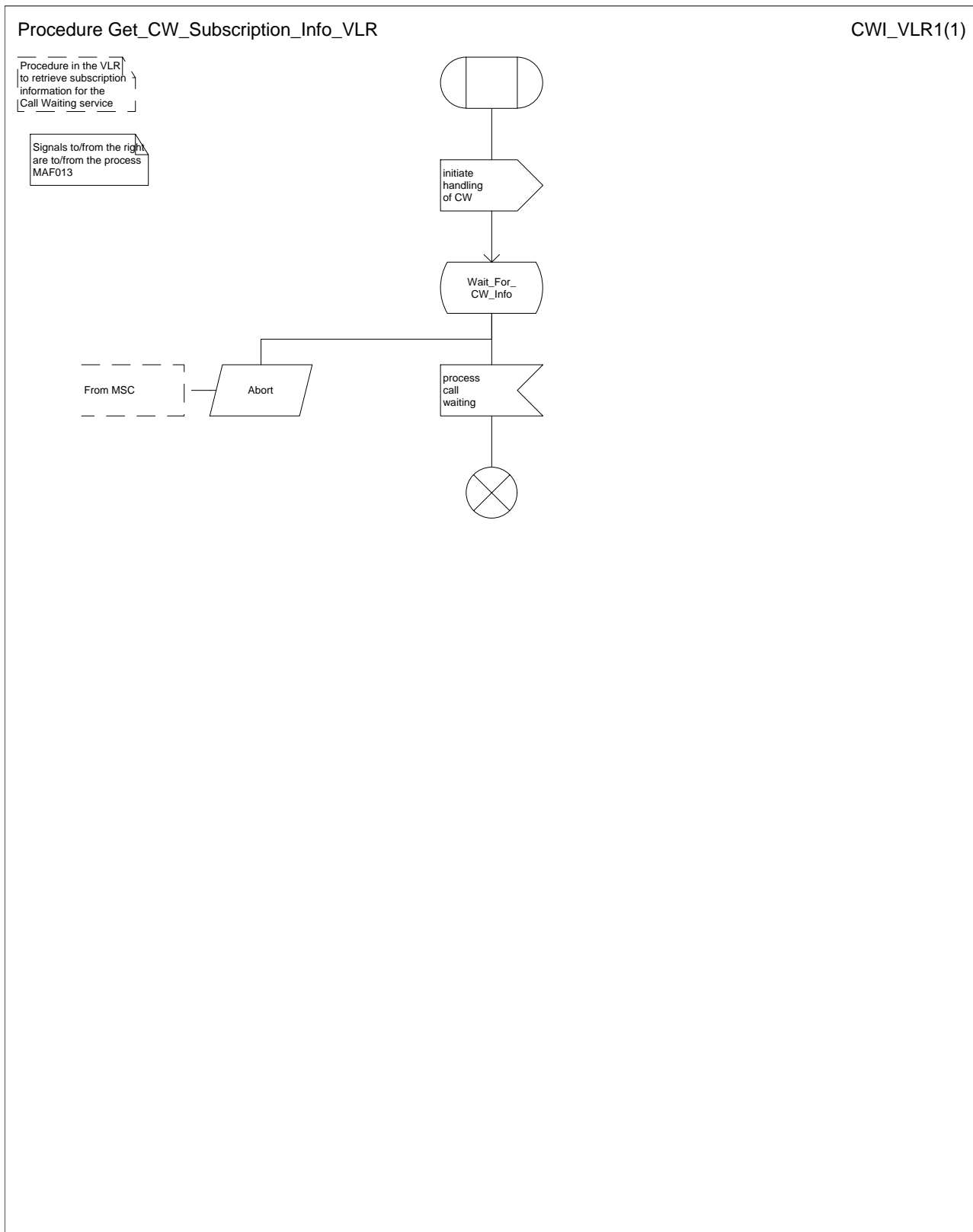
Figure 75: Procedure Get_CW_Subscription_Info_VLR
