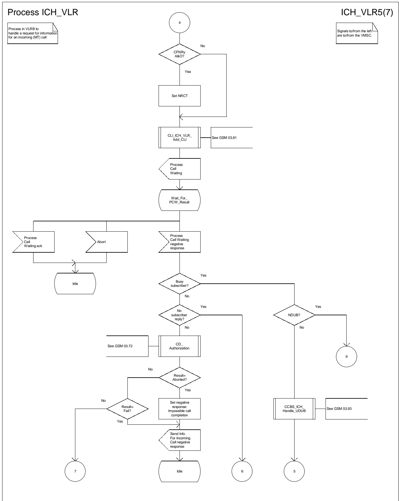
Figure 72e: Process ICH_VLR (sheet 5)
