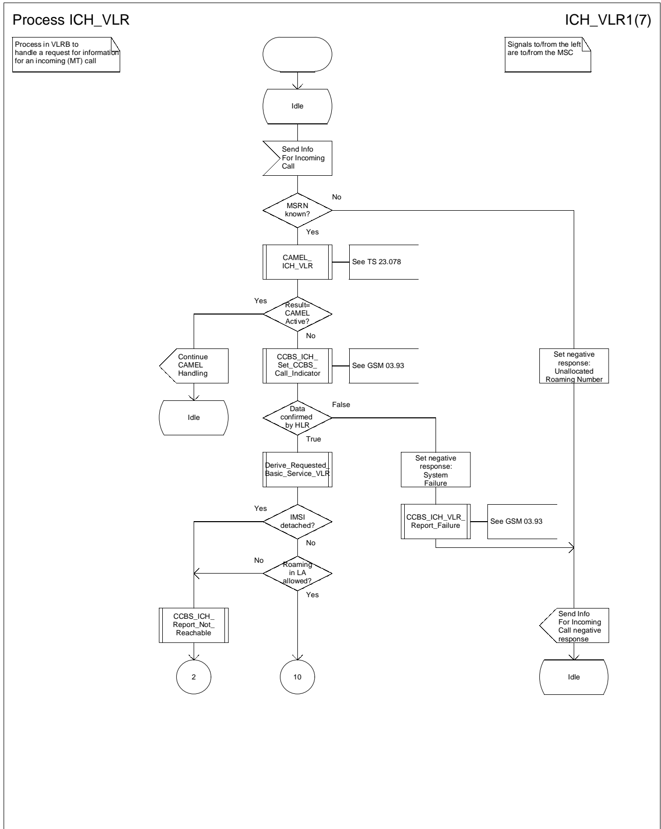
Figure 72a: Process ICH_VLR (sheet 1)
