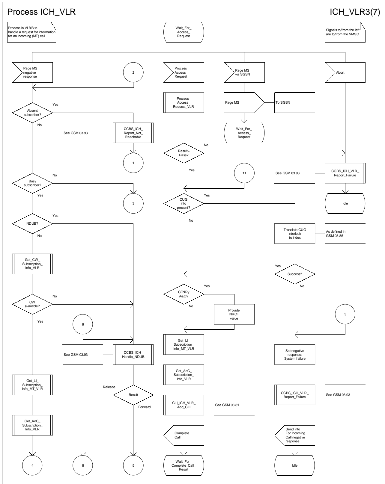
Figure 72c: Process ICH_VLR (sheet 3)
