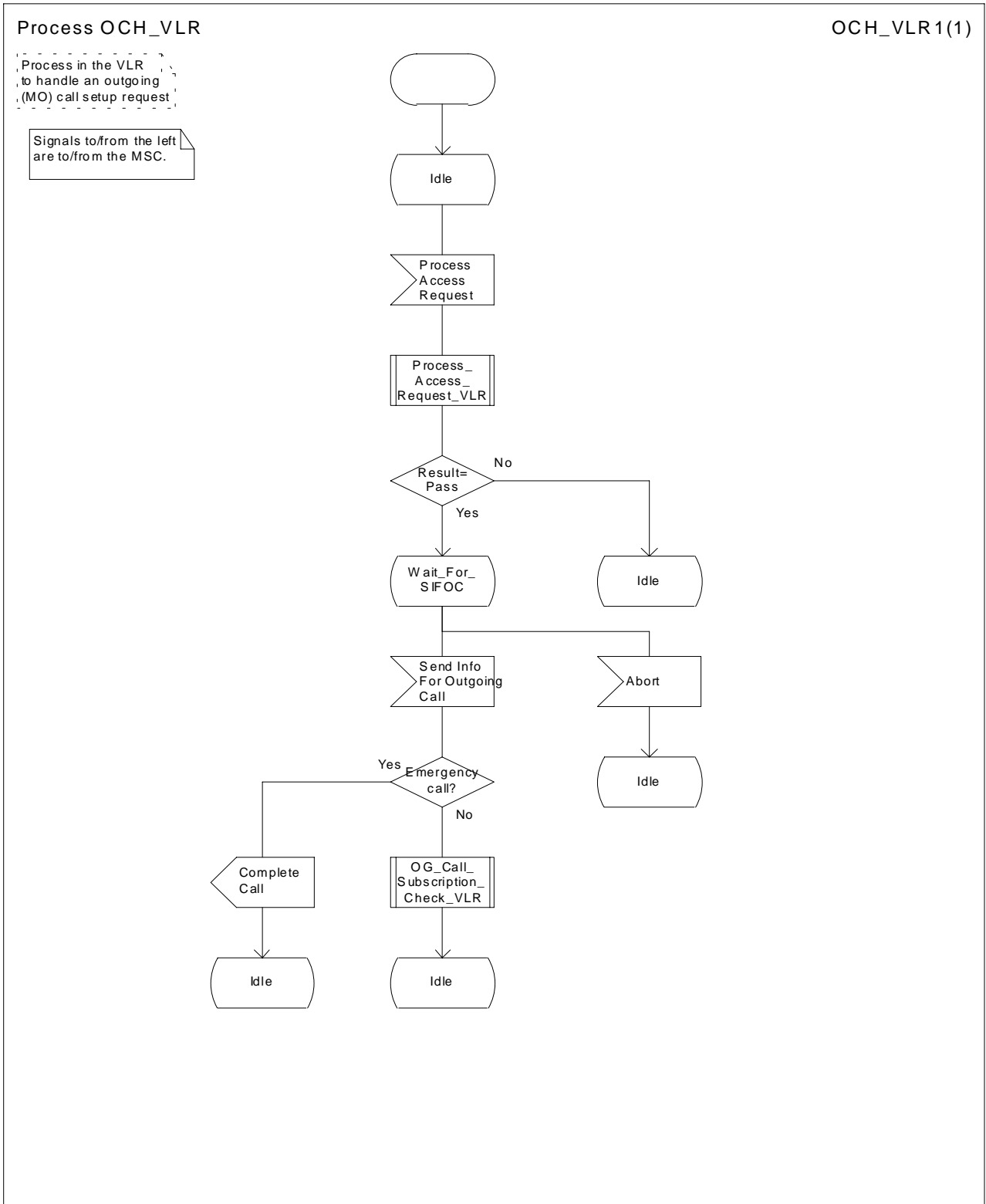
Figure 19: Process OCH_VLR
