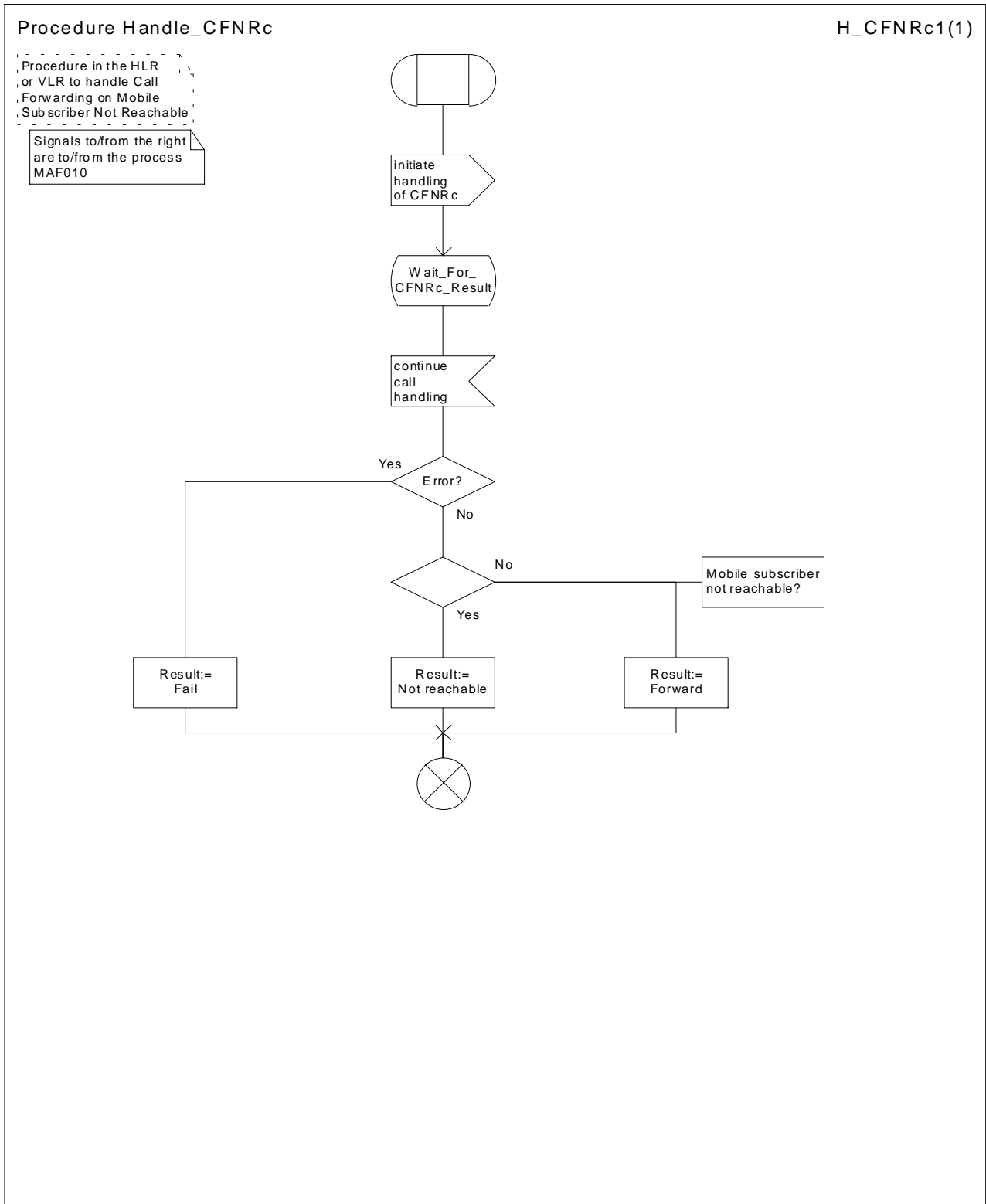
Figure 53: Procedure Handle_CFNRc
