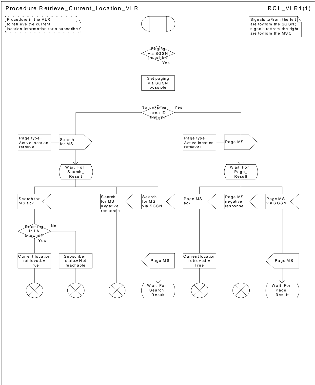
Figure 58: Procedure Retrieve_Current_Location_VLR
