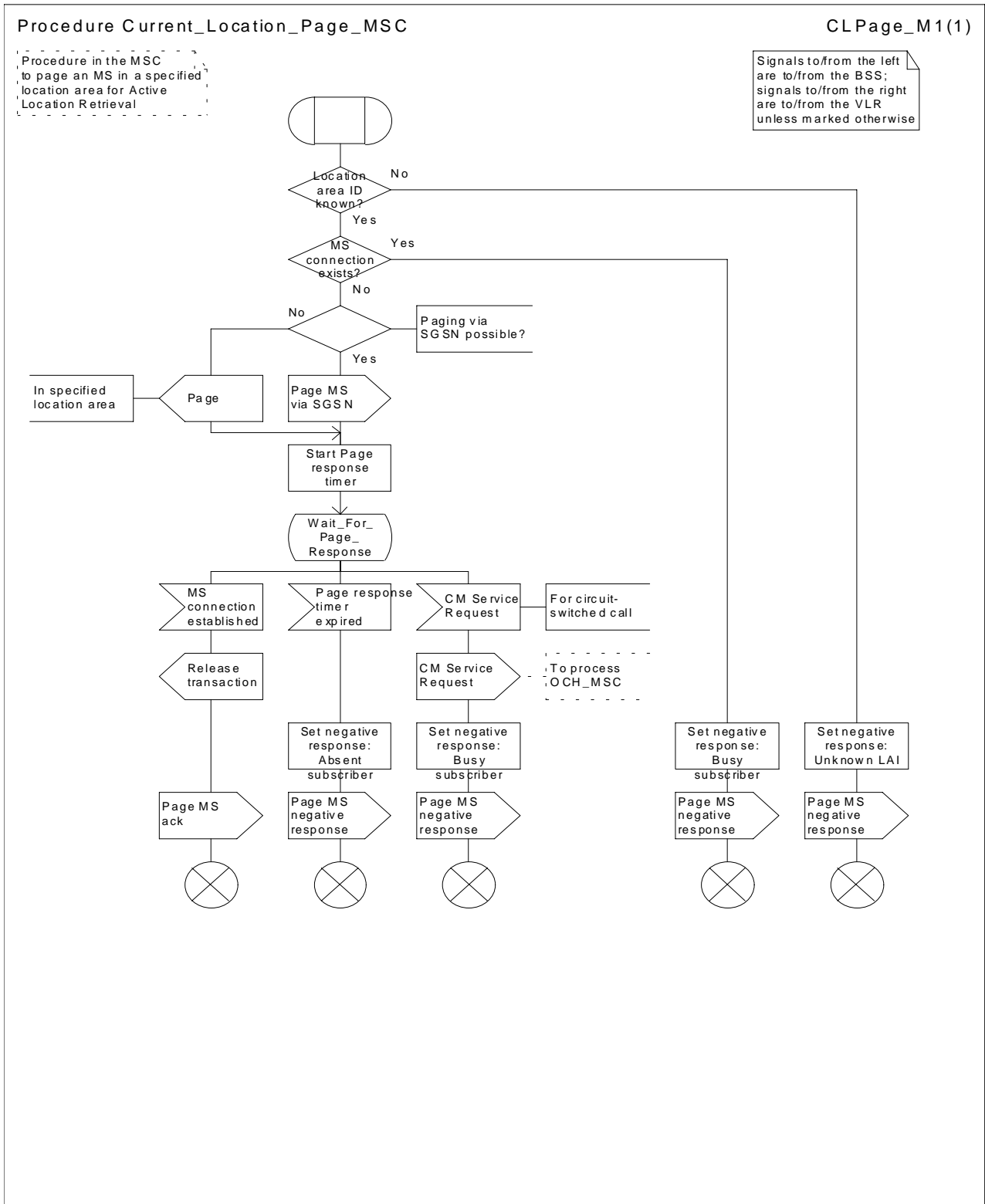
Figure 64: Procedure Current_Location_Page_MSC
