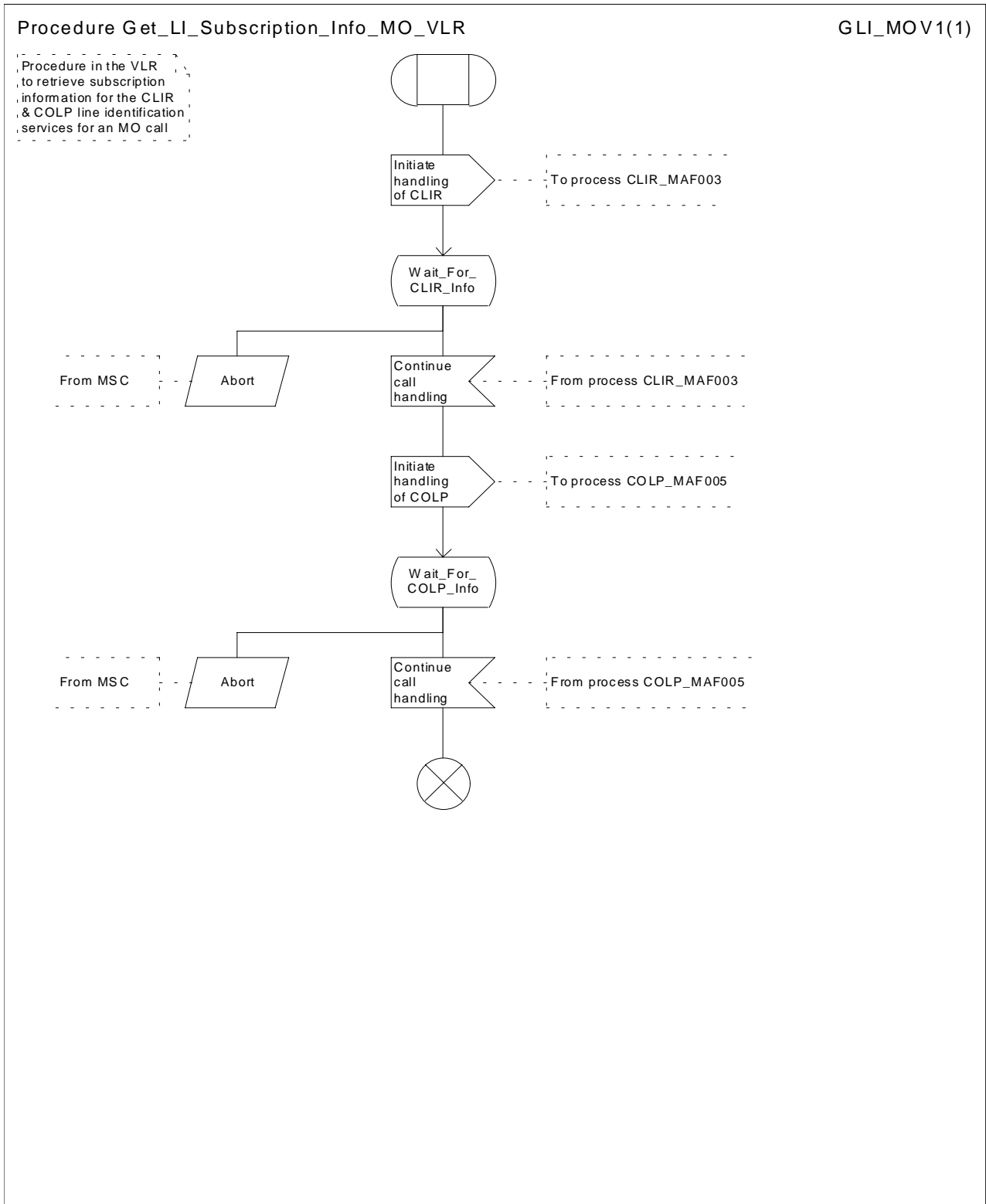
Figure 32: Procedure Get_LI_Subscription_Info_MO_VLR
