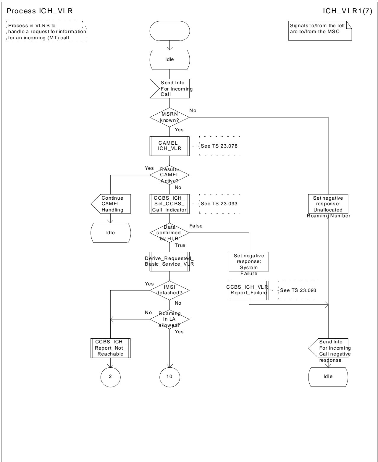
Figure 76a: Process ICH_VLR (sheet 1)
