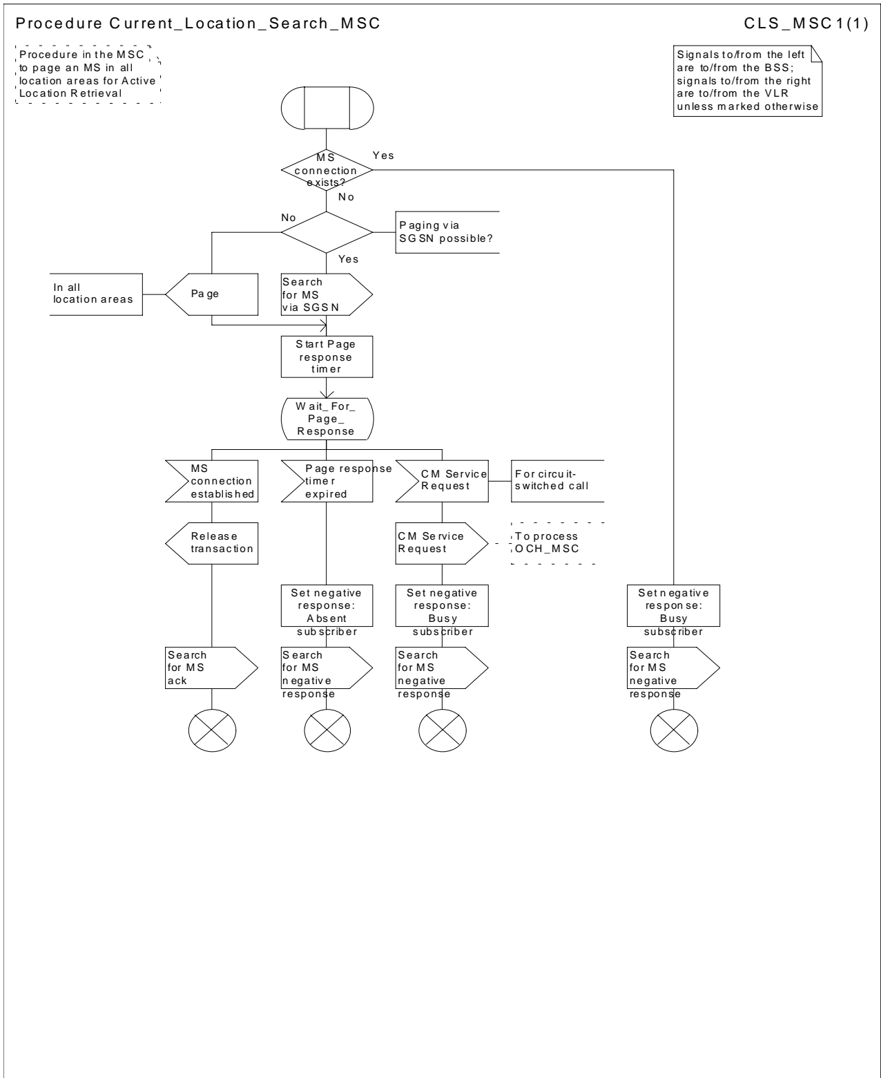
Figure 65: Procedure Current_Location_Search_MSC
