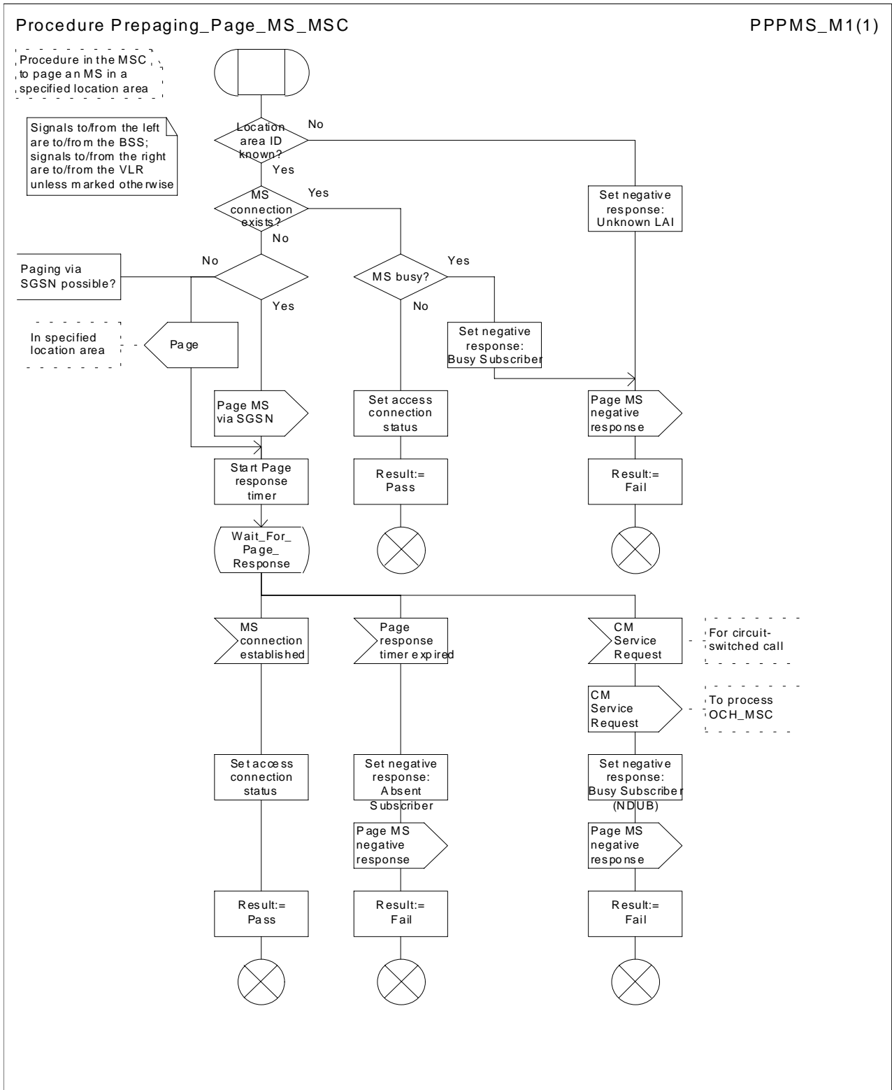
Figure 60: Procedure Preparing_Page_MS_MSC
