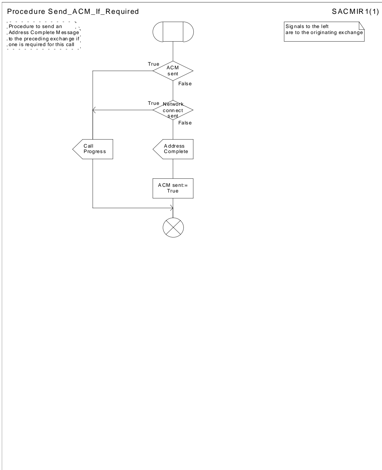
Figure 37: Procedure Send_ACM_If_Required
