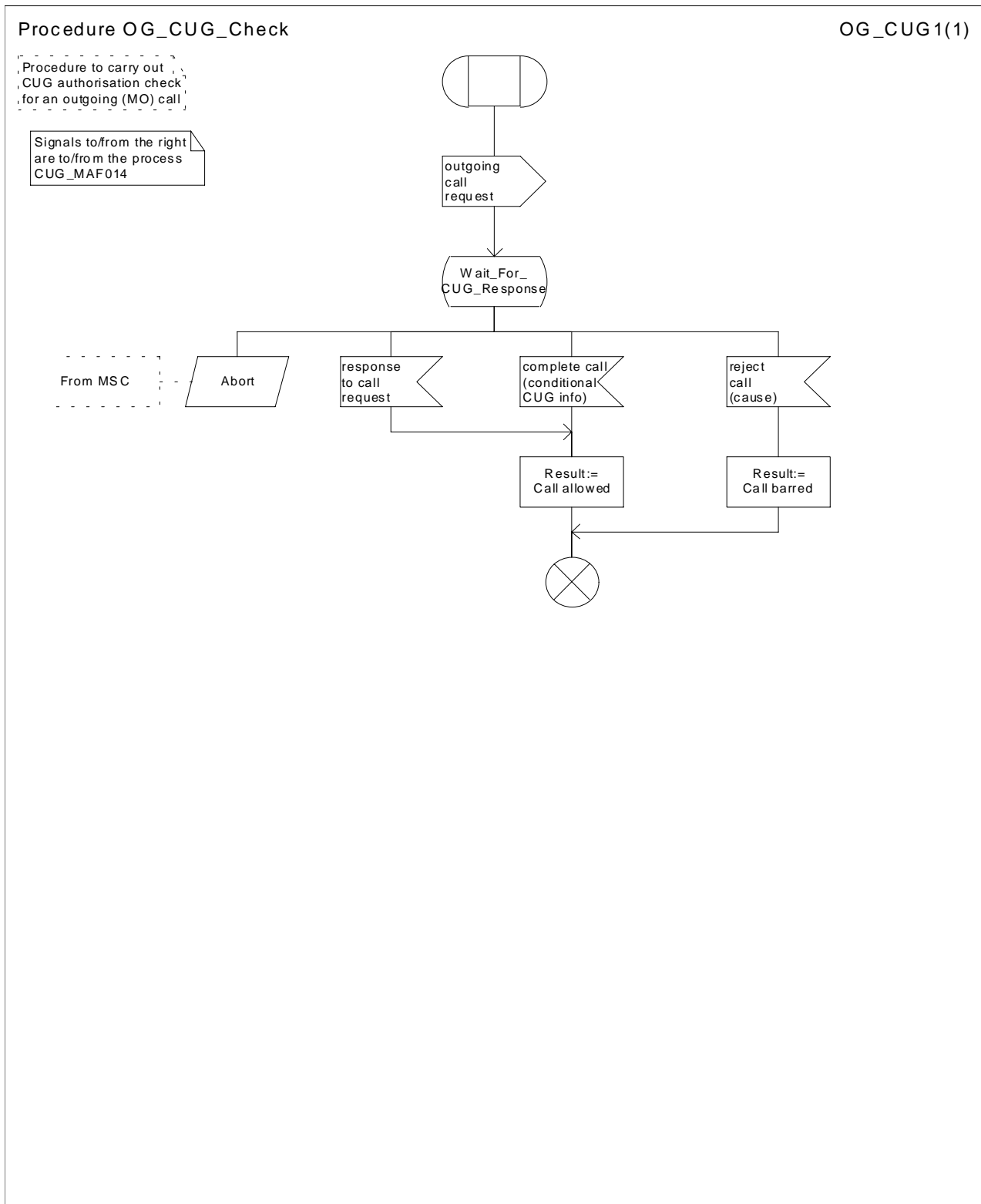
Figure 31: Procedure OG_CUG_Check
