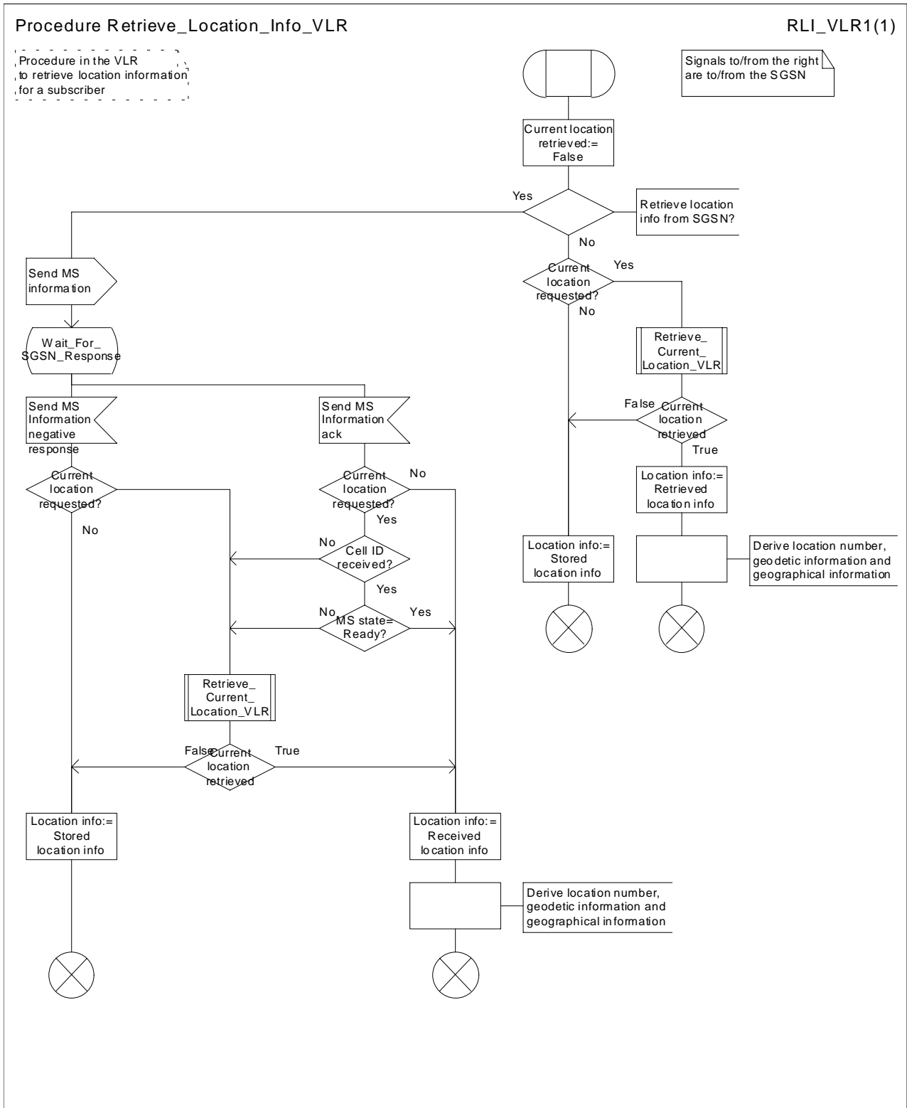
Figure 57: Procedure Retrieve_Location_Info_VLR
