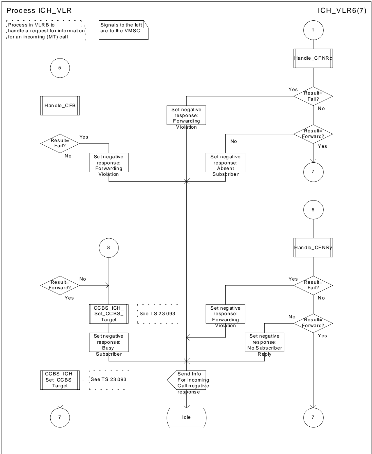
Figure 76f: Process ICH_VLR (sheet 6)
