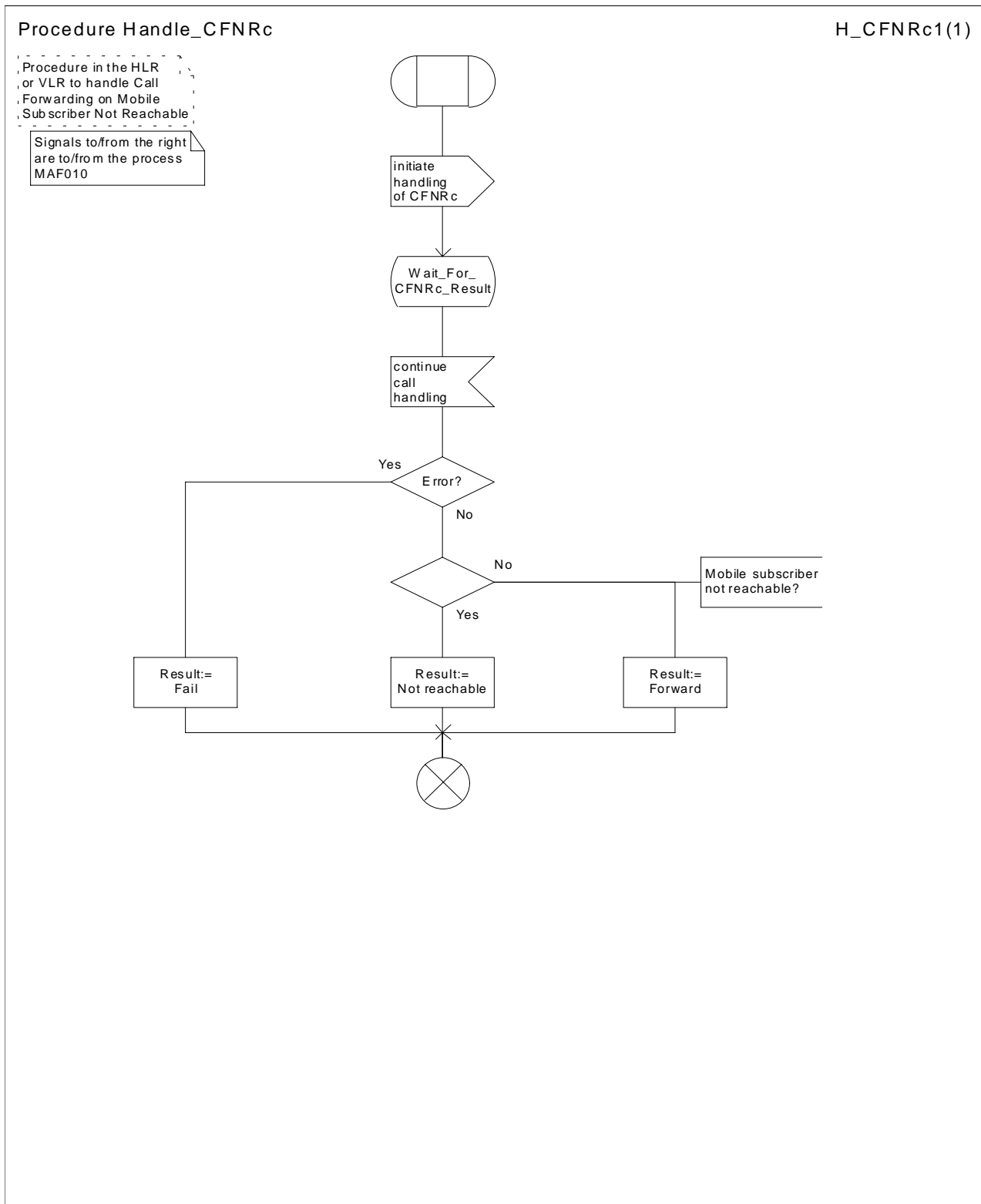
Figure 53: Procedure Handle_CFNRc
