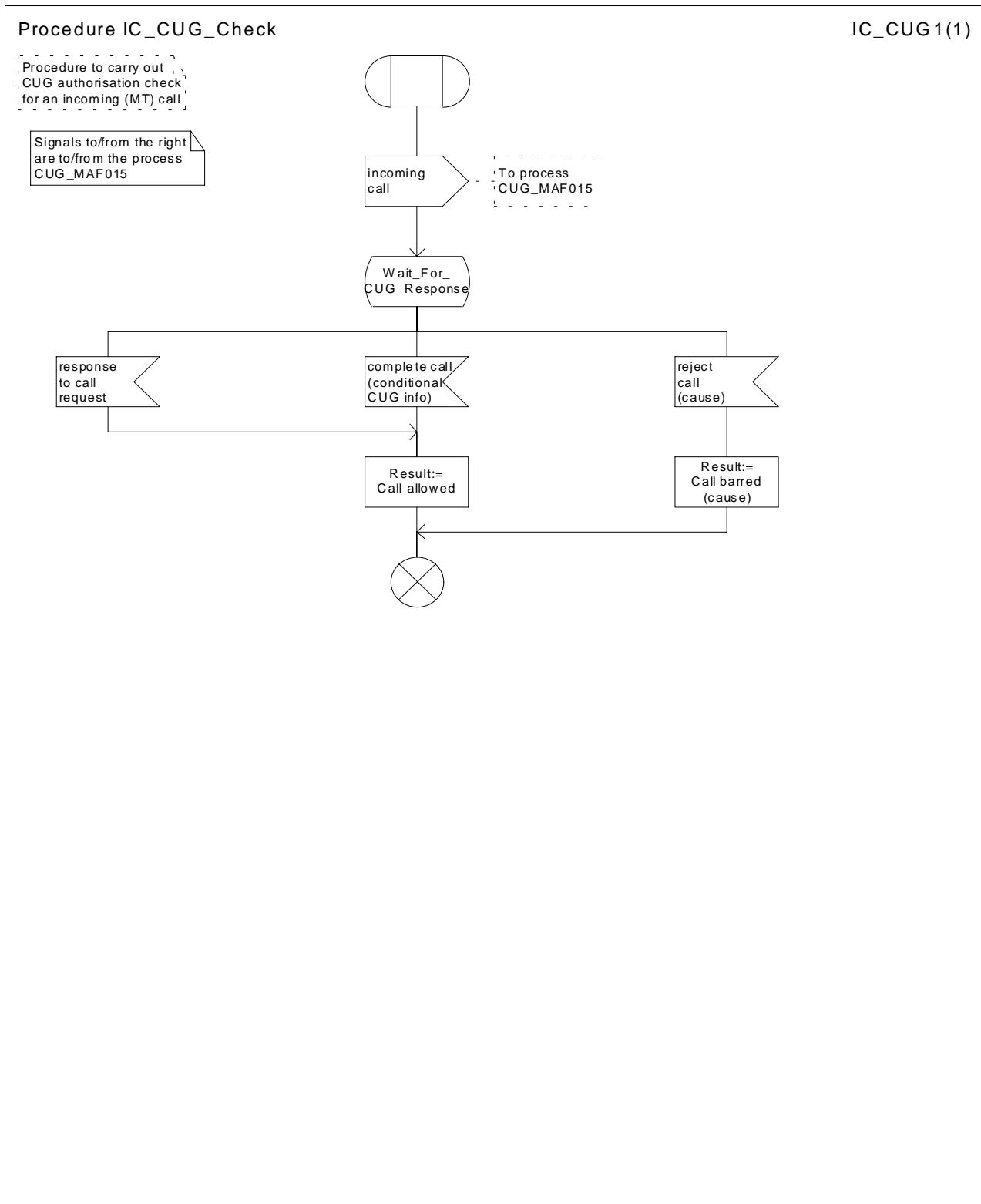
Figure 51: Procedure IC_CUG_Check
