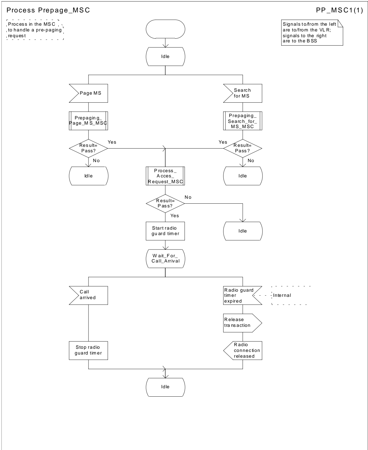
Figure 59: Process Prepage_MSC
