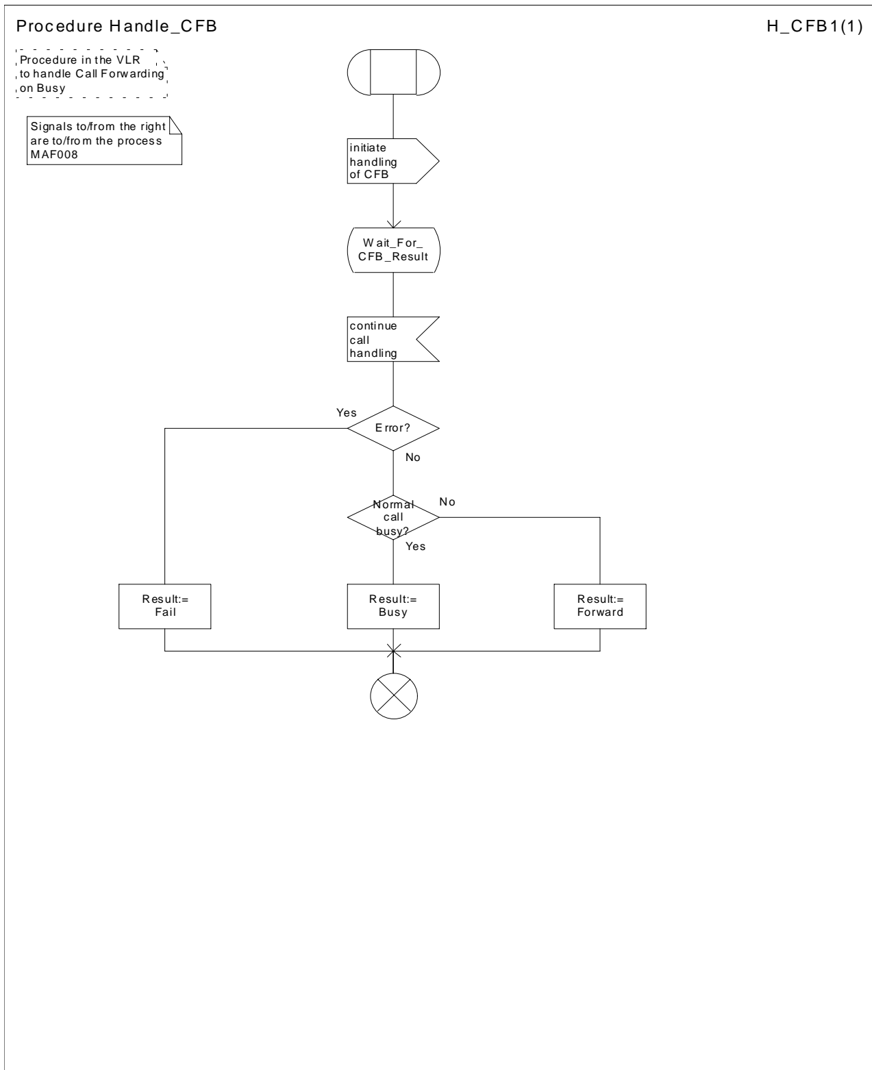
Figure 81: Procedure Handle_CFB
