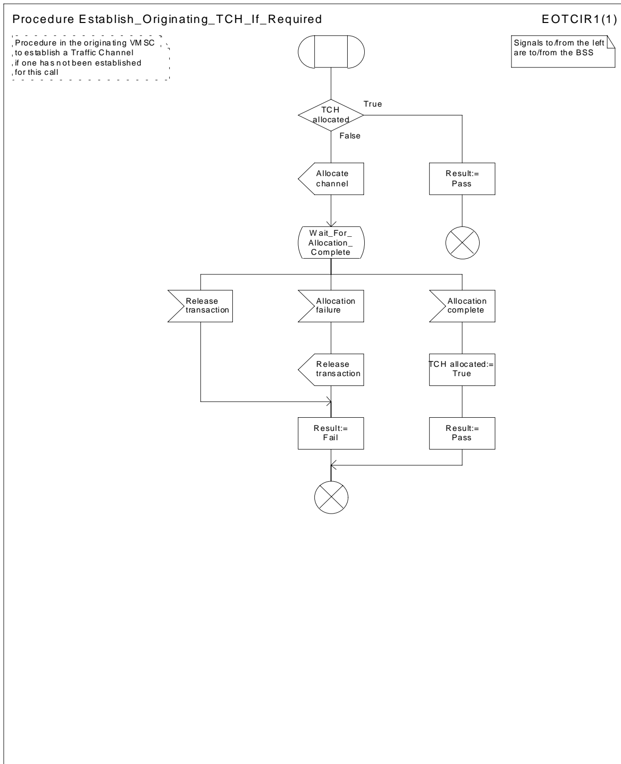
Figure 13: Procedure Establish_Originating_TCH_If_Required
