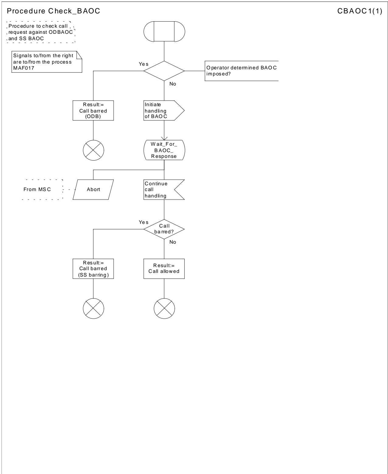
Figure 30: Procedure Check_BAOC
