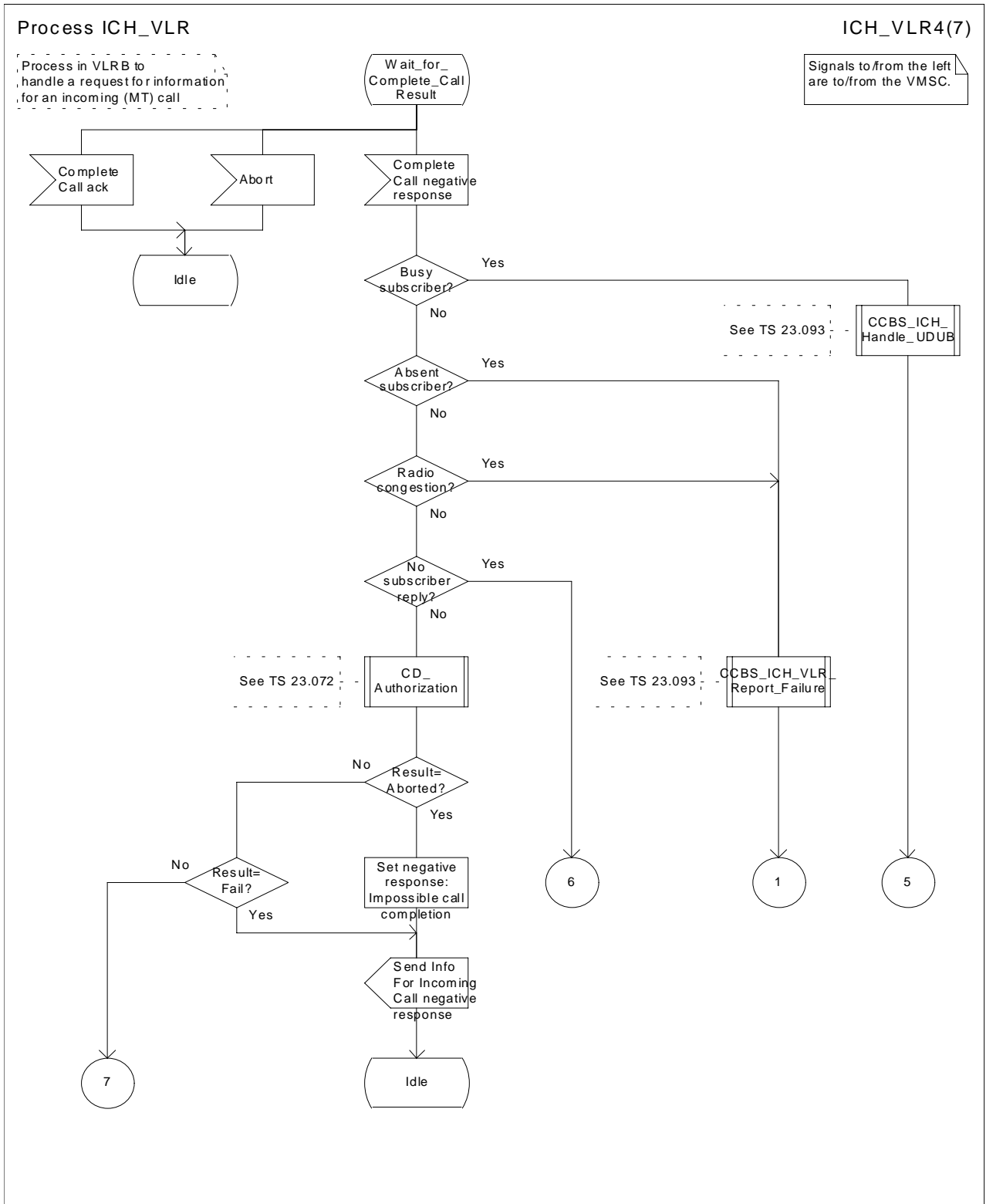
Figure 76d: Process ICH_VLR (sheet 4)
