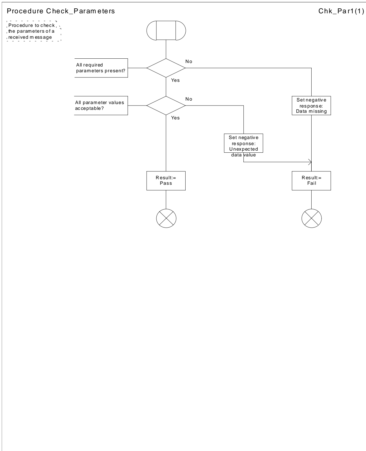
Figure 44: Procedure Check_Parameters
