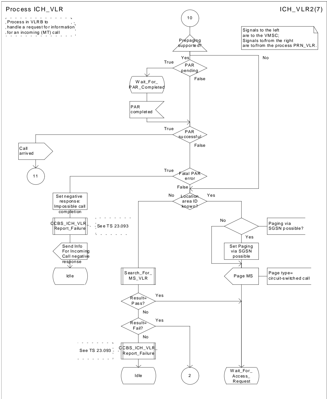
Figure 72b: Process ICH_VLR (sheet 2)
