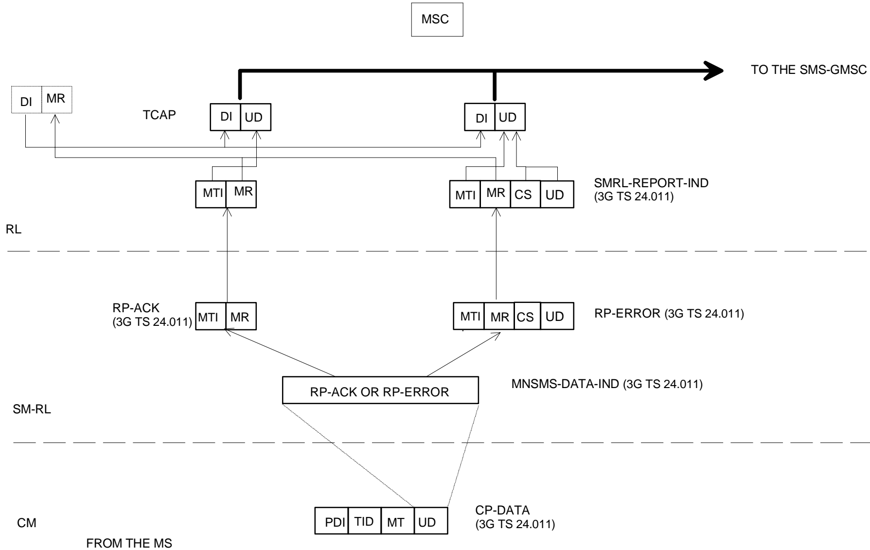
Figure C.6: Acknowledgement in the MT case
