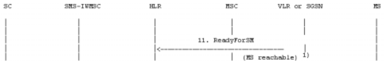
Figure 20a: The alert procedure when the MS becomes reachable, MNR, MNRG or both are set and MCEF is not set
