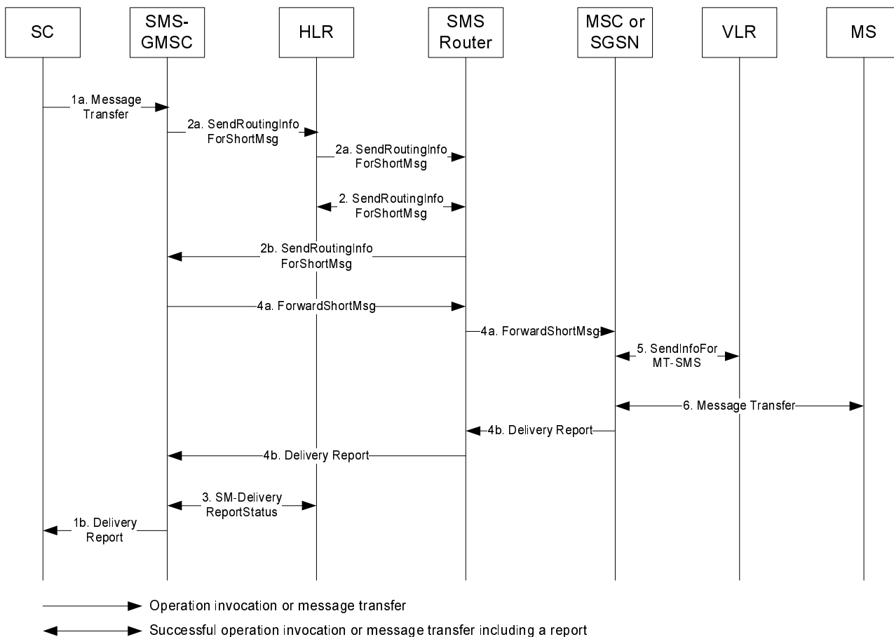
Figure 15a): Successful short message transfer attempt via the SMS Router, and the MSC or SGSN
