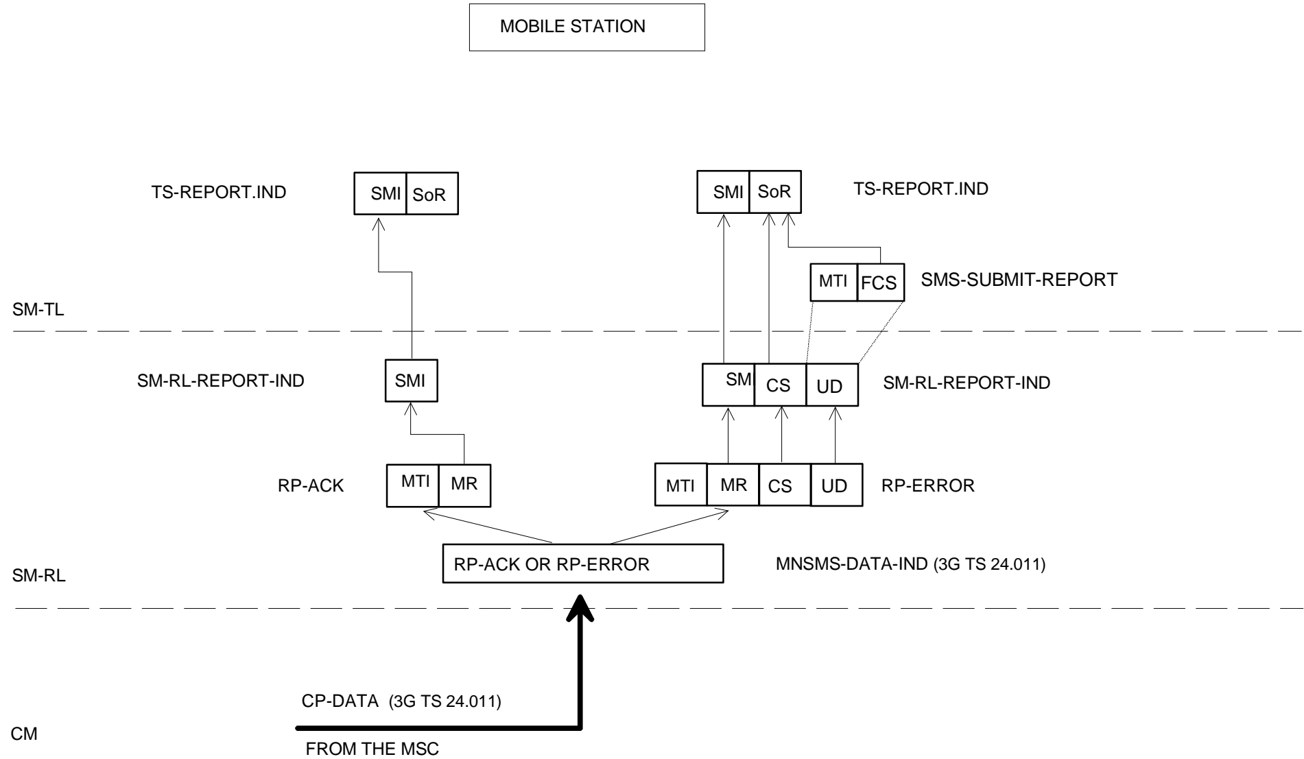
Figure C.16: Acknowledgement in the MO case
