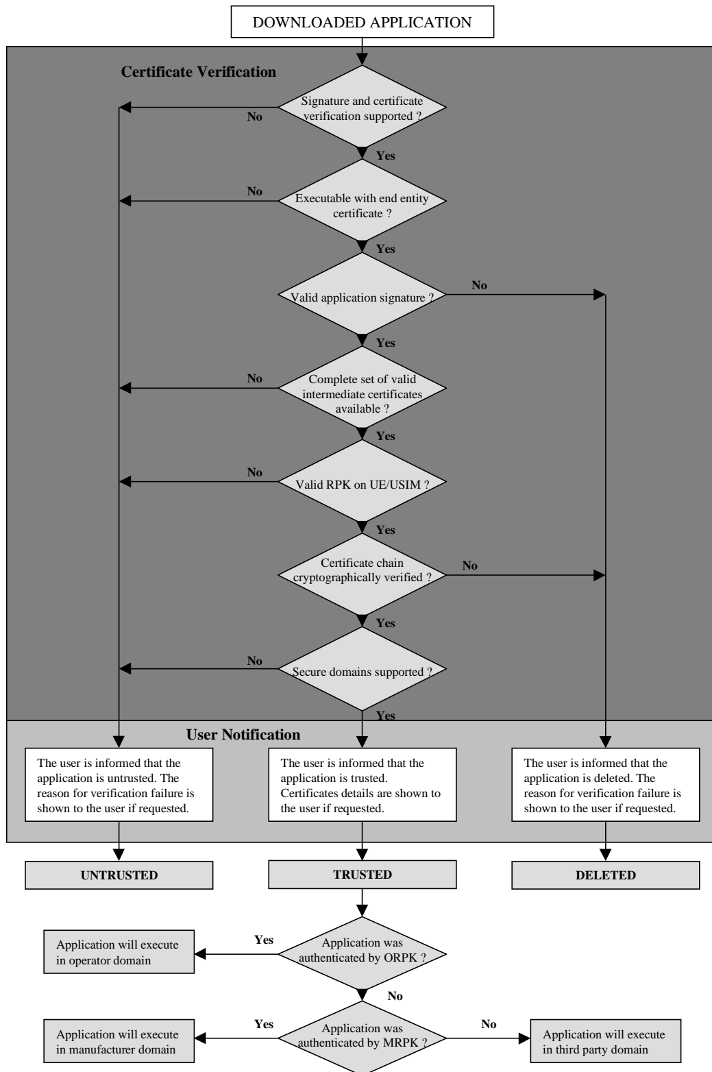
Figure 6A "Certificate Chain Verification Diagram"
