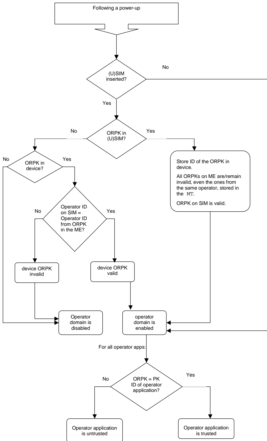
Figure 8: MExE device behaviour on power up
