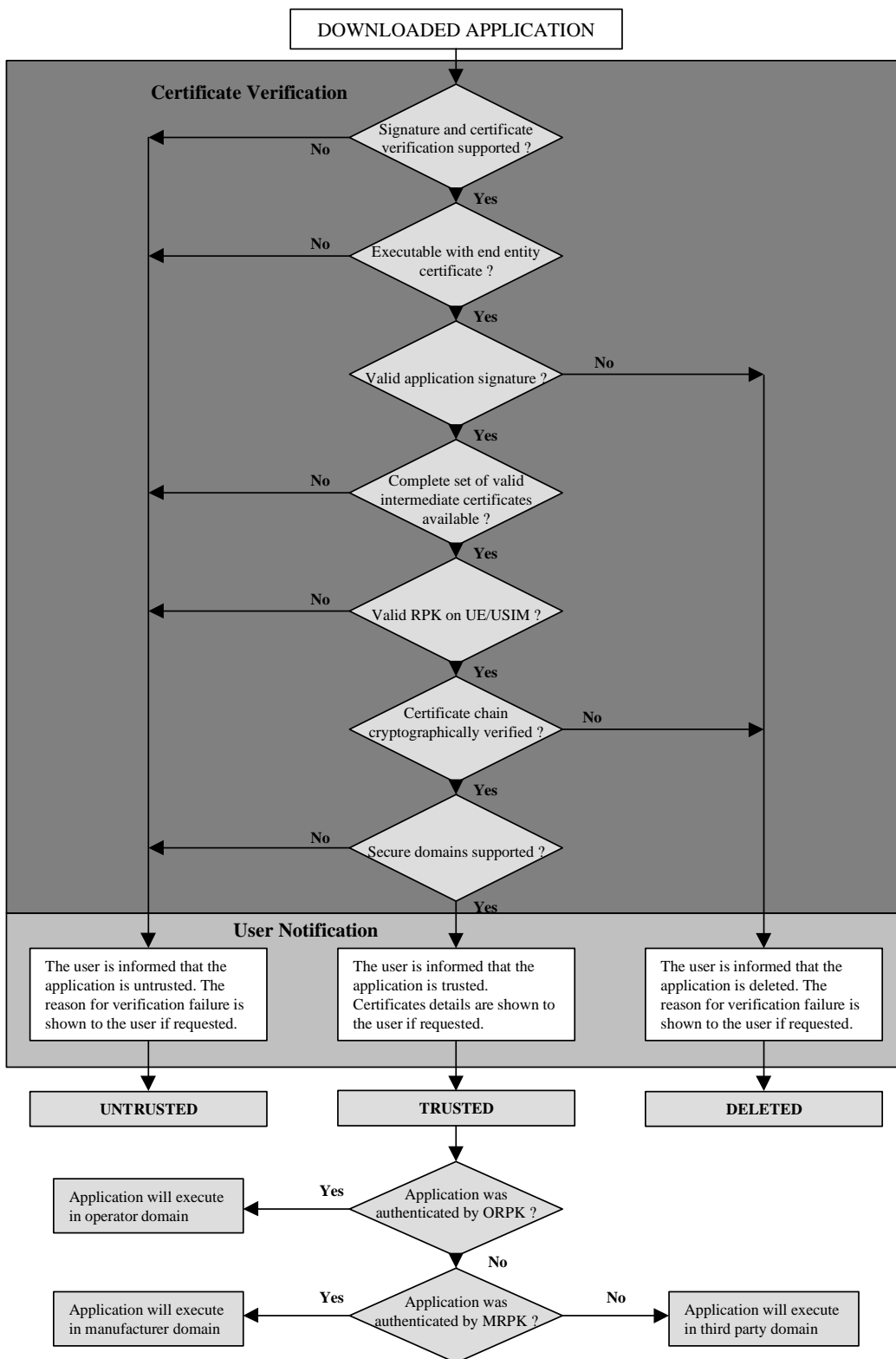
Figure 7: Certificate Chain Verification Diagram
