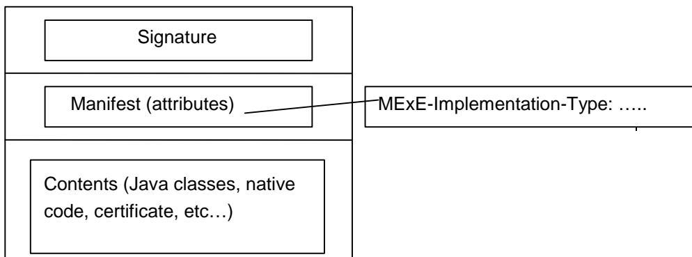
Figure 14: Signed packages
