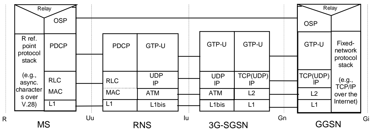
Figure 79: UMTS User Plane for PDP Type OSP
