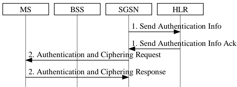
Figure 28: Authentication of GSM Subscriber in GSM Procedure
