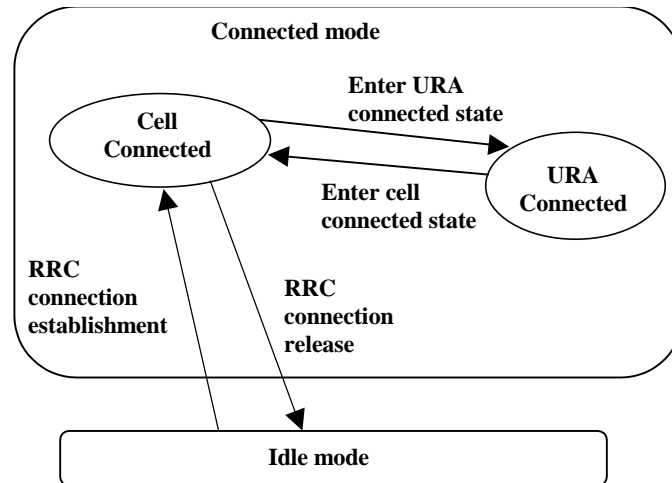
Figure 54: RRC Modes, Main RRC States and Main Mode and State Transition
