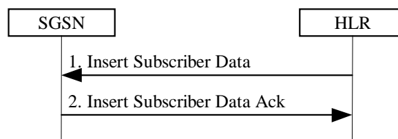
Figure 45: Insert Subscriber Data Procedure
