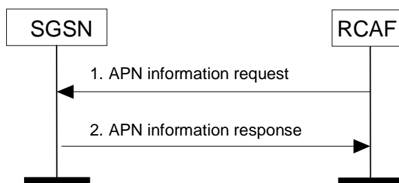
Figure 6.17-1: APN information retrieval procedure
