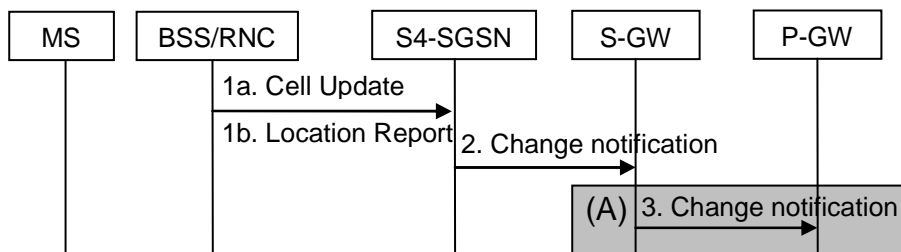
Figure 15.1.3.3-1: Reporting of Presence Reporting Area entering and leaving
