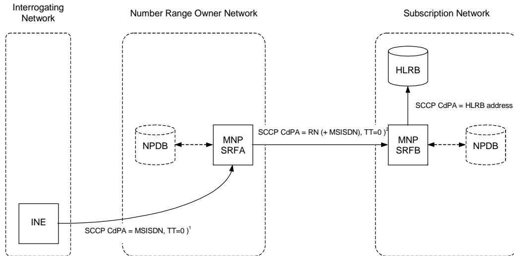
Figure B.2.3: MNP-SRF operation for indirectly routeing (i.e. via the number range owner network) a non-call related signalling message for a ported subscriber.
