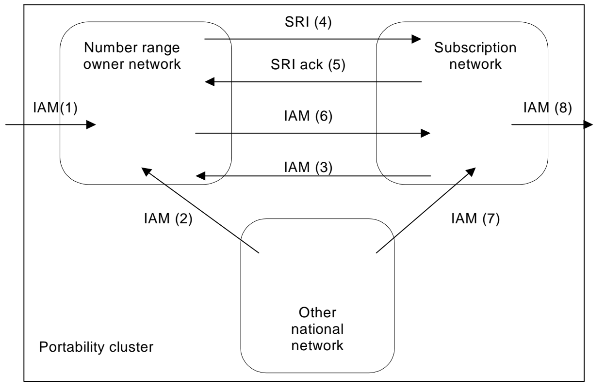
Figure 3 General architecture of a portability cluster for routing of calls
