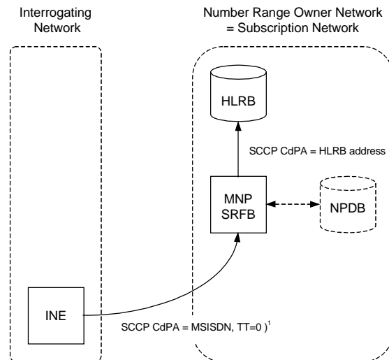
Figure B.2.1: MNP-SRF operation for routing a non-call related signalling message for a non-ported number where the interrogating network is inside the portability cluster and indirect routeing is used or the interrogating network is outside the portability cluster.
