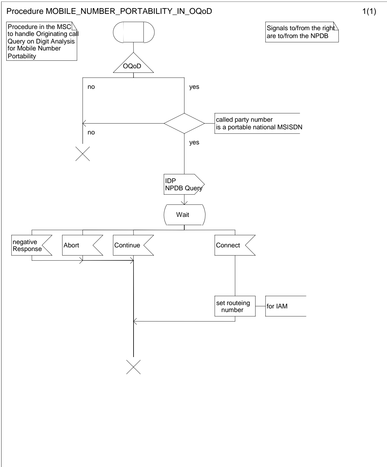
Figure A.15: Procedure MOBILE_NUMBER_PORTABILITY_IN_OQoD
