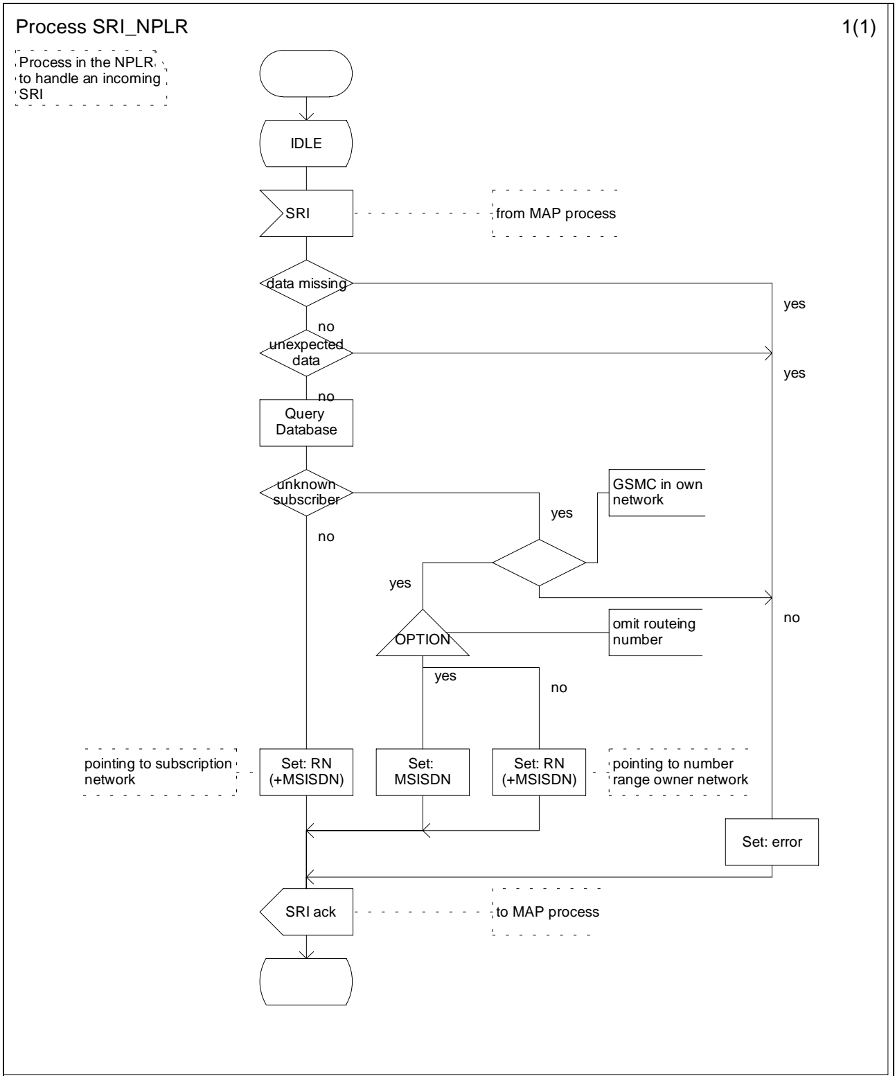
Figure C.2.2: Process SRI_NPLR
