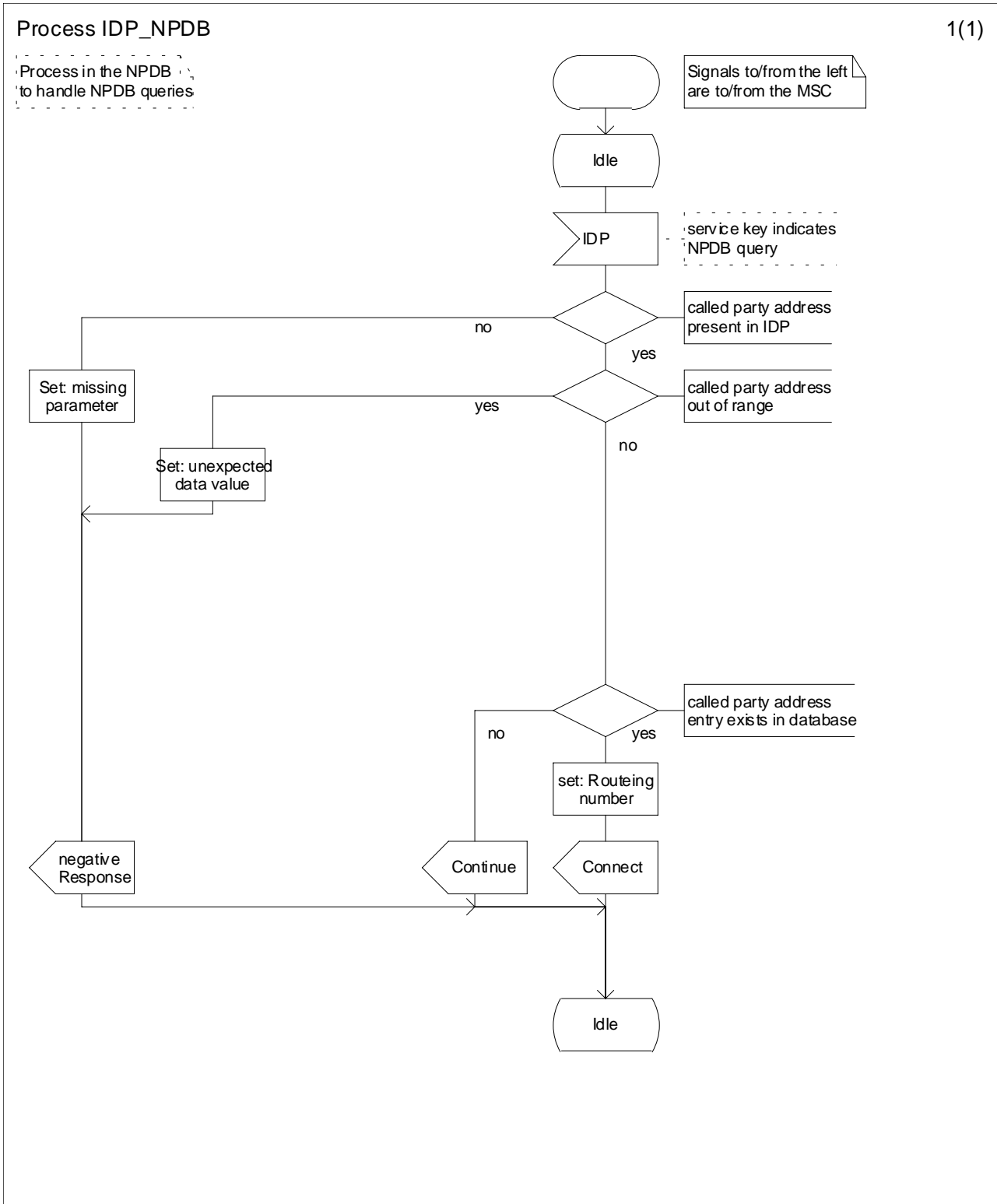
Figure A.16: Process IDP_NPDB
