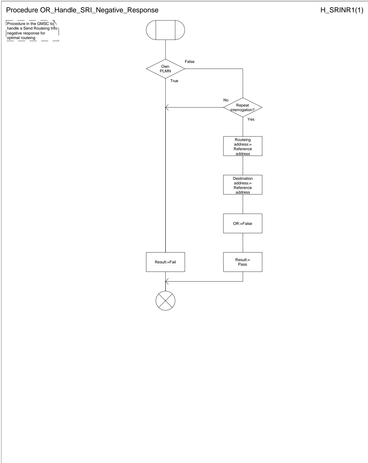
Figure 9: Procedure OR_Handle_SRI_Negative_Response
