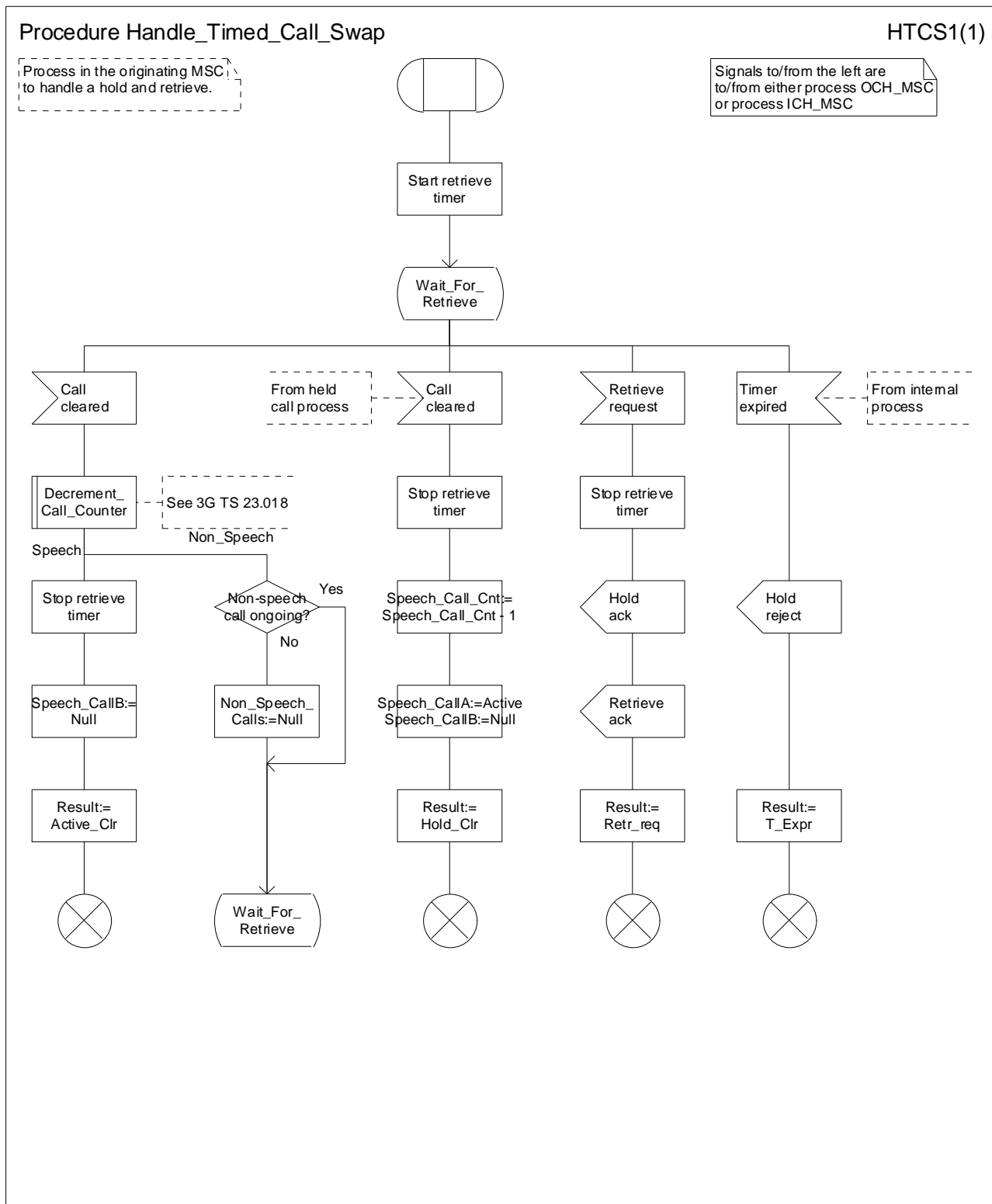
Figure 2.2c: Procedure Handle_Timed_Call_Swap
