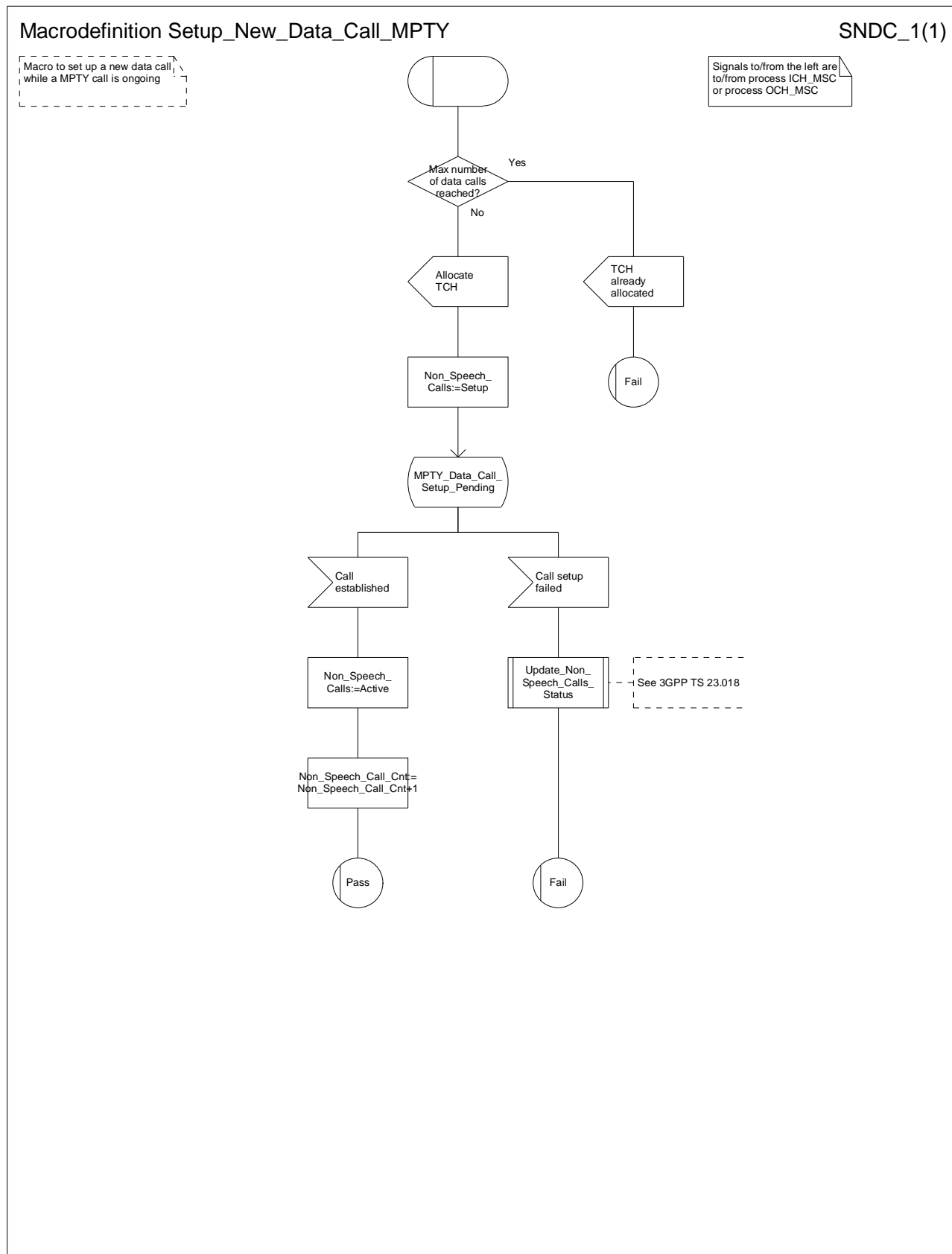
Figure 1.4: Setup_New_Data_Call_MPTY
