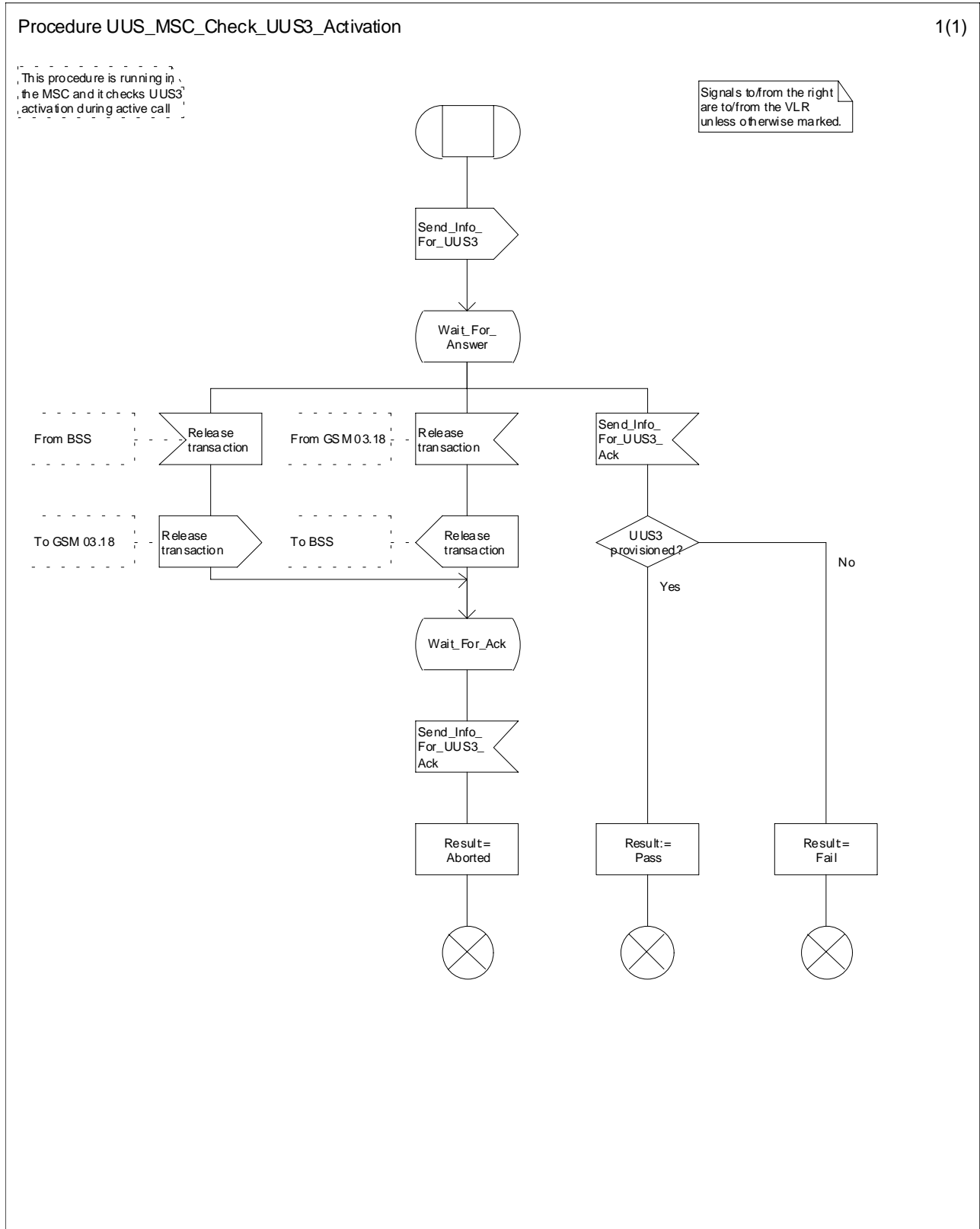
Figure 9.4.1.2: Procedure UUS_MSC_Check_UUS3_Activation
