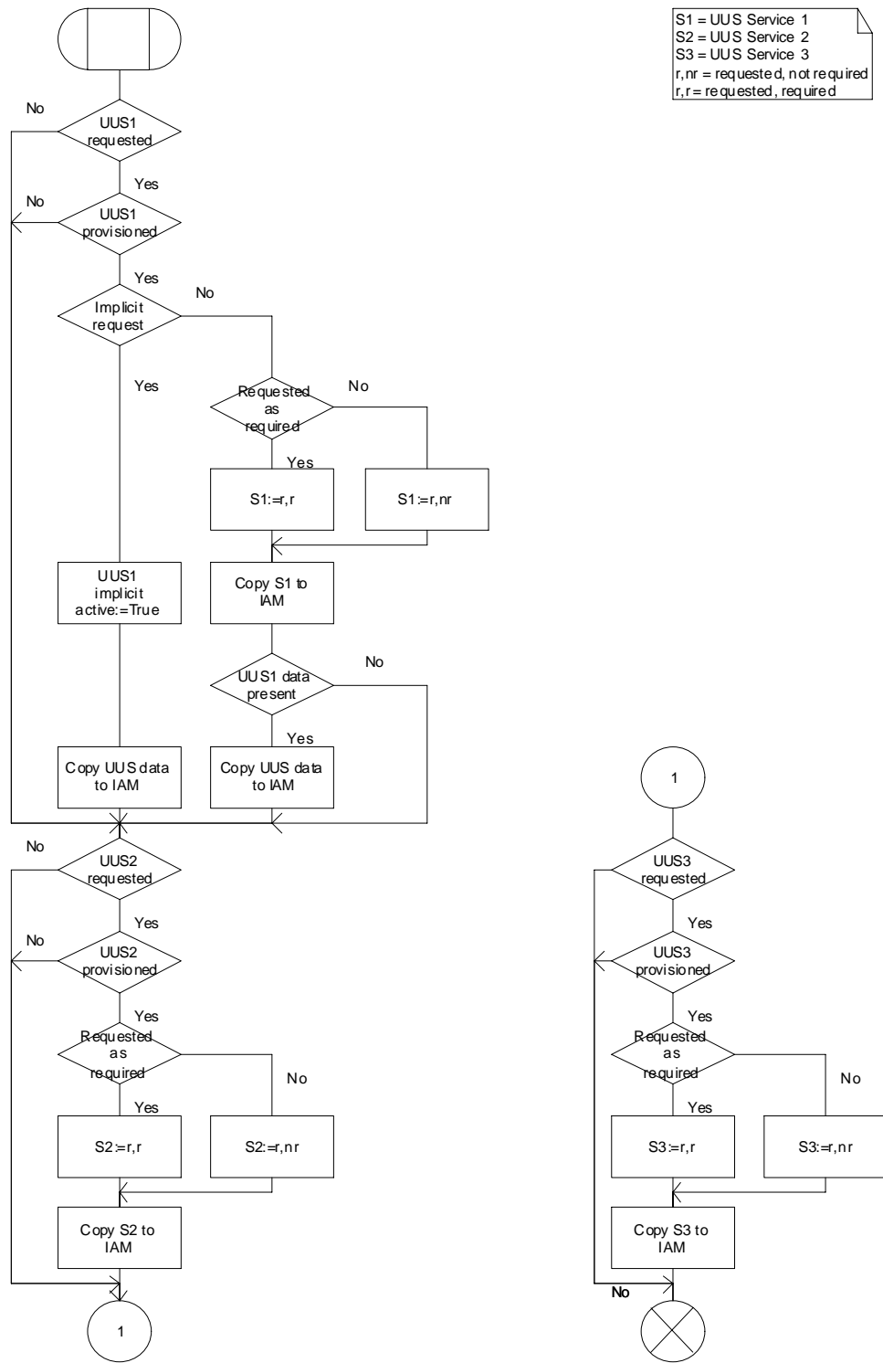
Figure 9.1.1.2: Procedure UUS_OCH_Set_Info_In_IAM
