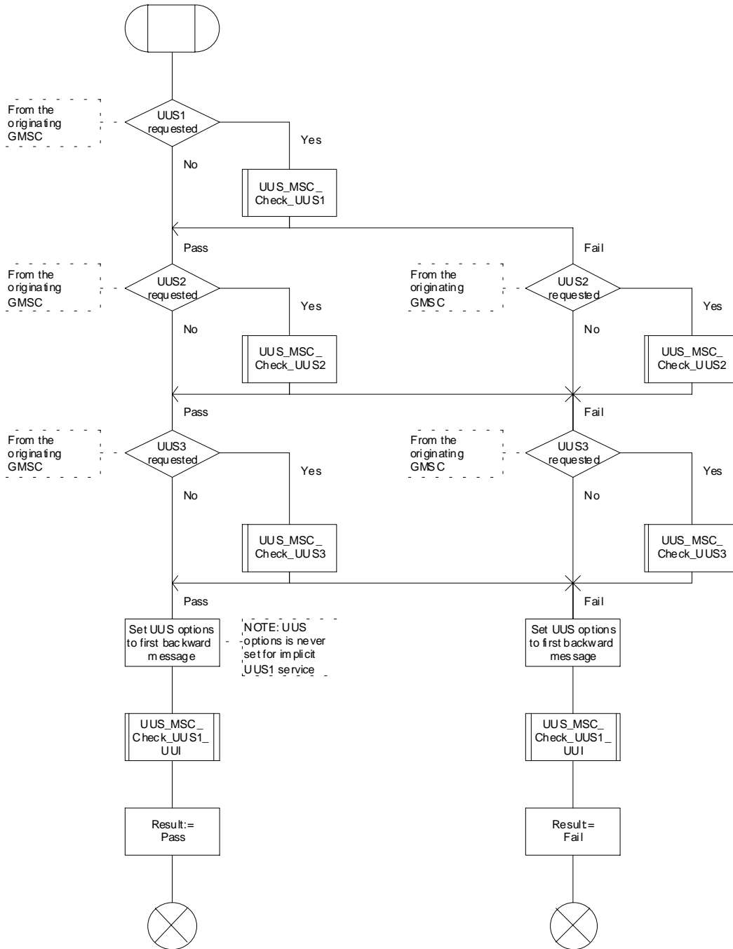
Figure 9.2.2.1: Procedure UUS_ICH_Check_Support
