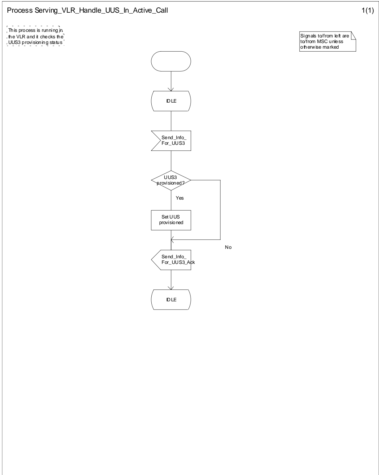
Figure 9.4.2.1: Process Serving_VLR_Handle_UUS_In_Active_Call
