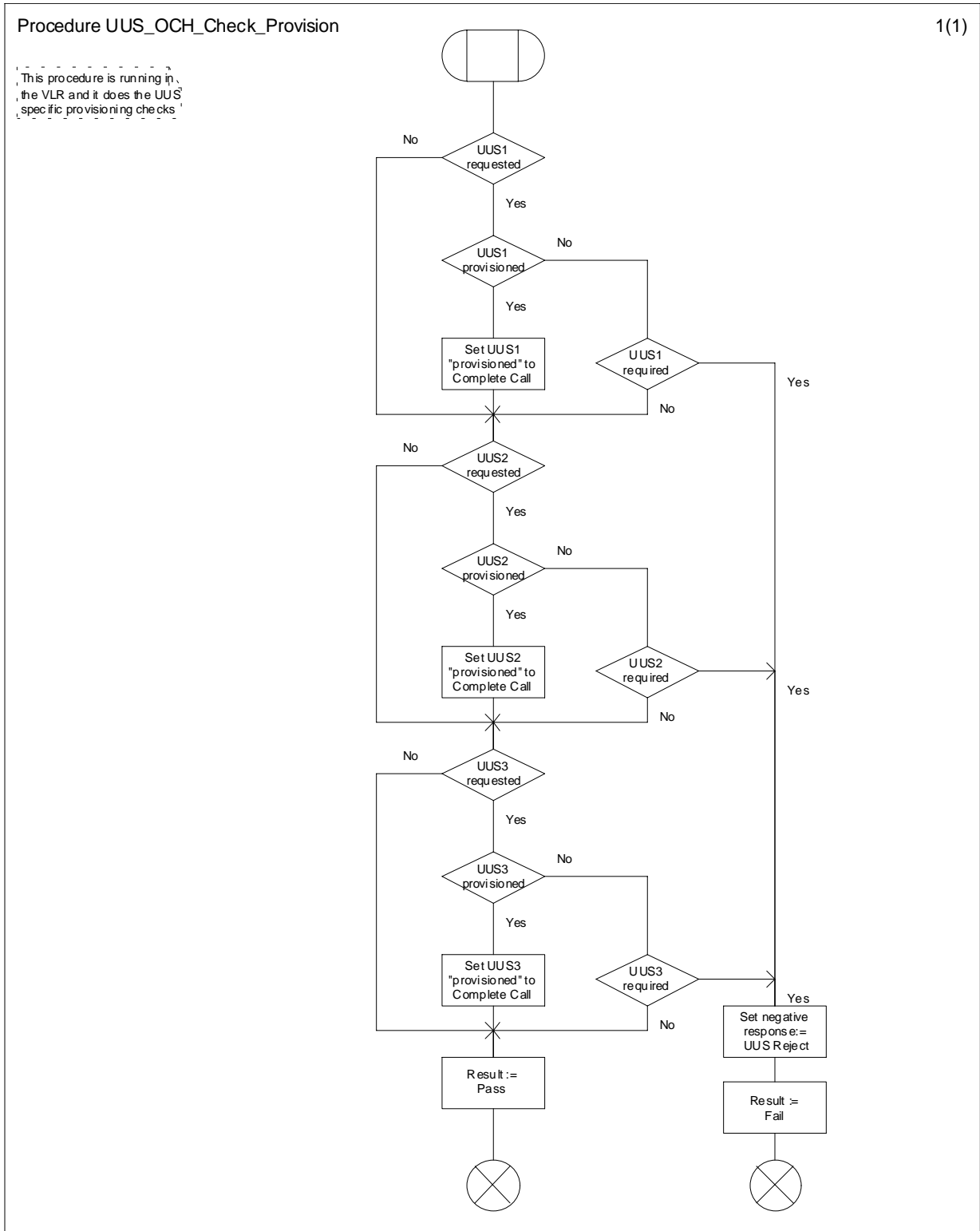
Figure 9.1.2.1: Procedure UUS_OCH_Check_Provision
