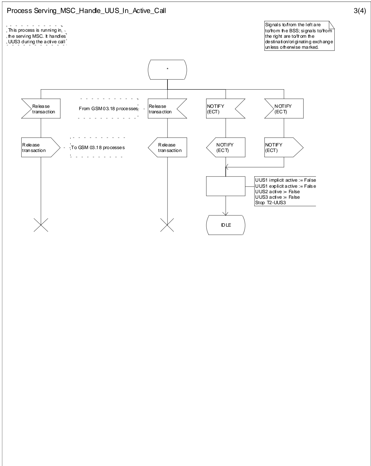
Figure 9.4.1.1: Process Serving_MSC_Handle_UUS_In_Active_Call (sheet 3)
