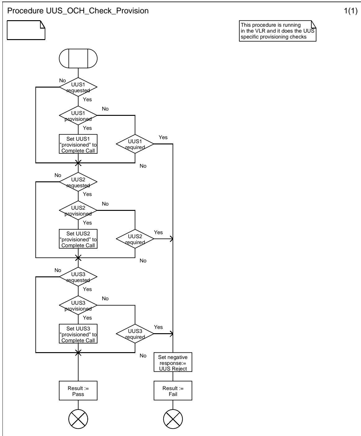
Figure 9.1.2.1: Procedure UUS_OCH_Check_Provision
