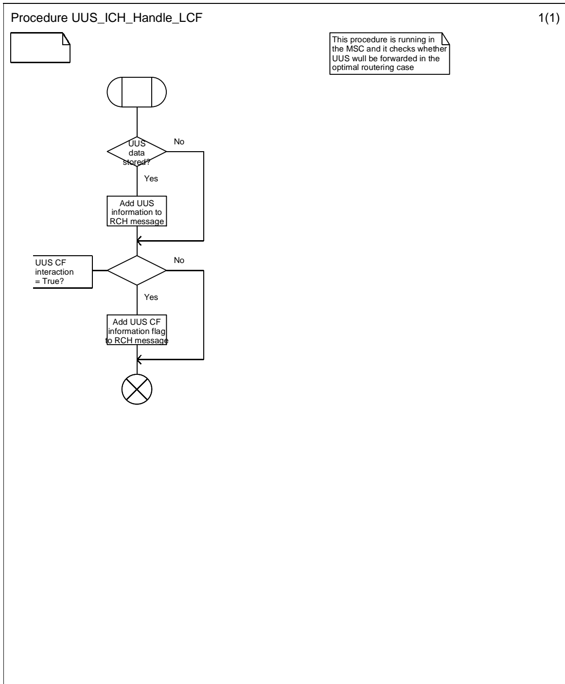
Figure 9.2.2.3: Procedure UUS_ICH_Handle_LCF
