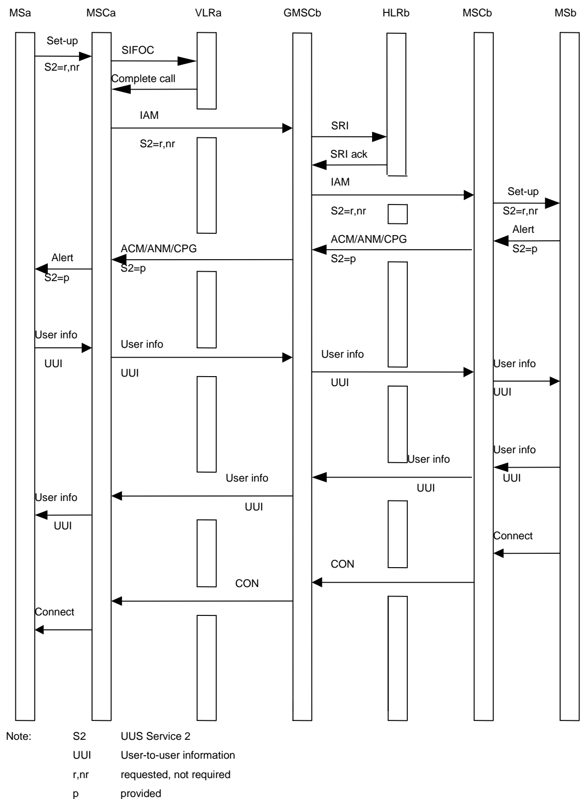
Figure 5.2.2.1: Information flow for UUS2 explicit request (mobile to mobile call)
