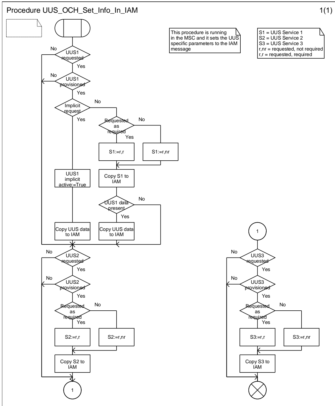
Figure 9.1.1.2: Procedure UUS_OCH_Set_Info_In_IAM
