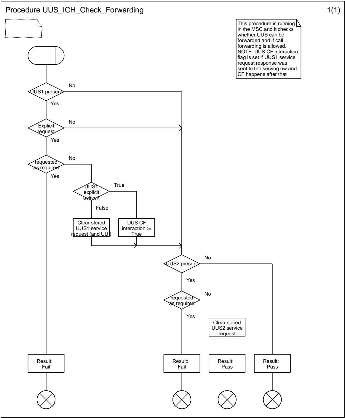
Figure 9.2.2.2: Procedure UUS_ICH_Check_Forwarding
