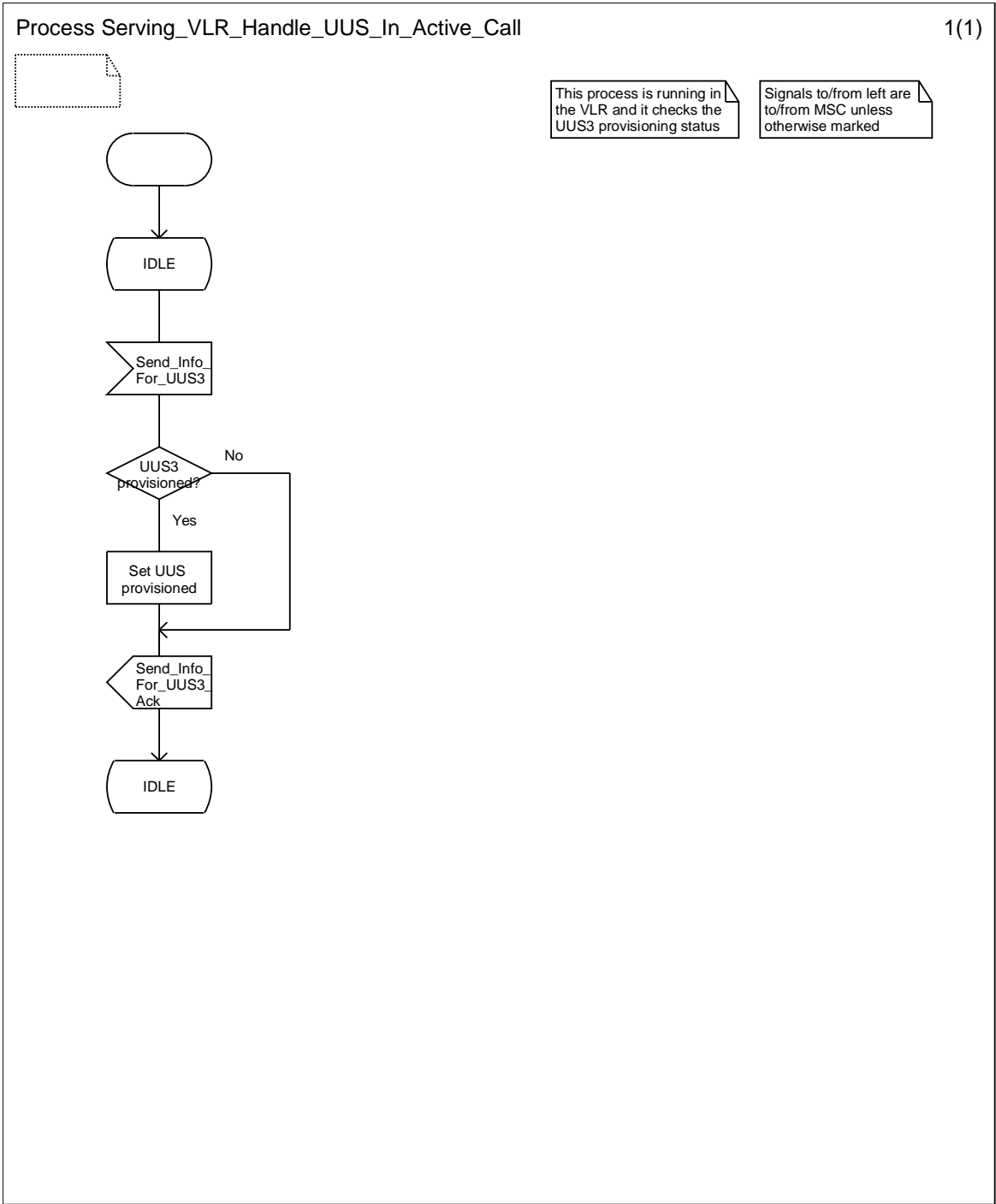
Figure 9.4.2.1: Process Serving_VLR_Handle_UUS_In_Active_Call
