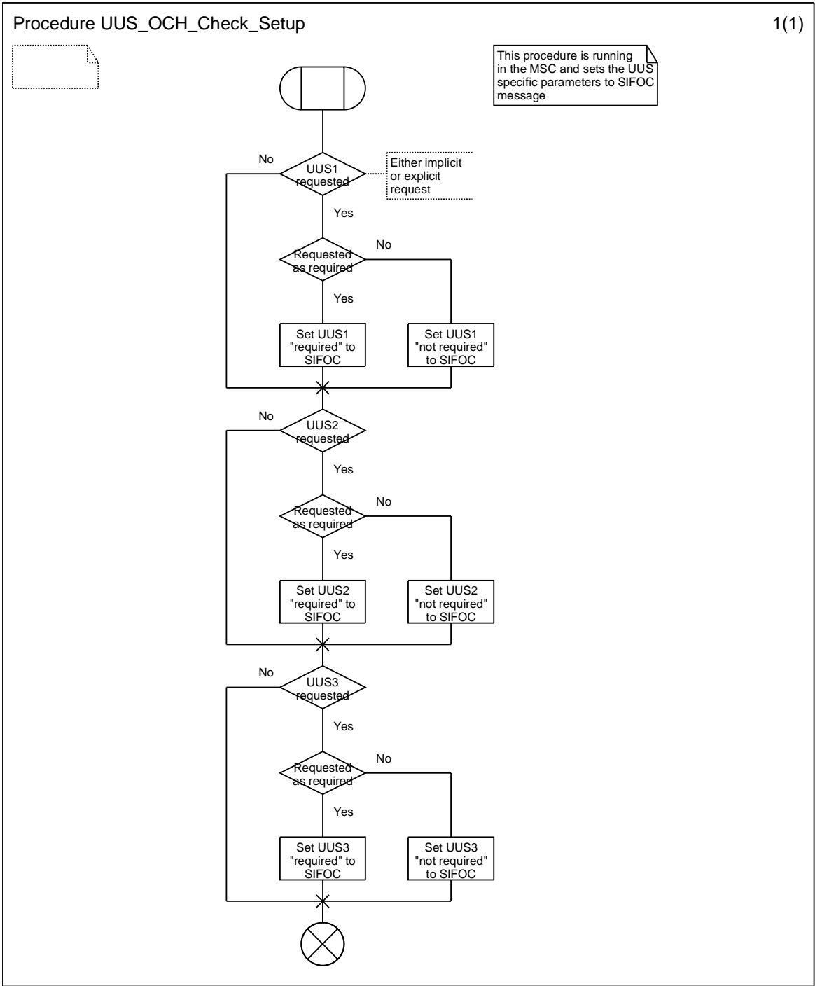
Figure 9.1.1.1: Procedure UUS_OCH_Check_Setup
