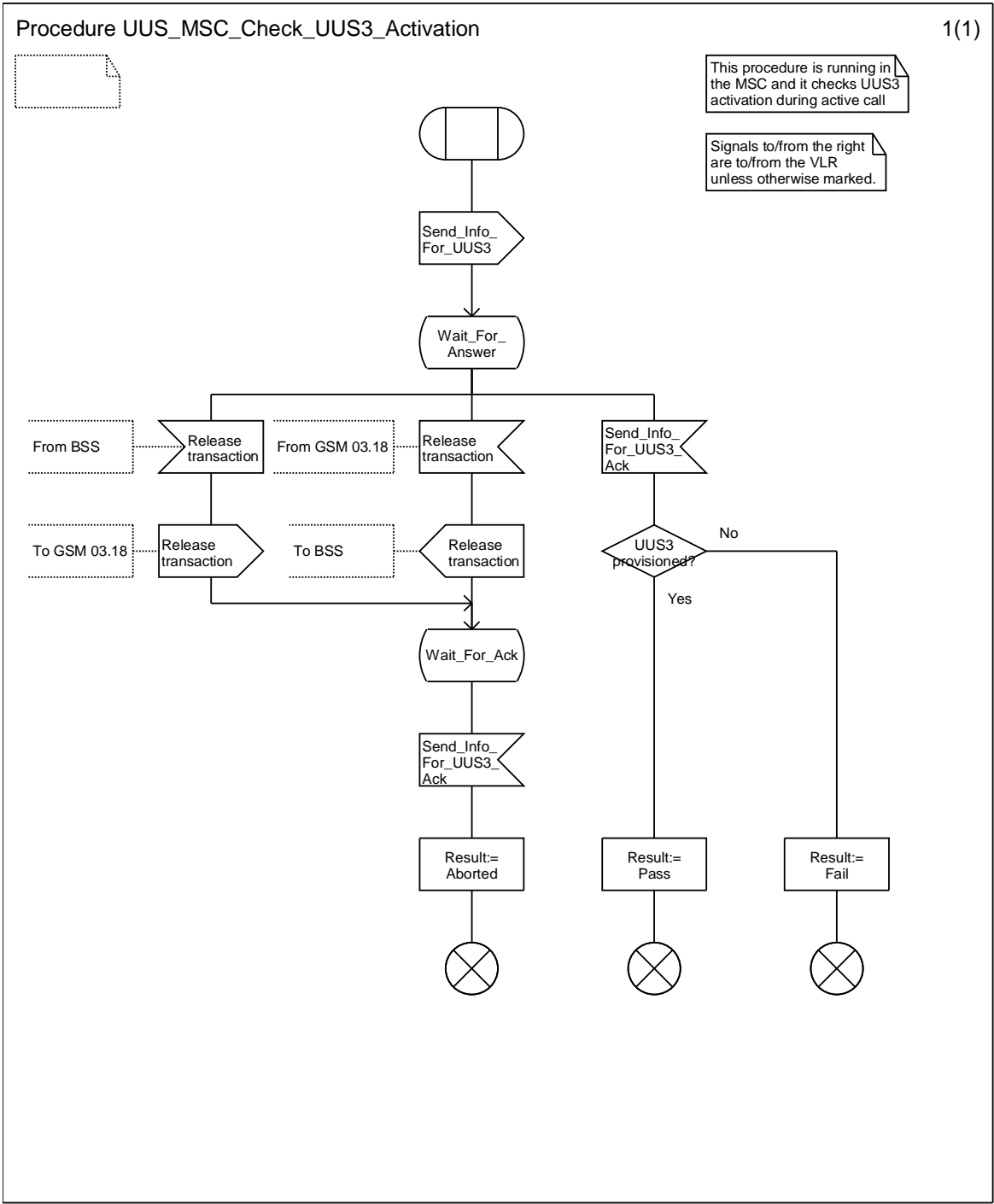
Figure 9.4.1.2: Procedure UUS_MSC_Check_UUS3_Activation
