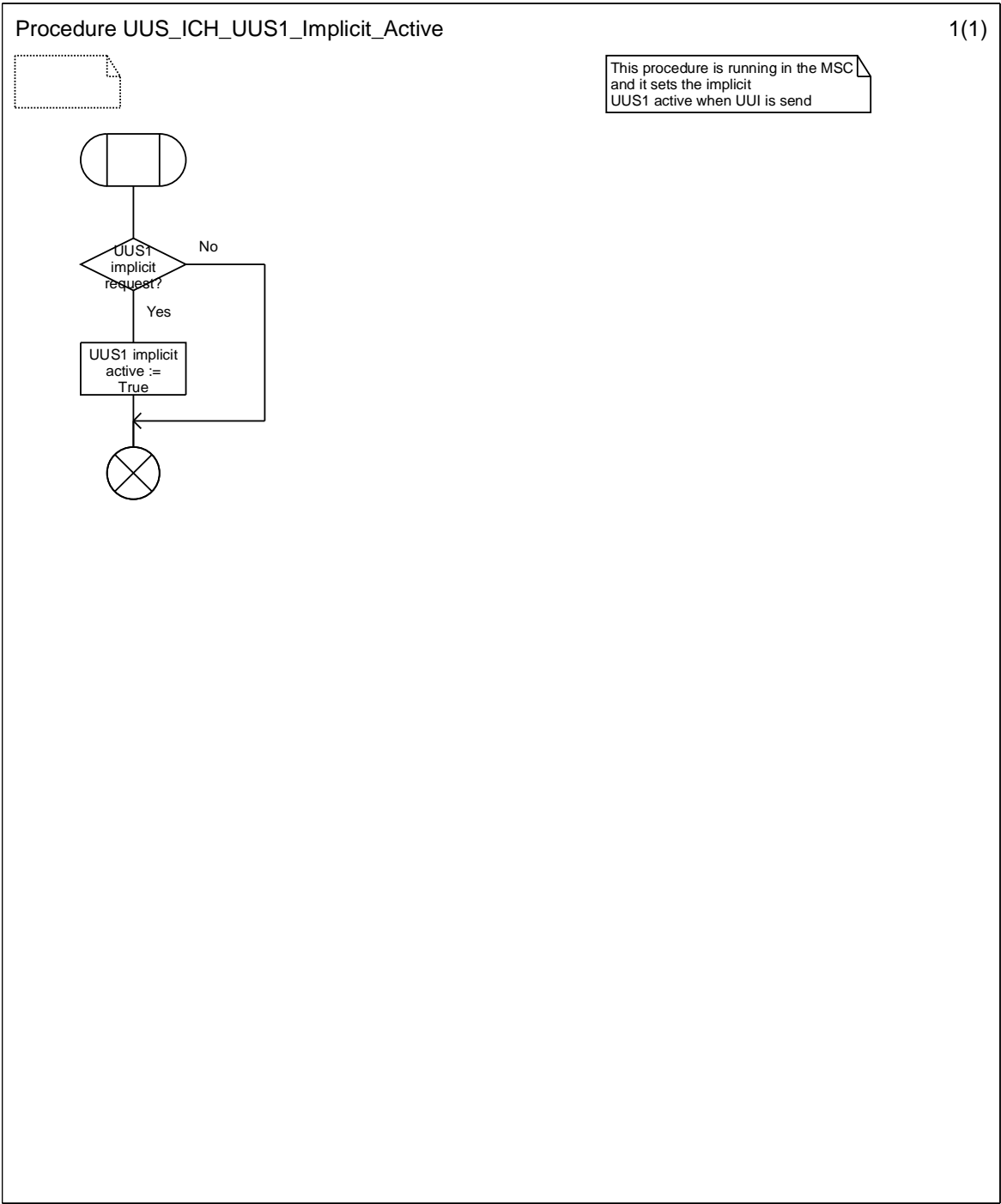
Figure 9.2.2.5: Procedure UUS_ICH_UUS1_Implicit_Active
