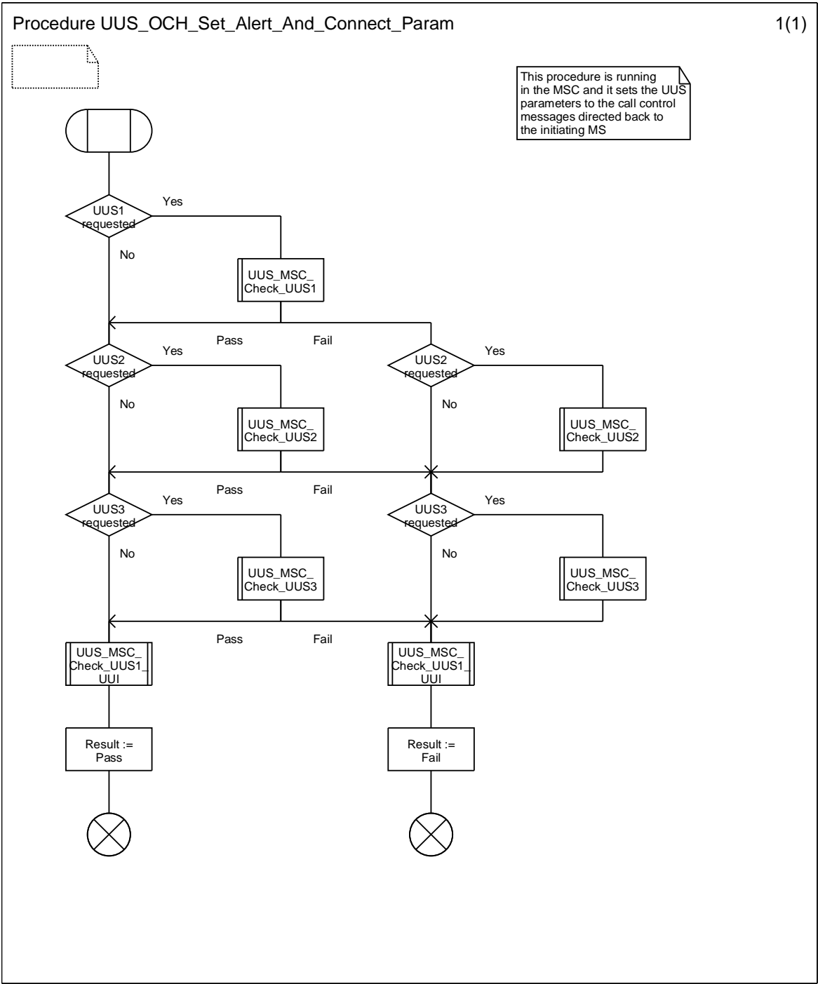
Figure 9.1.1.3: Procedure UUS_OCH_Set_Alert_And_Connect_Param
