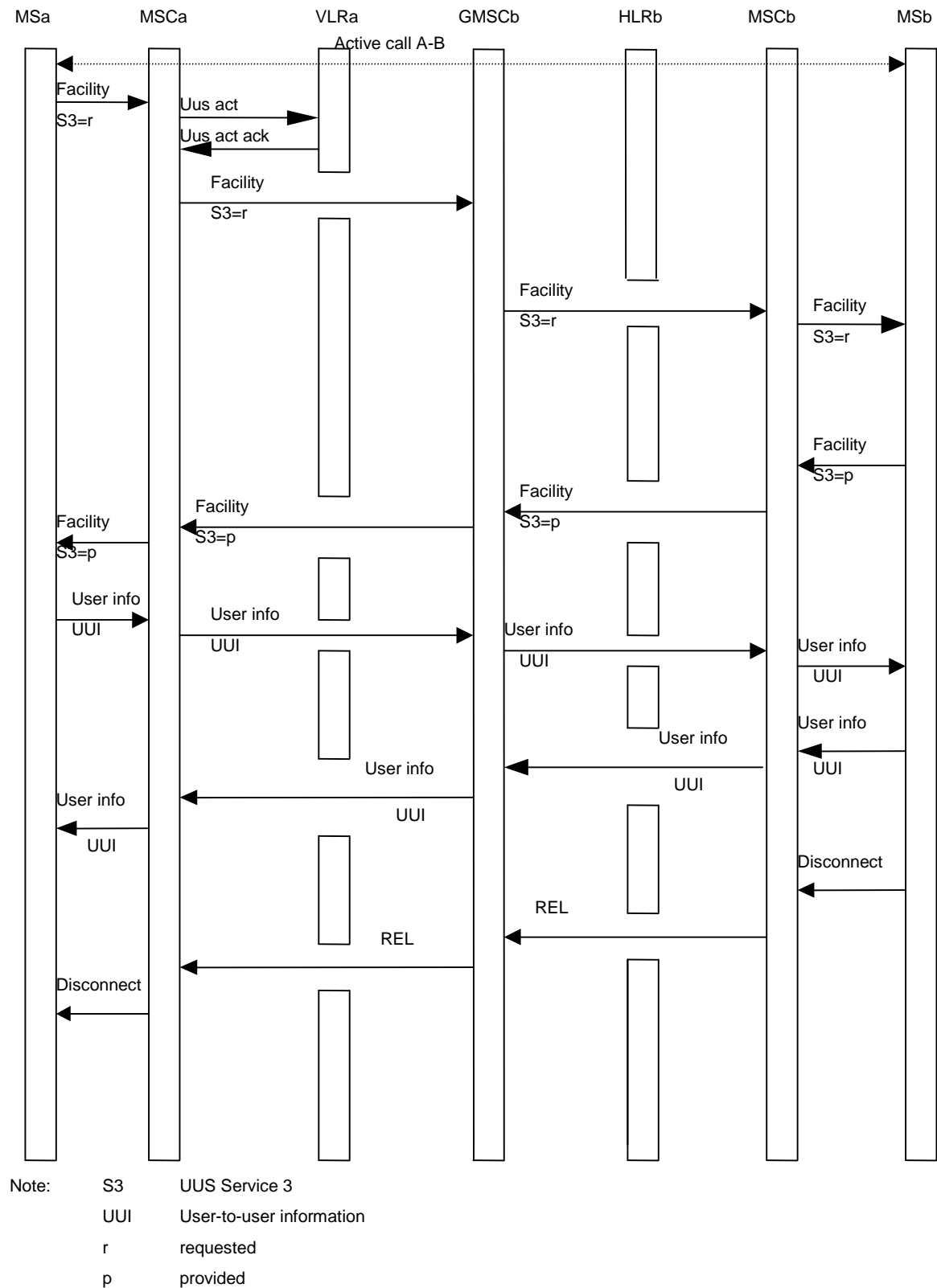
Figure 5.2.3.2.2: Information flow for UUS3 explicit request during active call (mobile to mobile call)
