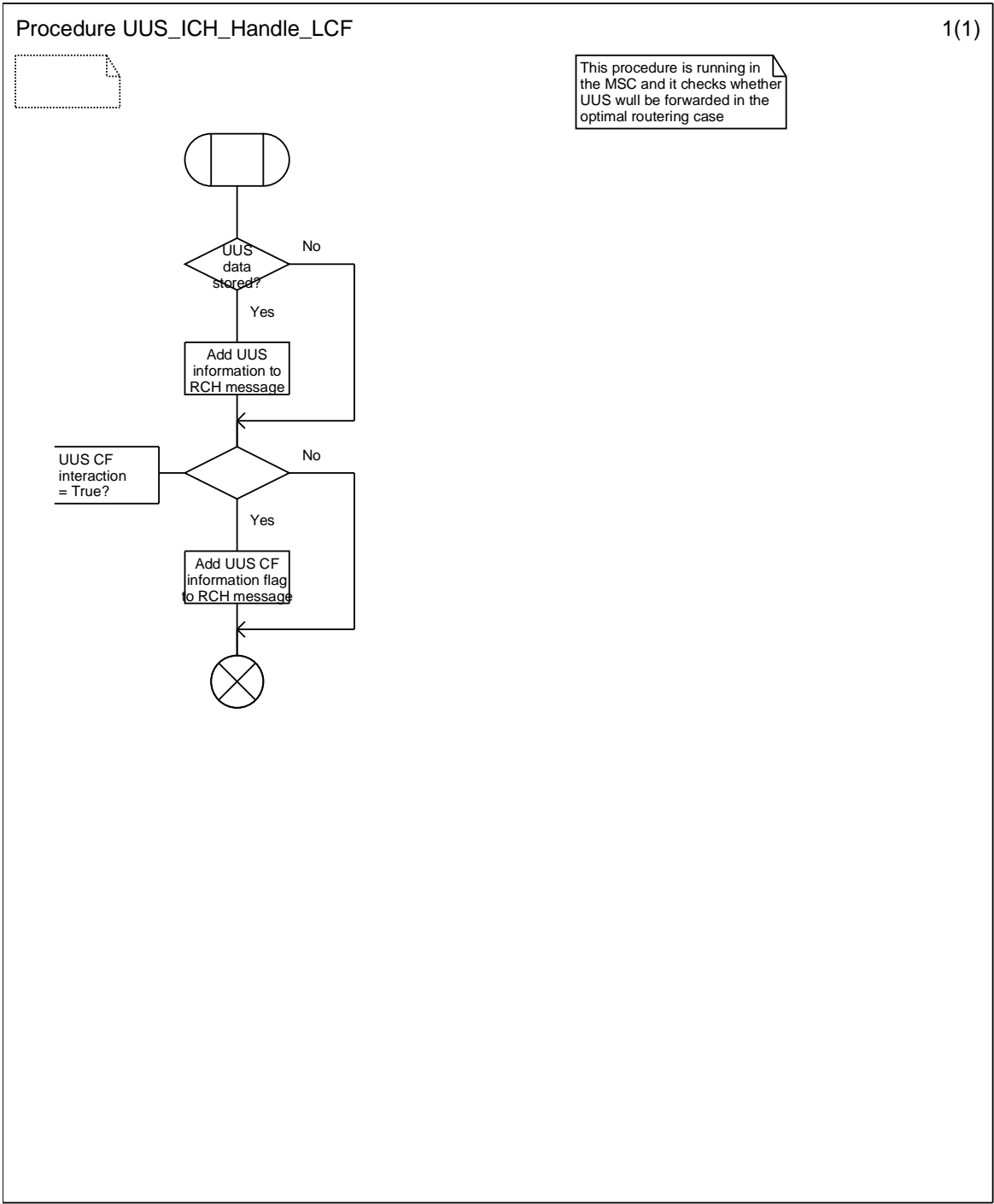
Figure 9.2.2.3: Procedure UUS_ICH_Handle_LCF
