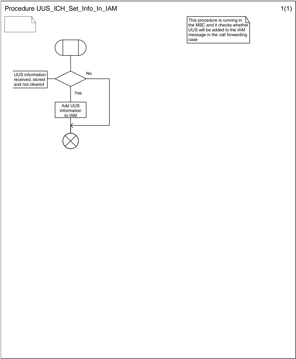
Figure 9.2.2.4: Procedure UUS_ICH_Set_Info_In_IAM
