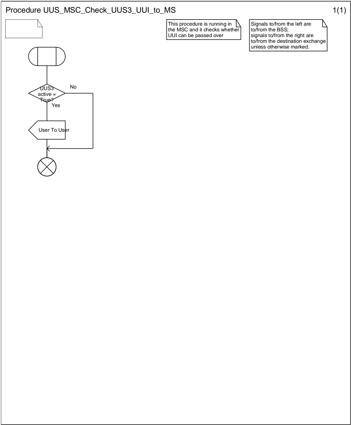
Figure 9.3.4: Procedure UUS_MSC_Check_UUS3_UUI_to_MS
