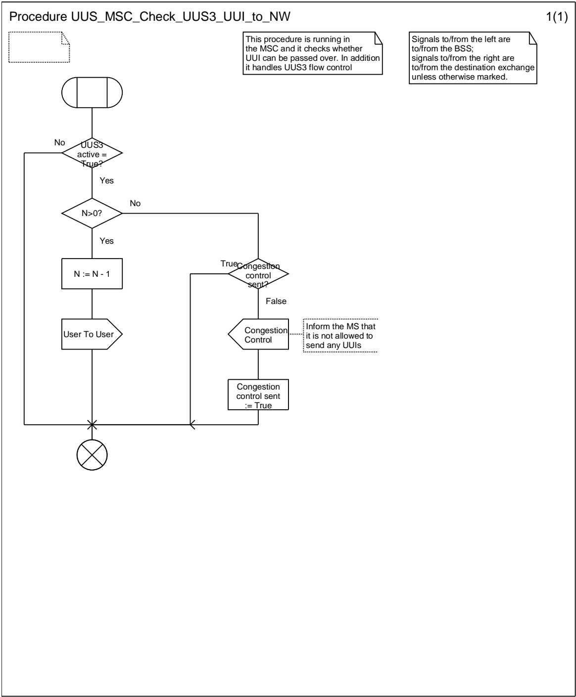
Figure 9.3.5: Procedure UUS_MSC_Check_UUS3_UUI_to_NW
