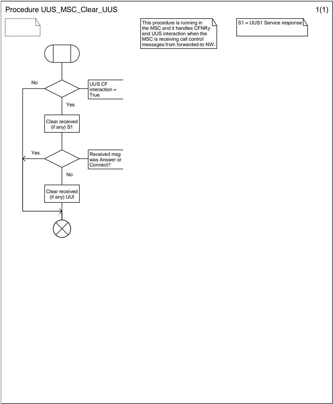
Figure 9.3.6: Procedure UUS_MSC_Clear_UUS
