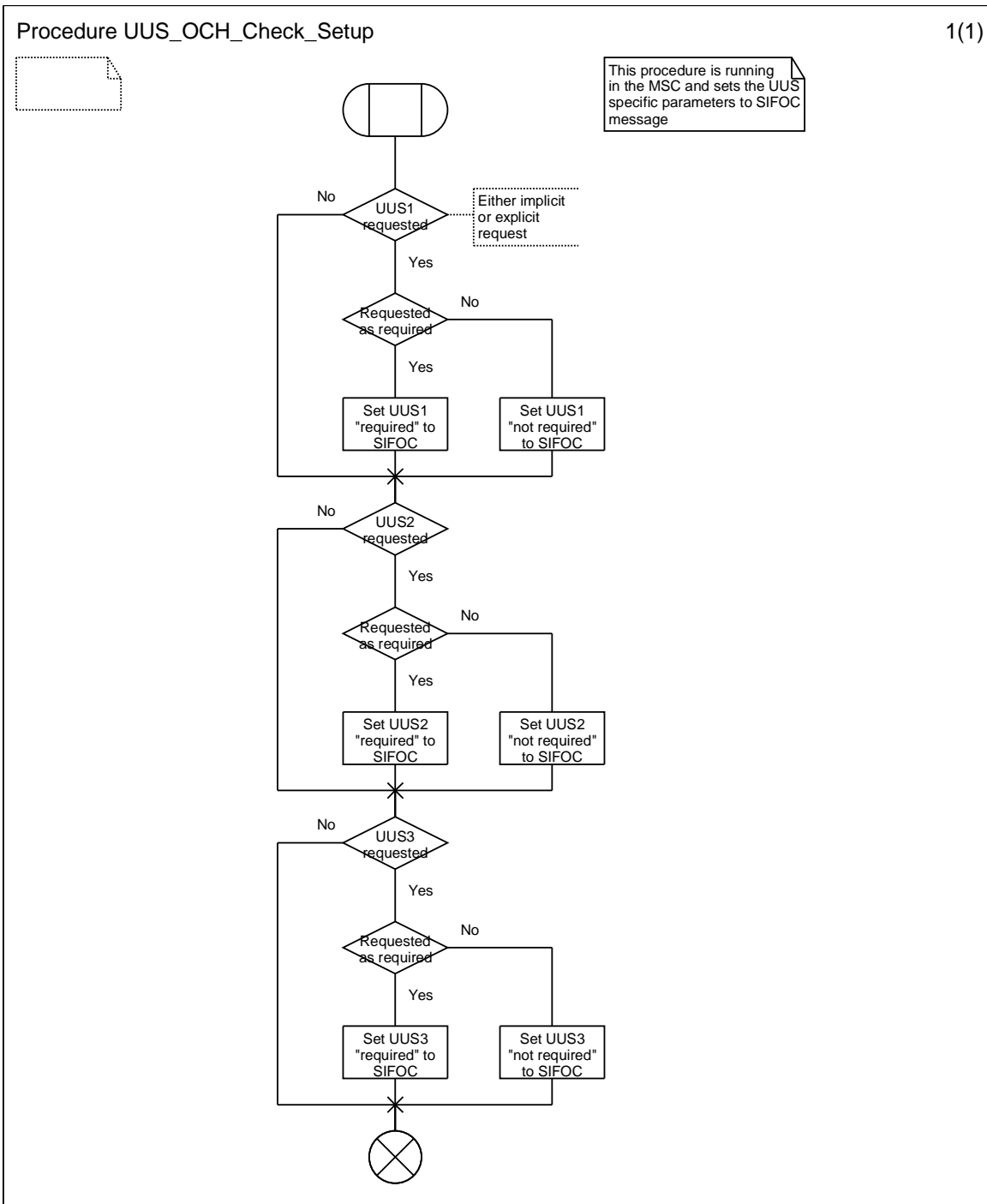
Figure 9.1.1.1: Procedure UUS_OCH_Check_Setup
