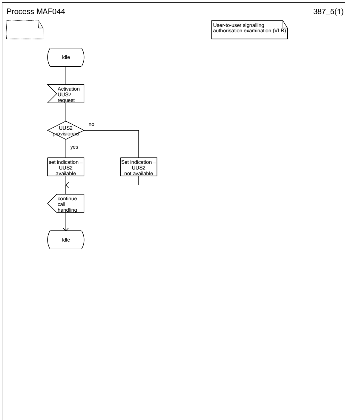
Figure 5.2.2.2: MAF044
