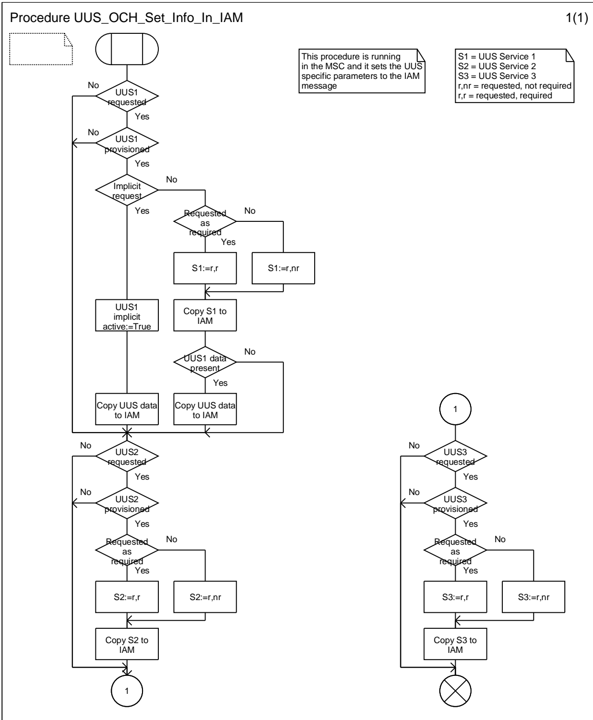
Figure 9.1.1.2: Procedure UUS_OCH_Set_Info_In_IAM
