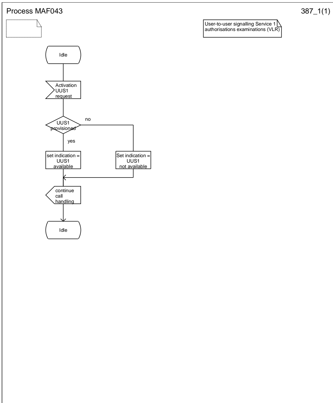
Figure 5.2.1.2: MAF043
