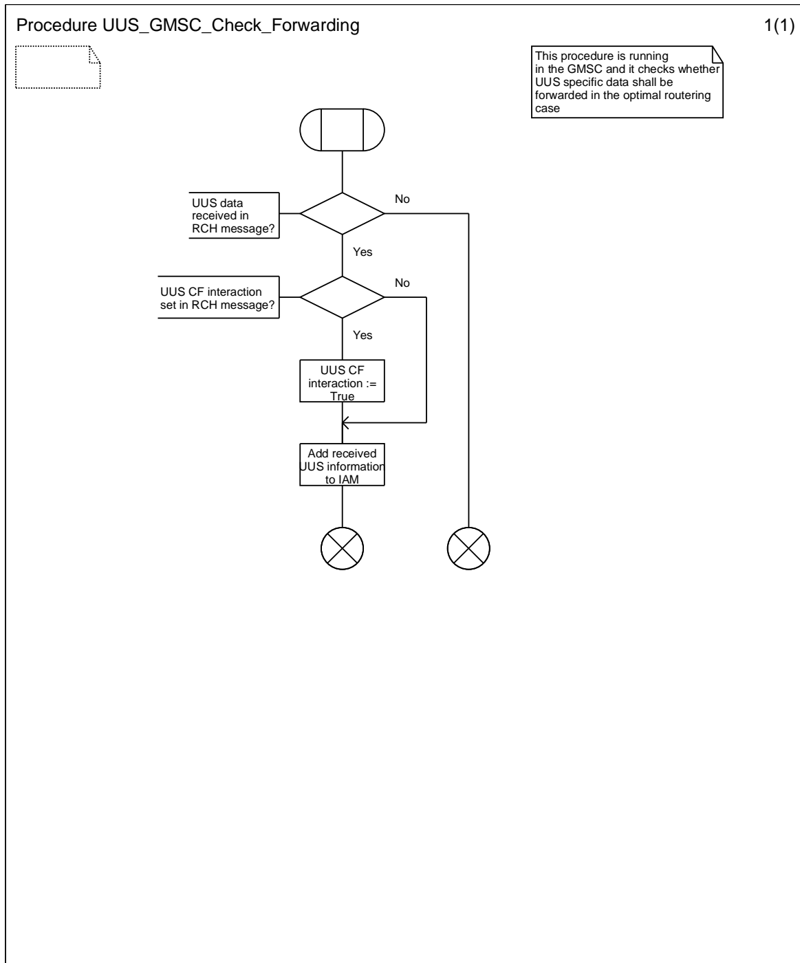
Figure 9.2.1.1: Procedure UUS_GMSC_Check_Forwarding
