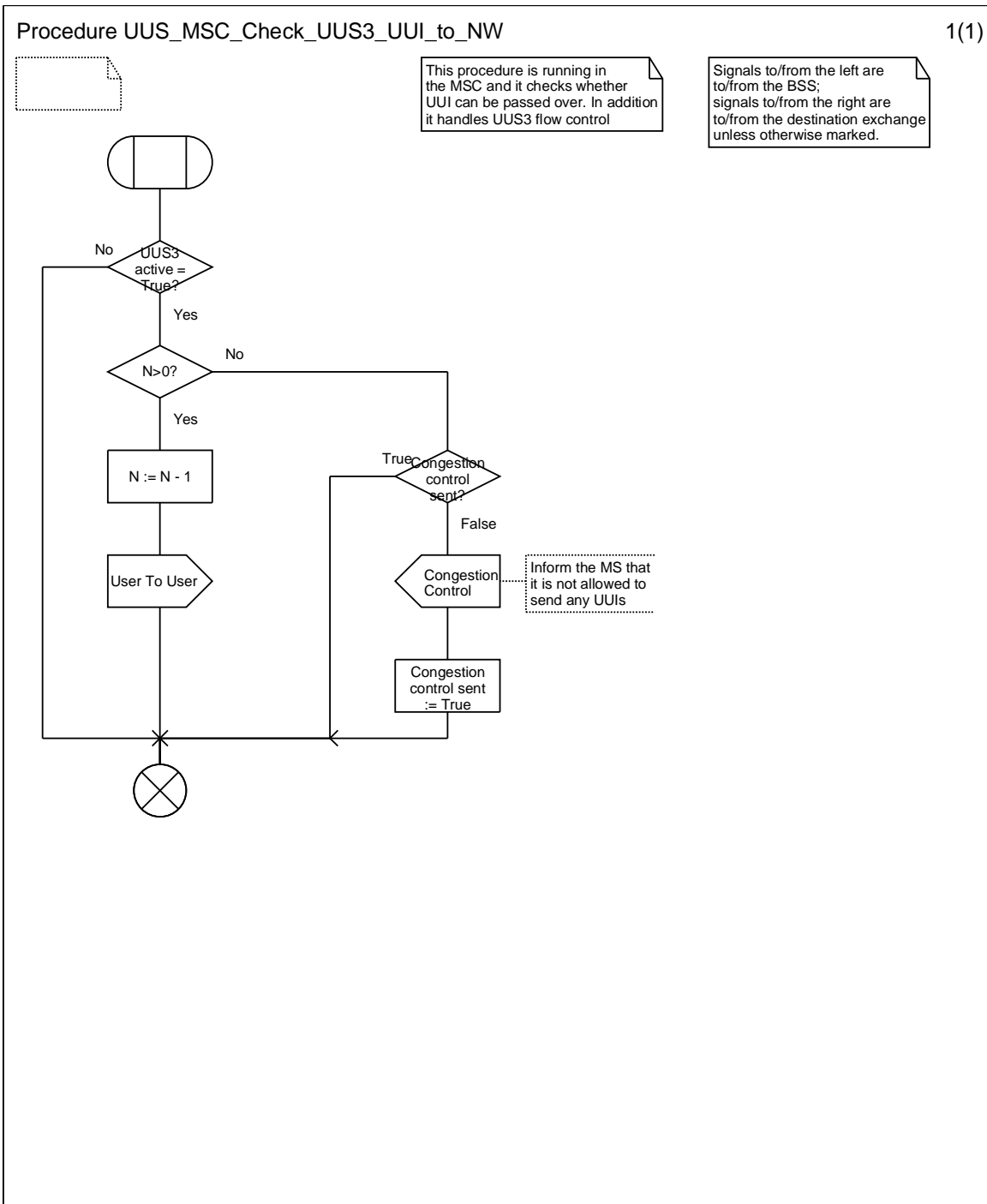
Figure 9.3.5: Procedure UUS_MSC_Check_UUS3_UUI_to_NW
