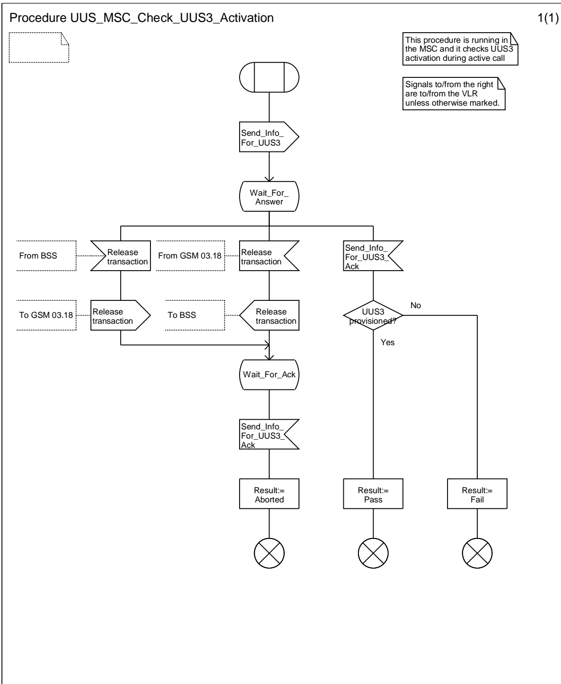
Figure 9.4.1.2: Procedure UUS_MSC_Check_UUS3_Activation
