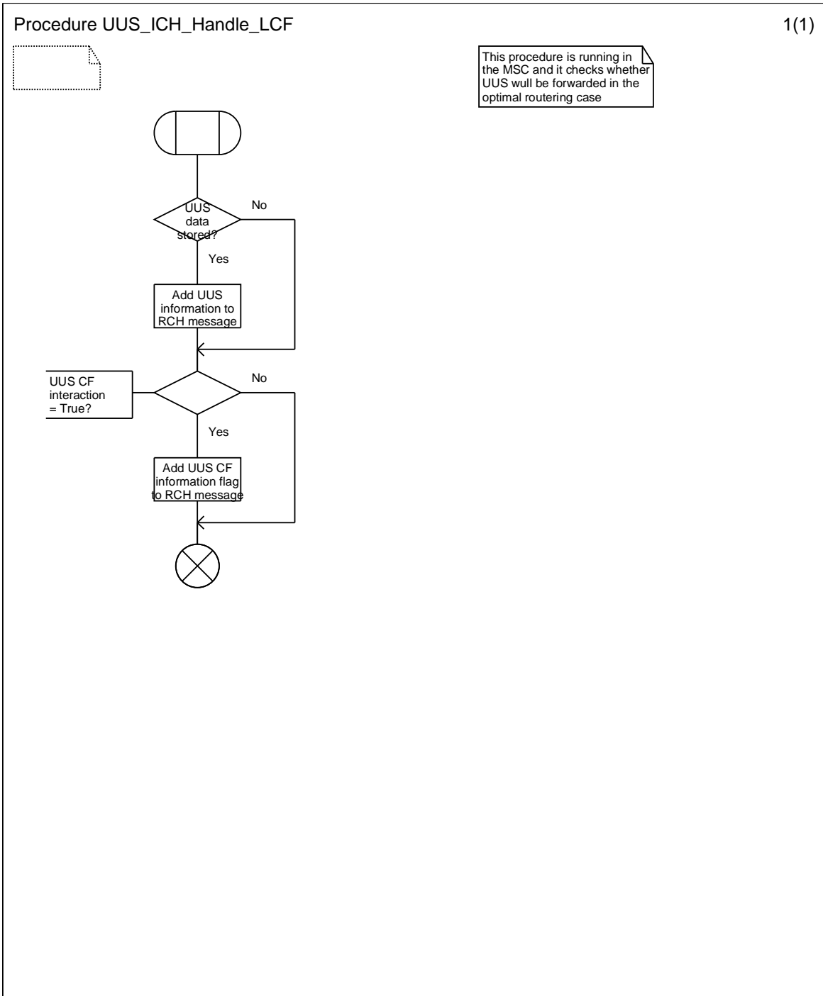
Figure 9.2.2.3: Procedure UUS_ICH_Handle_LCF
