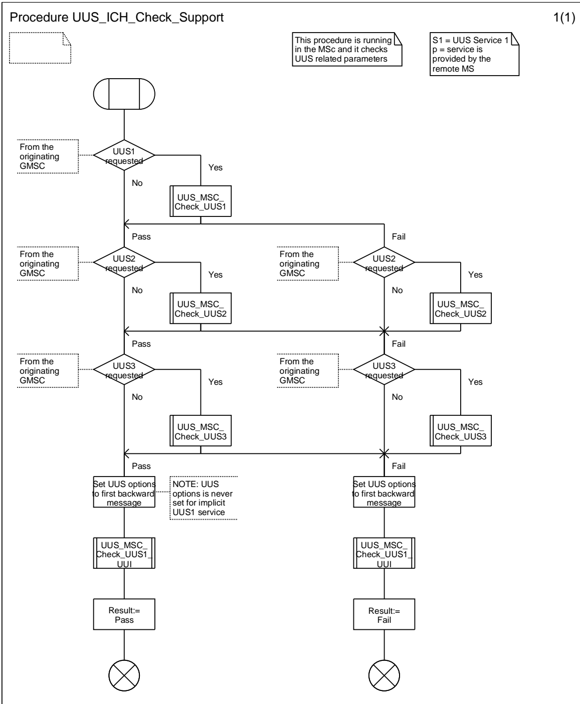
Figure 9.2.2.1: Procedure UUS_ICH_Check_Support
