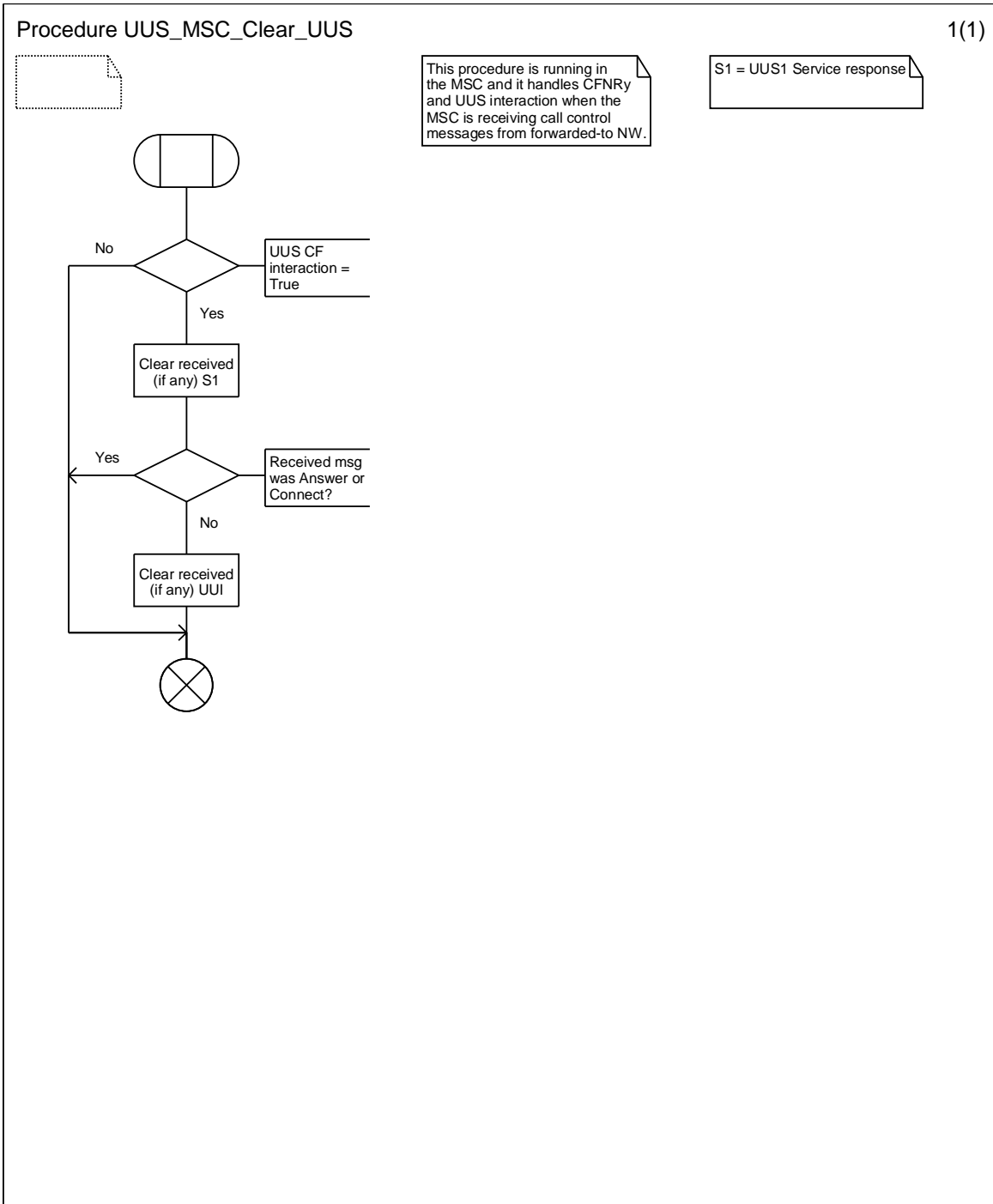
Figure 9.3.6: Procedure UUS_MSC_Clear_UUS
