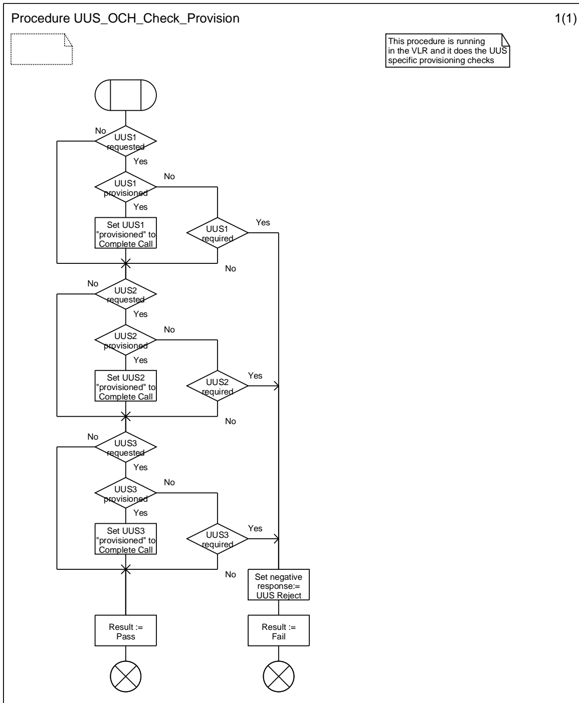
Figure 9.1.2.1: Procedure UUS_OCH_Check_Provision
