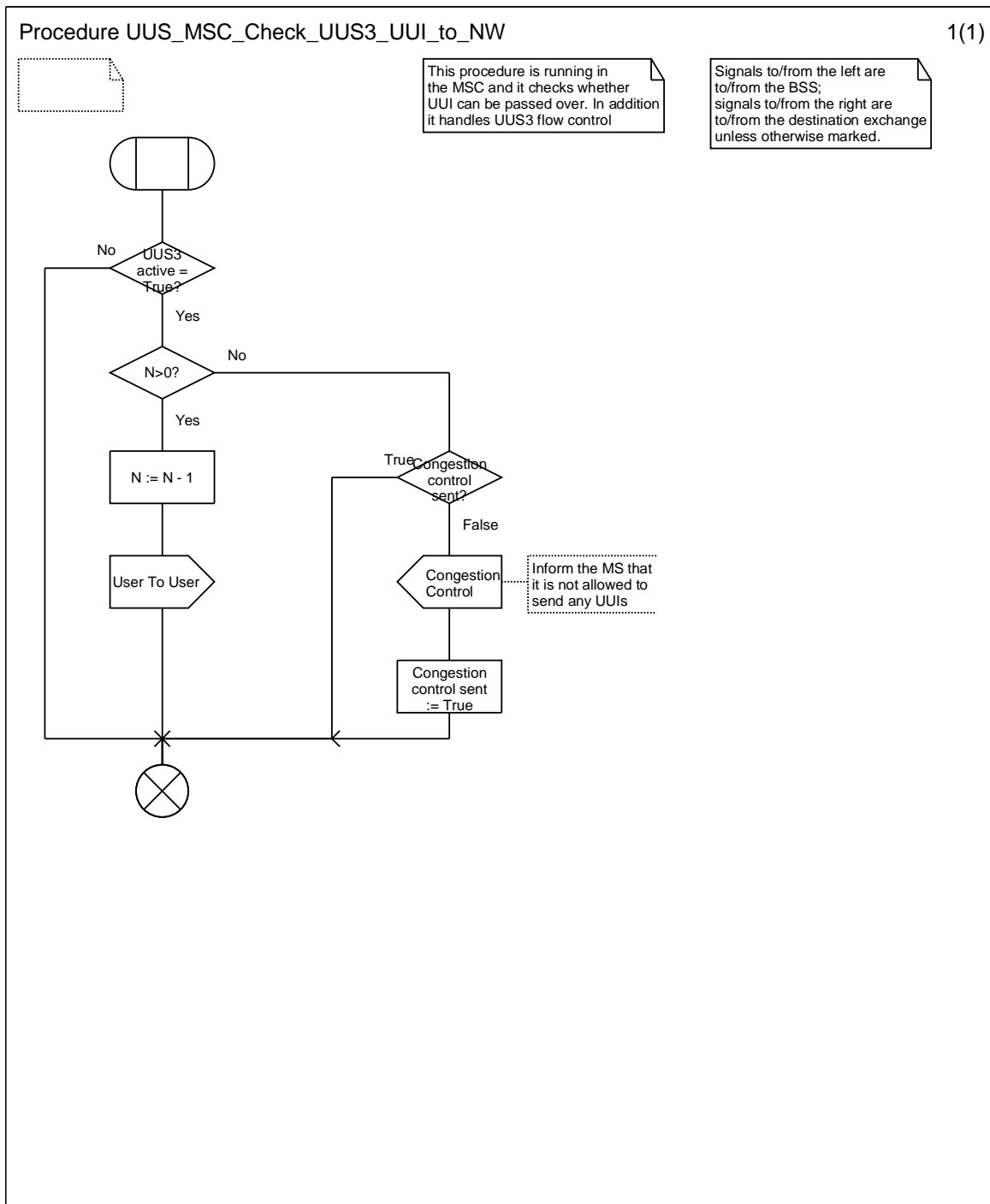
Figure 9.3.5: Procedure UUS_MSC_Check_UUS3_UUI_to_NW
