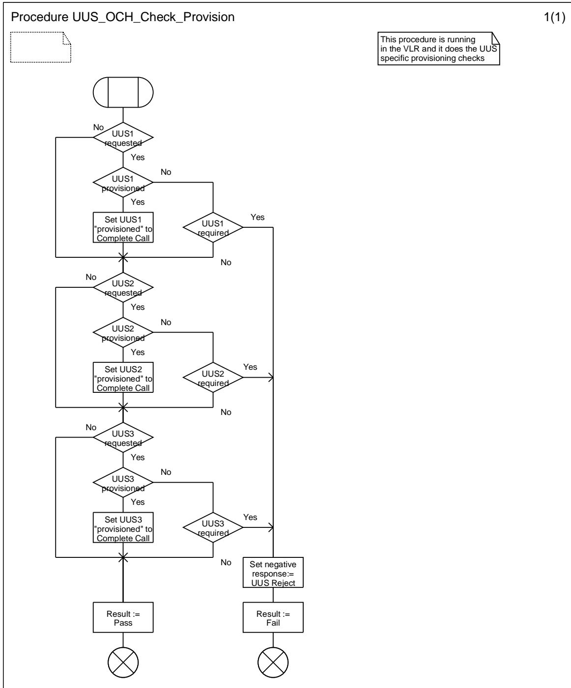
Figure 9.1.2.1: Procedure UUS_OCH_Check_Provision
