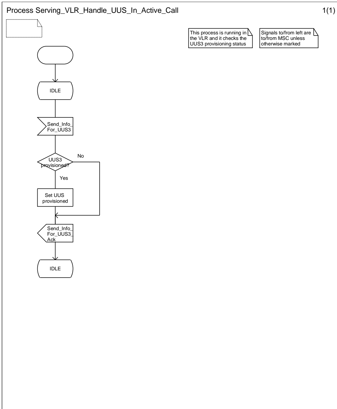
Figure 9.4.2.1: Process Serving_VLR_Handle_UUS_In_Active_Call
