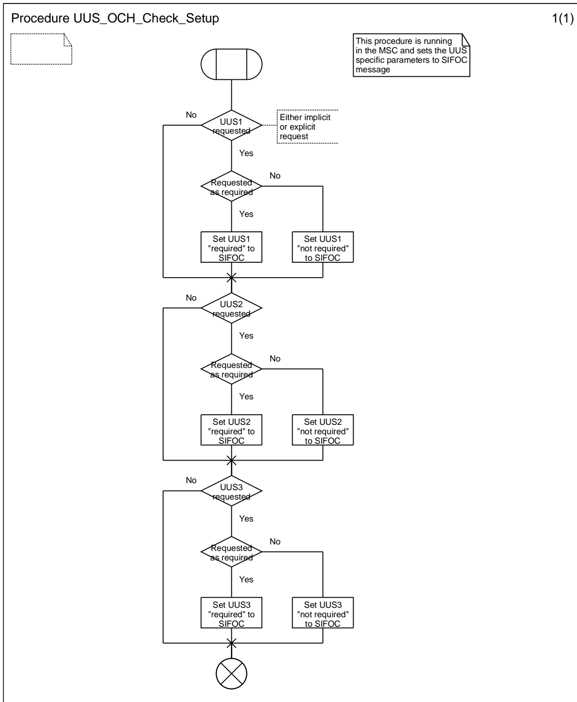
Figure 9.1.1.1: Procedure UUS_OCH_Check_Setup
