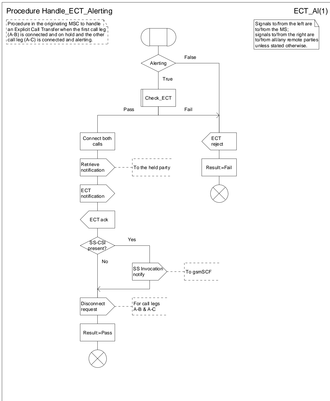
Figure 6: Procedure Handle_ECT_Alerting
