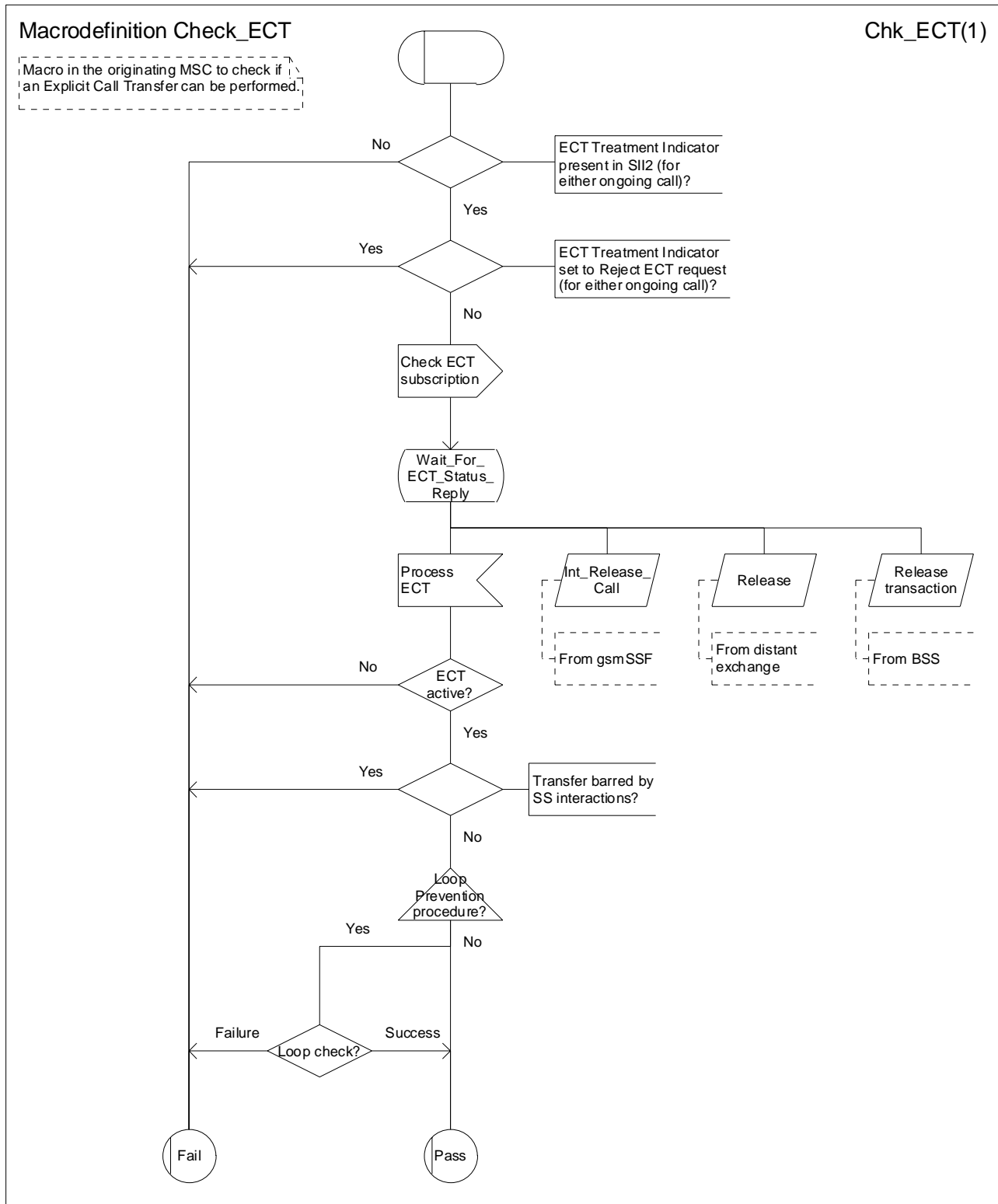
Figure 3: Macro Check_ECT
