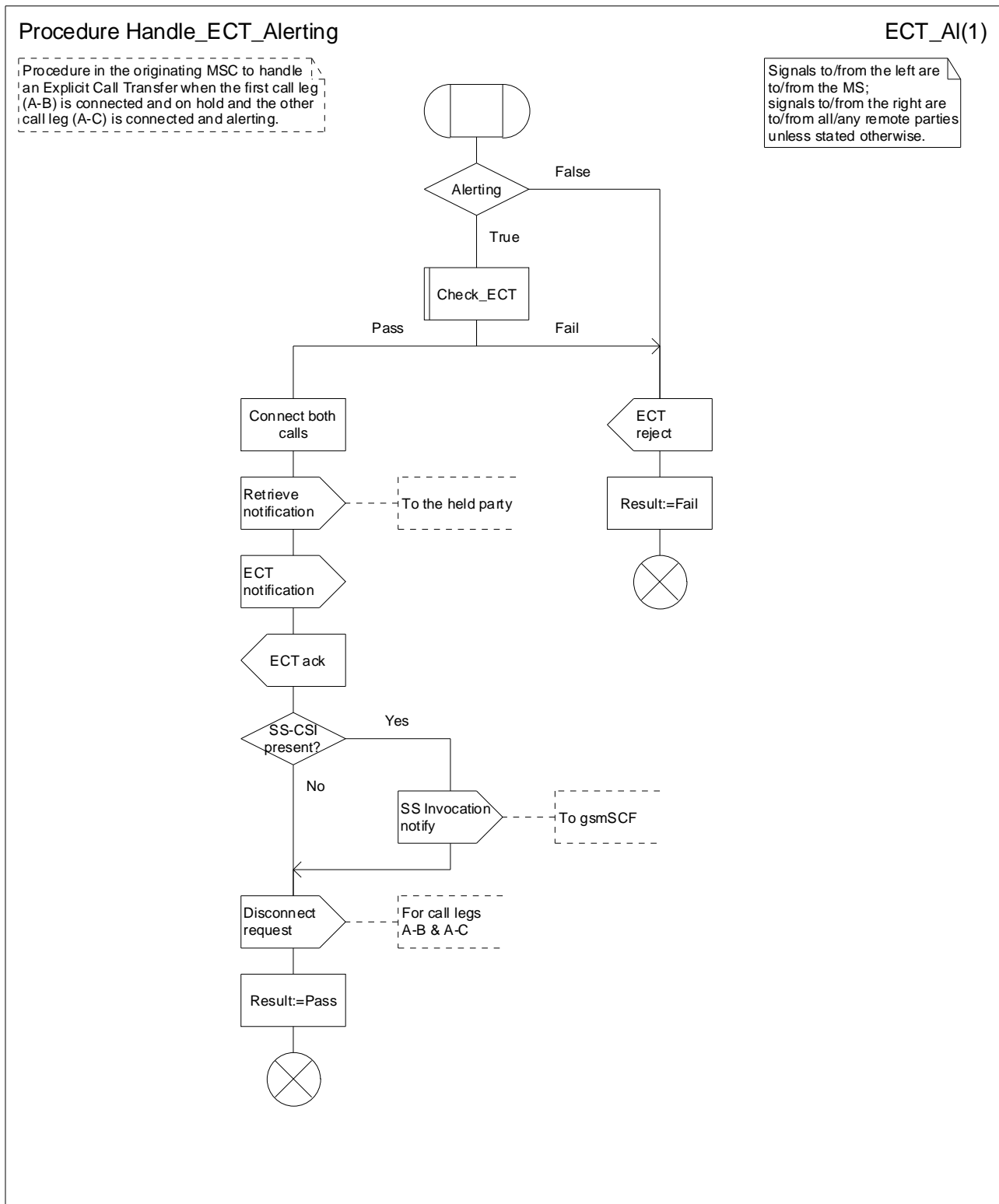
Figure 6: Procedure Handle_ECT_Alerting
