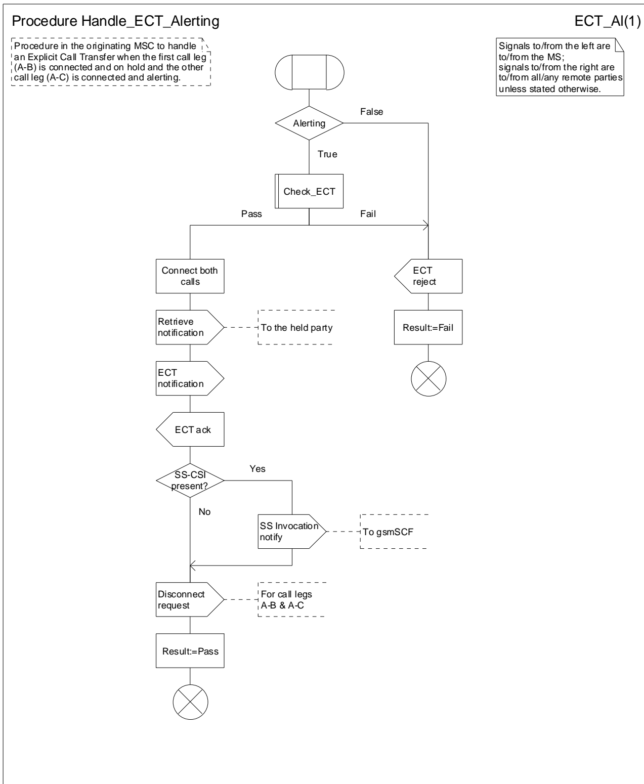
Figure 6: Procedure Handle_ECT_Alerting
