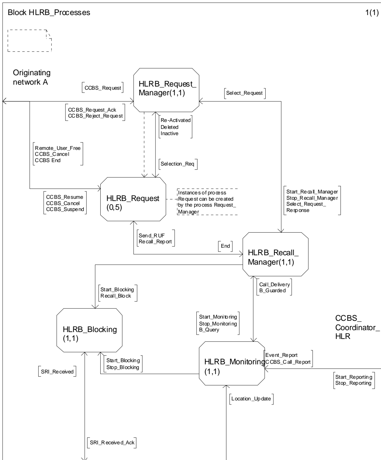
Figure 11.2.2.1: HLRB_Processes
