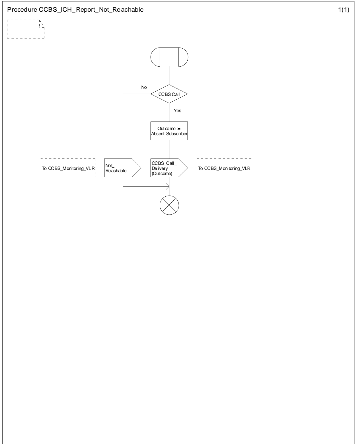
Figure 11.2.3.6: Procedure CCBS_ICH_Report_Not_Reachable
