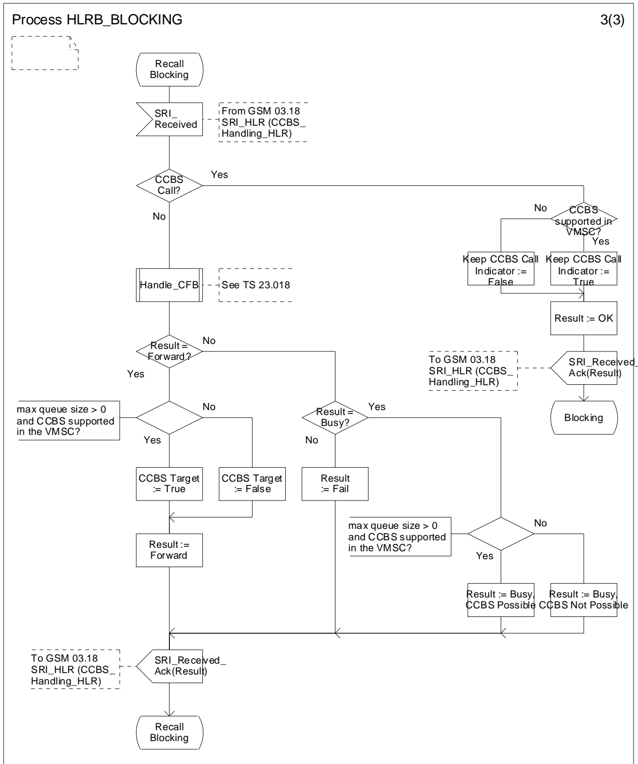
Figure 11.2.2.6: Process HLRB_BLOCKING (sheet 3 of 3)
