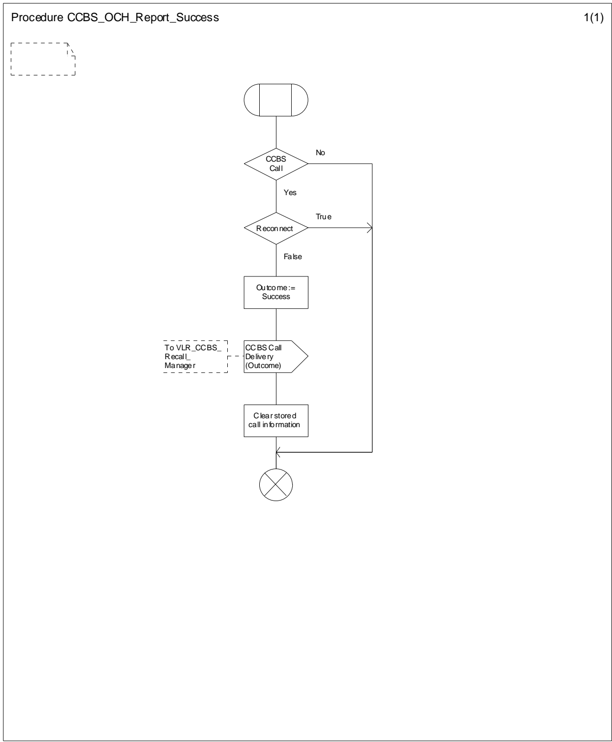
Figure 11.1.1.11: Procedure CCBS_OCH_Report_Success
