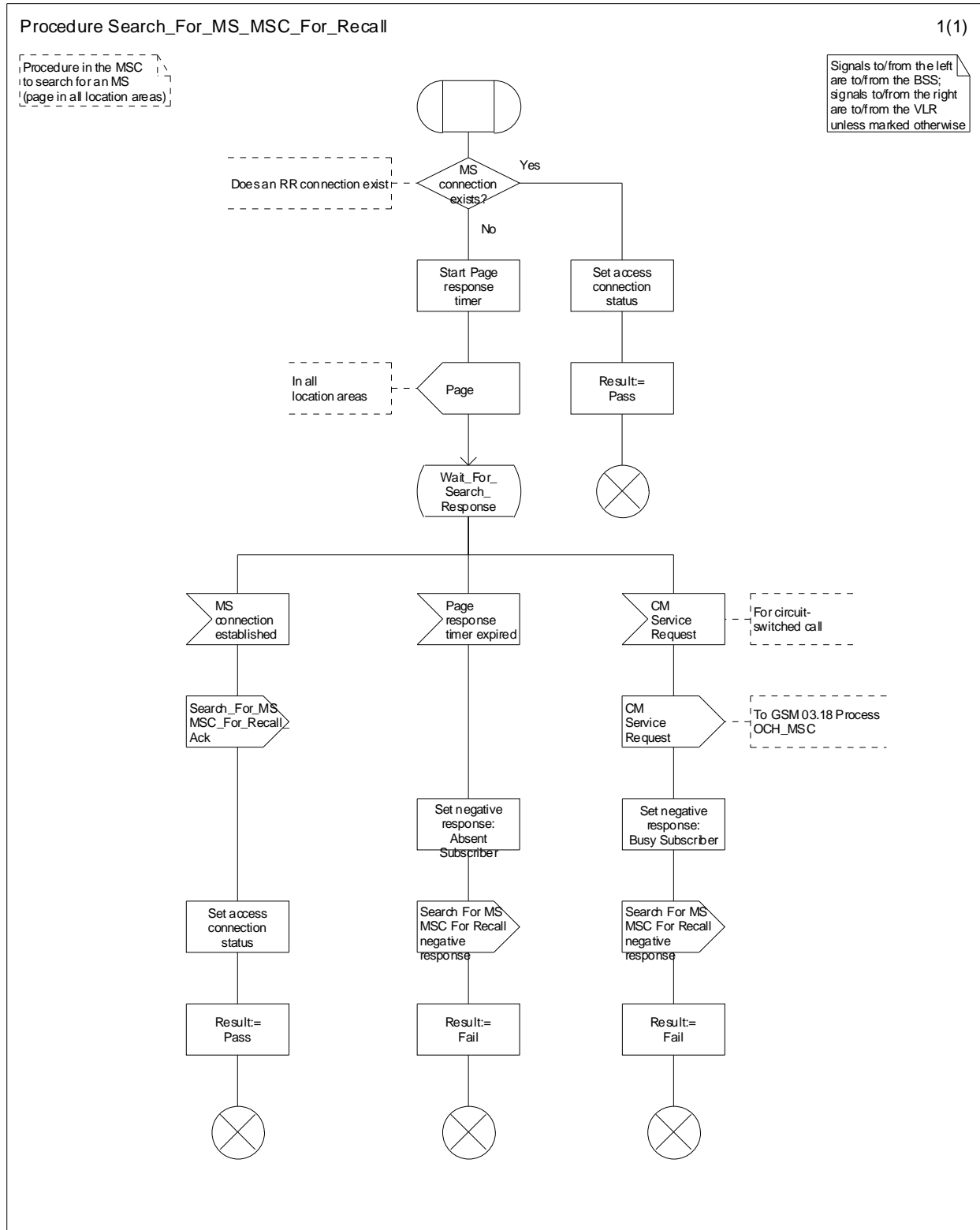
Figure 11.1.1.8: Procedure Search_For_MS_MSC_For_Recall
