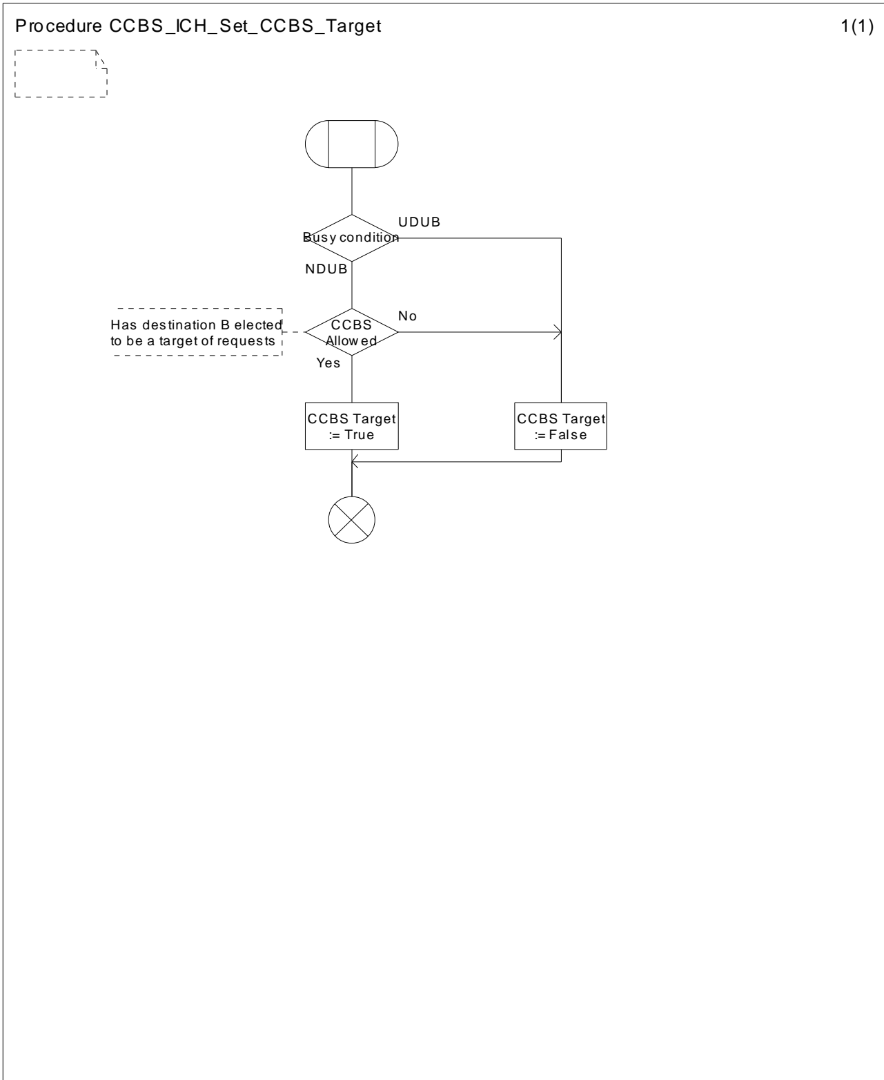
Figure 11.2.3.11: Procedure CCBS_ICH_Set_CCBS_Target
