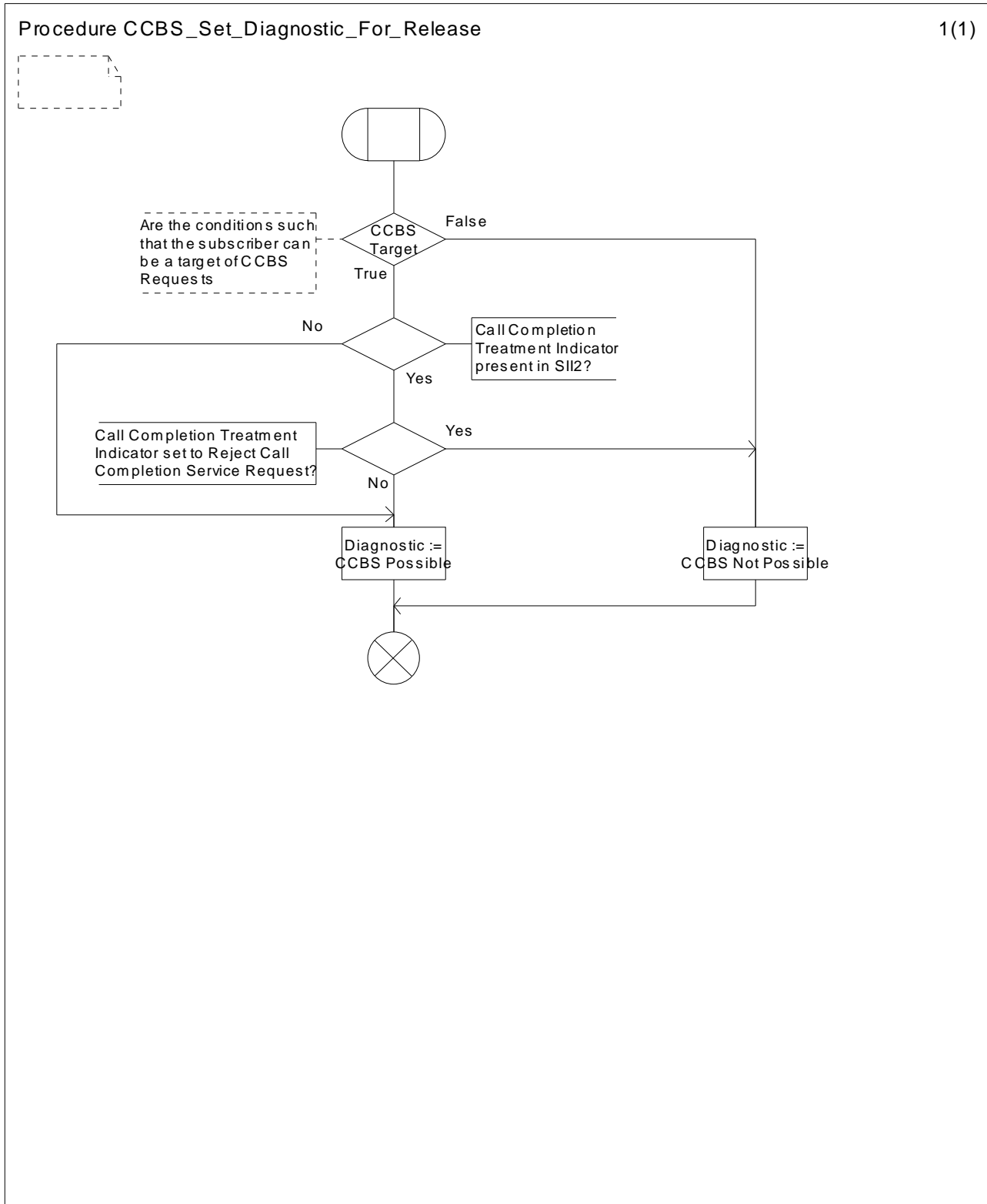
Figure 11.3.4: Procedure CCBS_Set_Diagnostic_For_Release
