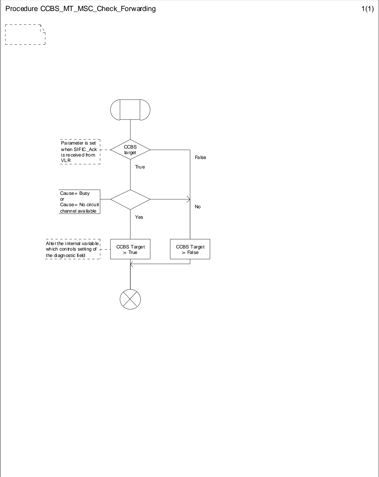
Figure 11.2.3.1: Procedure CCBS_MT_MSC_Check_Forwarding
